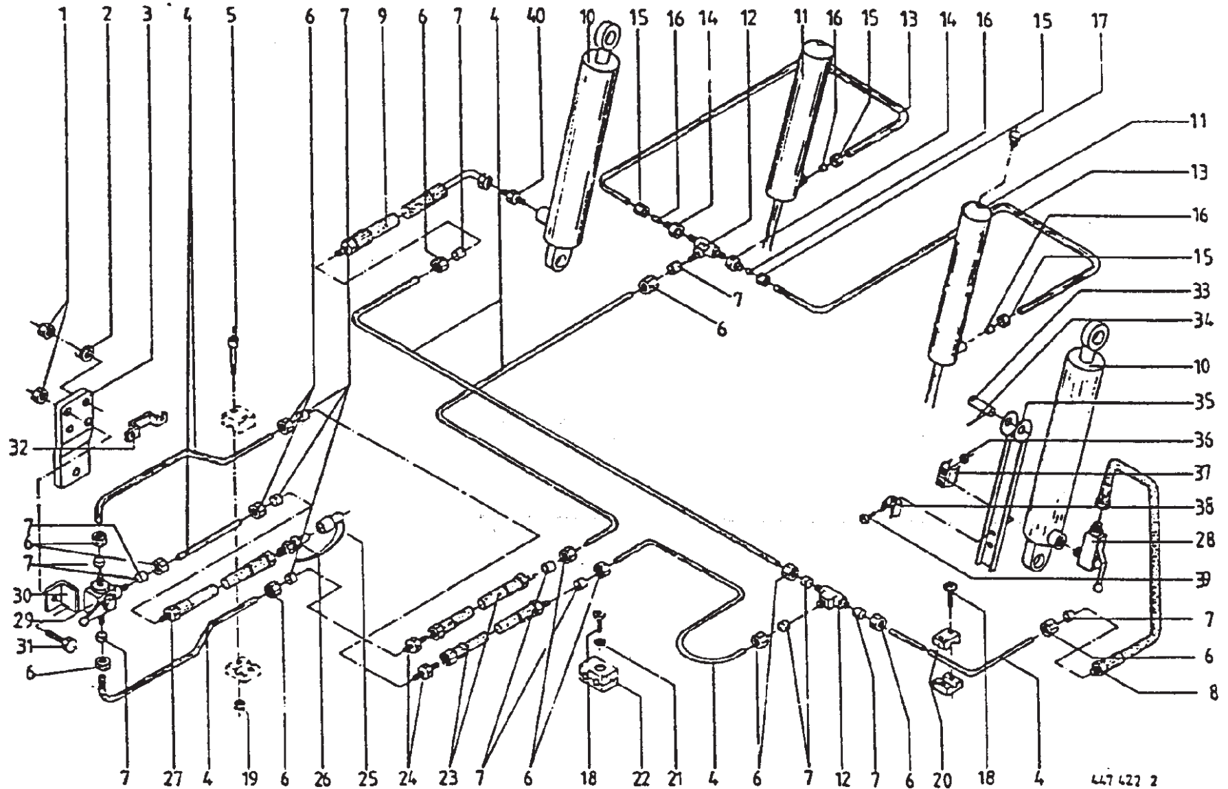
Hydraulics - Wide Pickup
