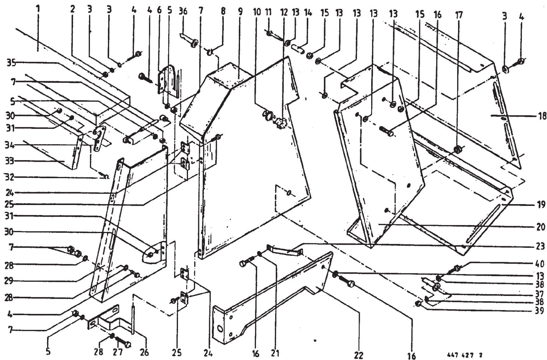
Front & Rear Guards - KR-160 - Wide Pickup
