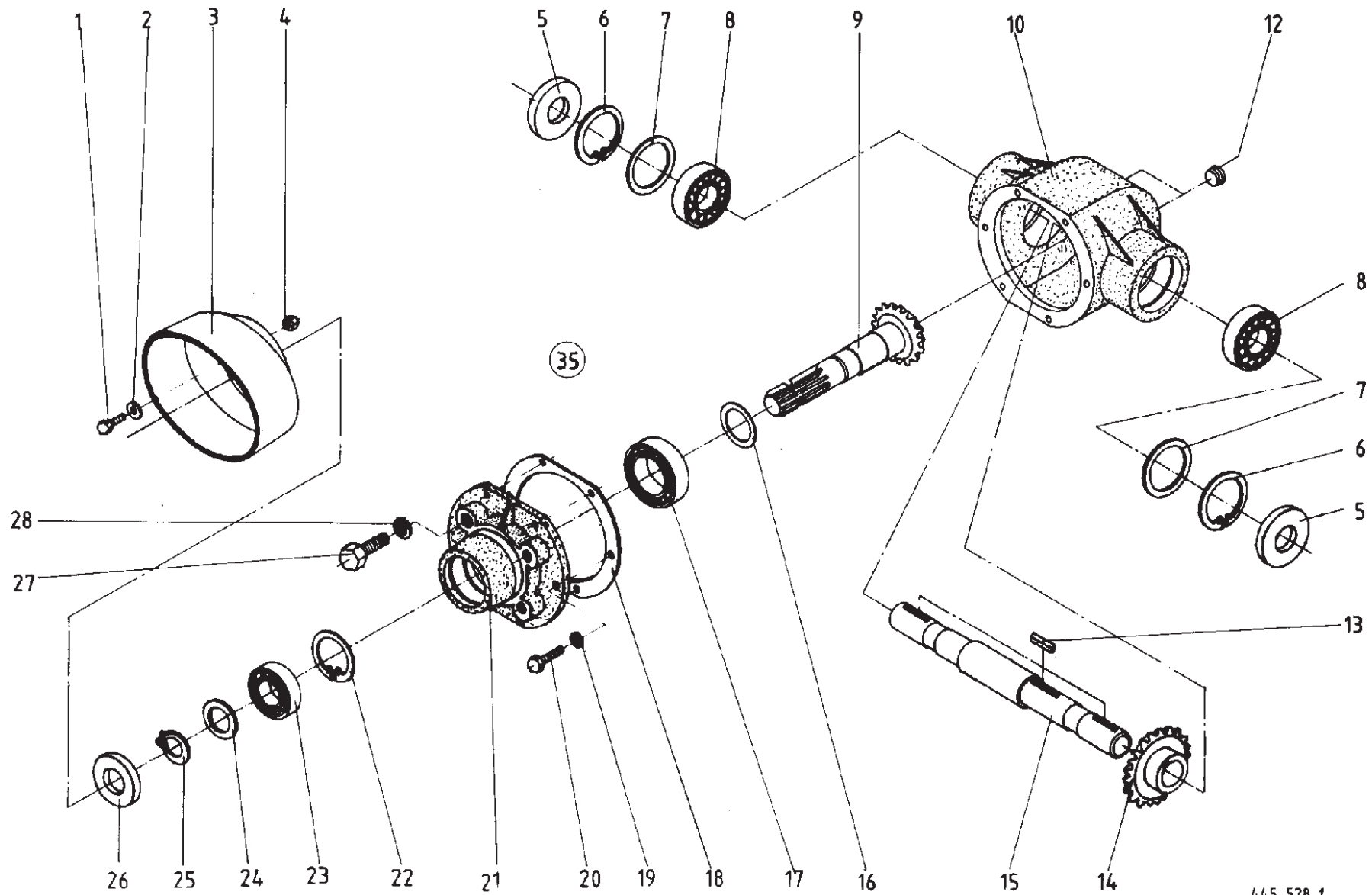
Gearbox (with Dog Clutch)
