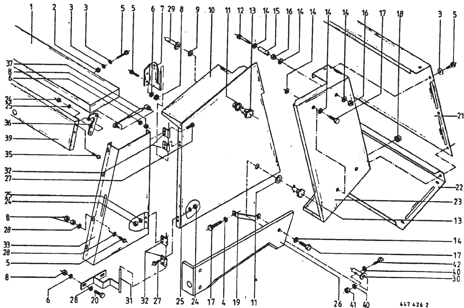
Front & Rear Guards - KR-130 - Wide Pickup
