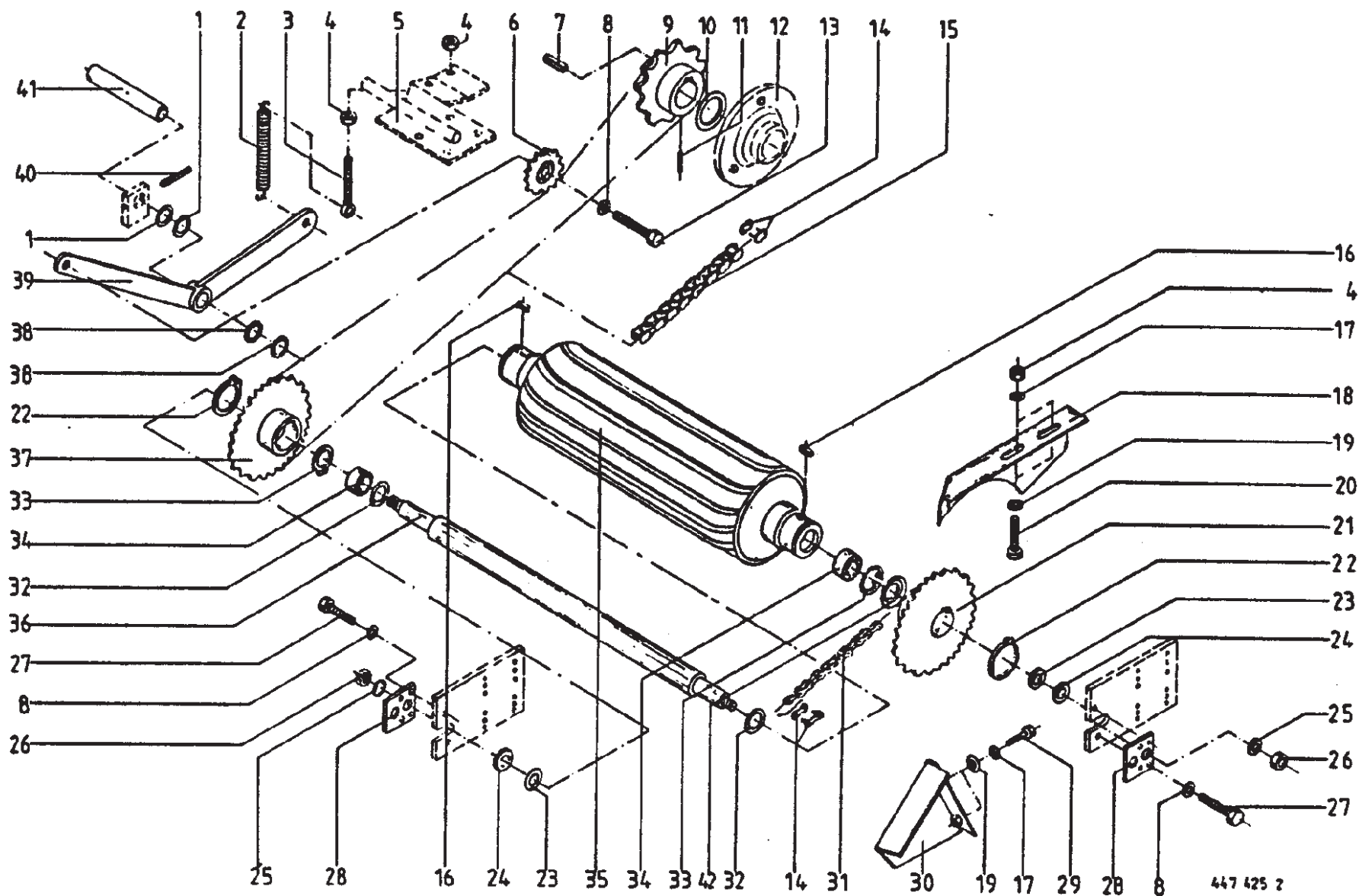
Lower Roller - Wide Pickup
