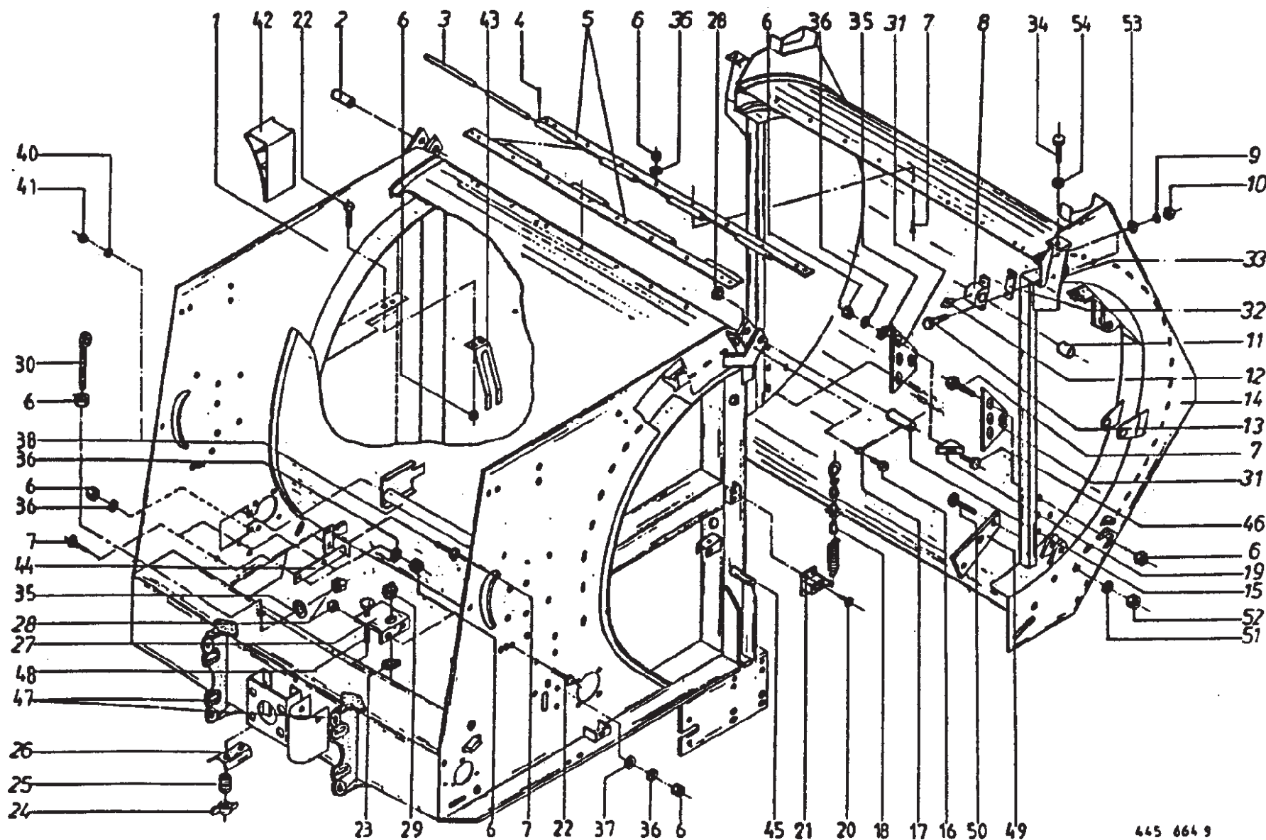
Main Frame - Standard Pickup
