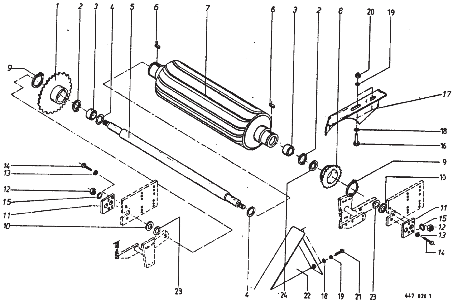
Lower Roller - Standard Pickup
