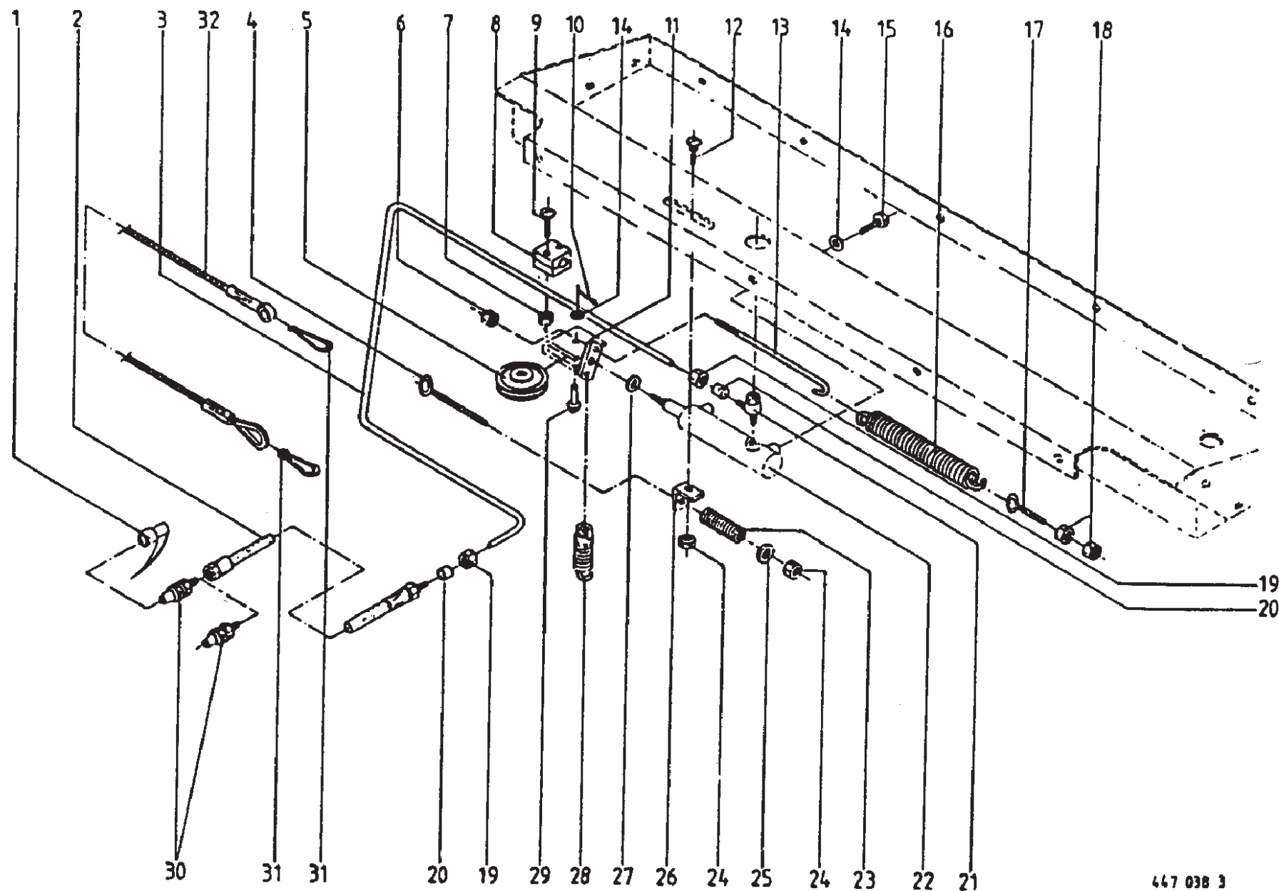
Hydraulic Starter
