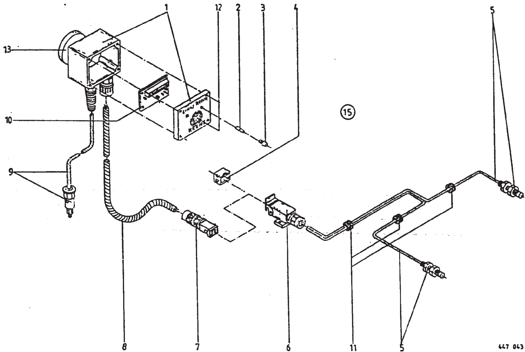
Bale Monitor
