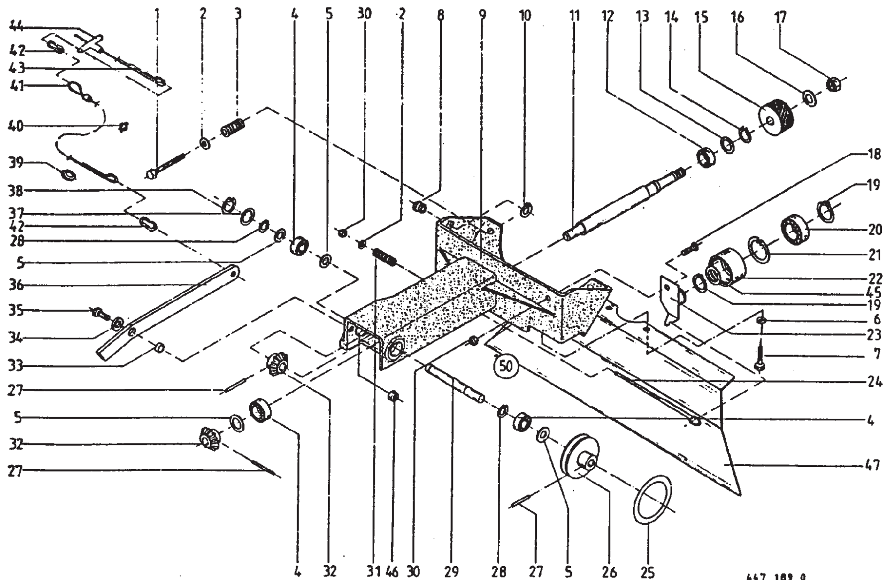
Single Twine Manual Starter
