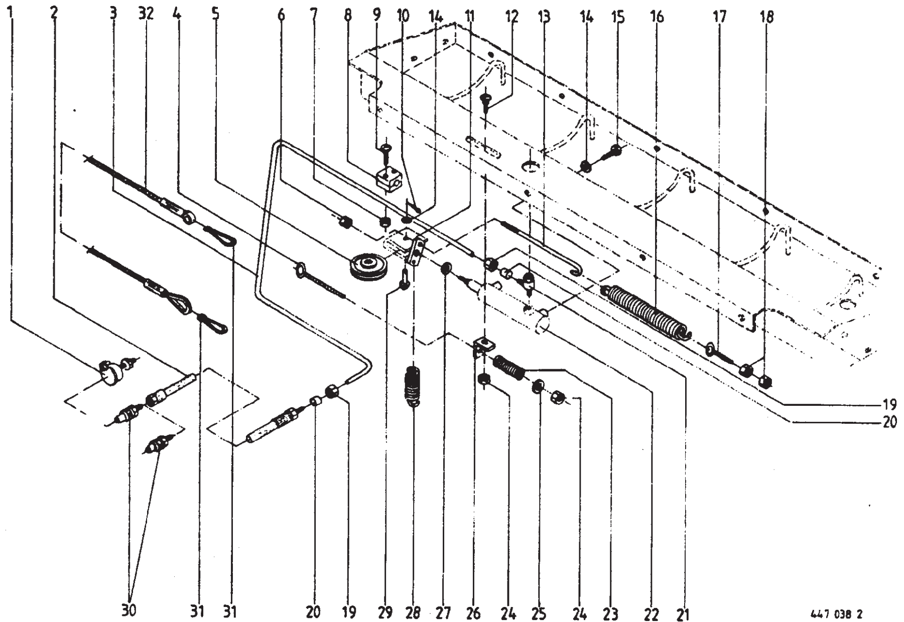
Hydraulic Starter
