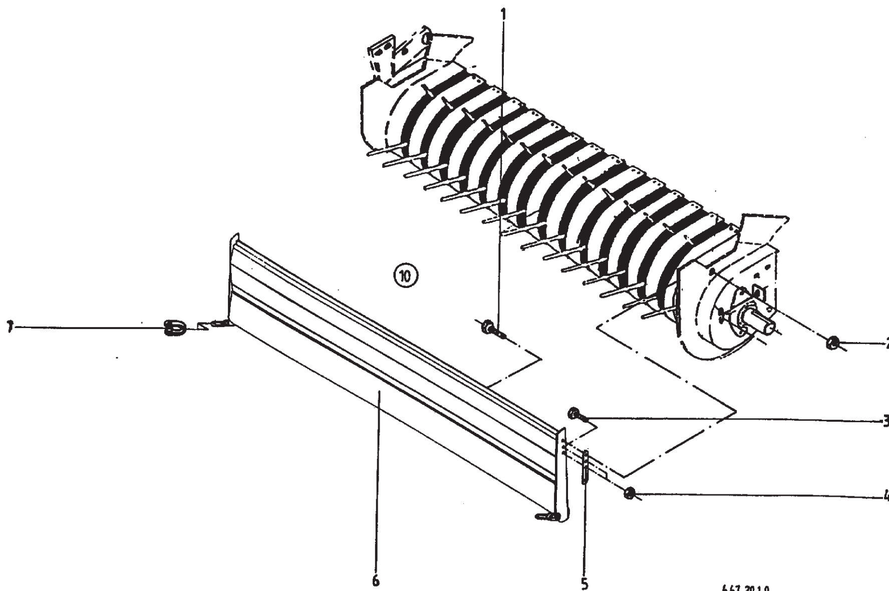
Pickup Baffle Plate
