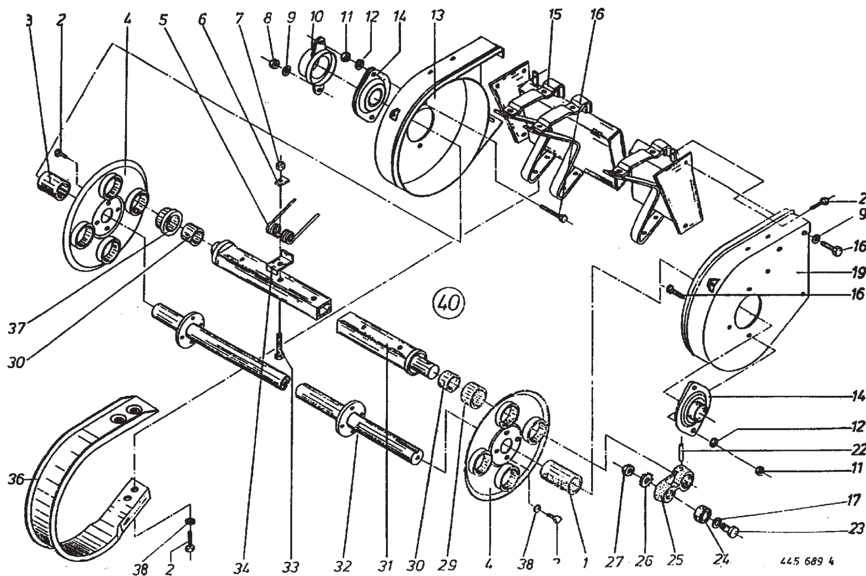
Pickup Drum
