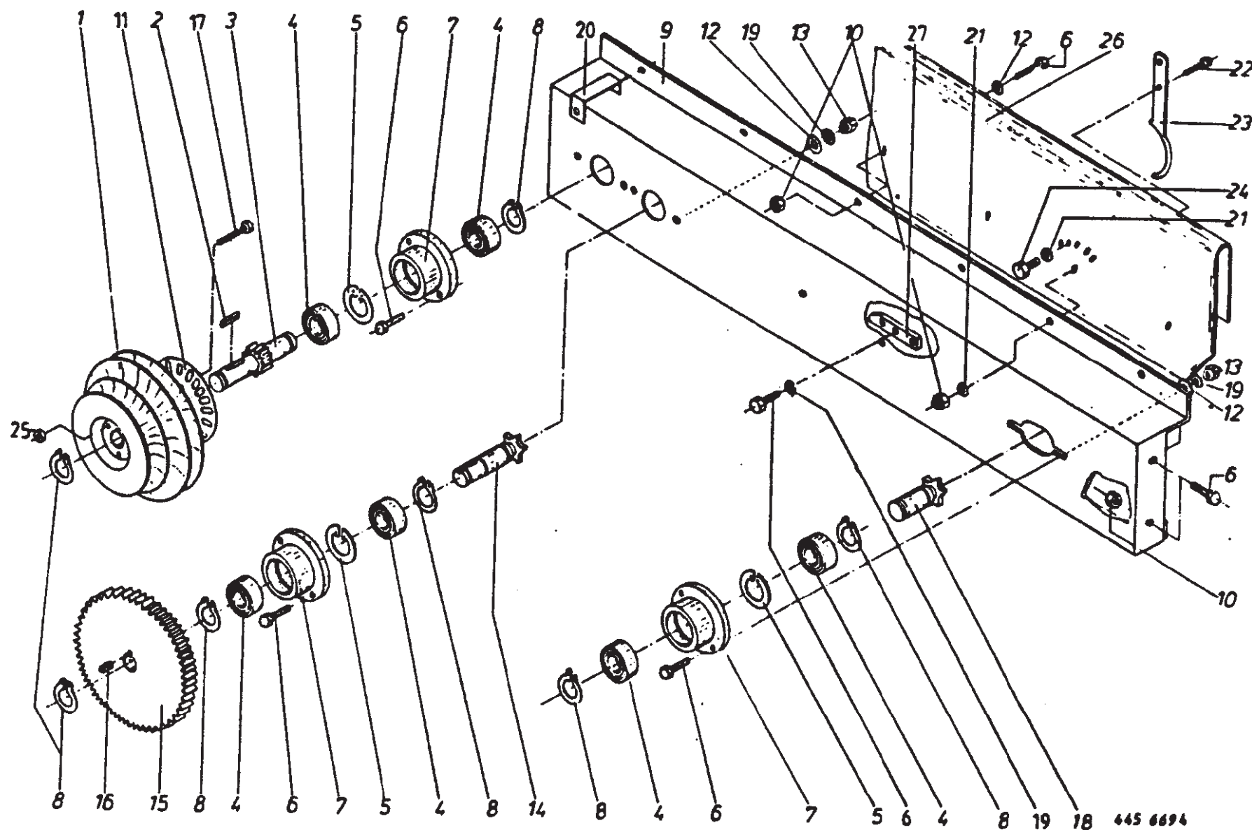
Single Twine Mechanism
