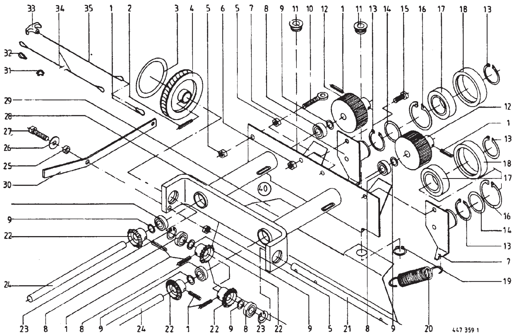
Double Twine Manual Starter
