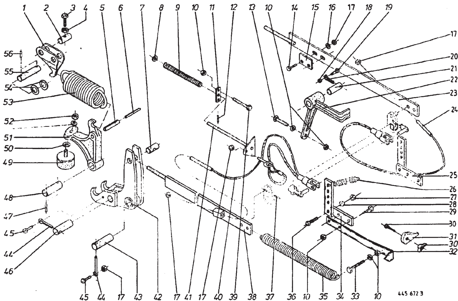
Tailgate Locking Mechanism
