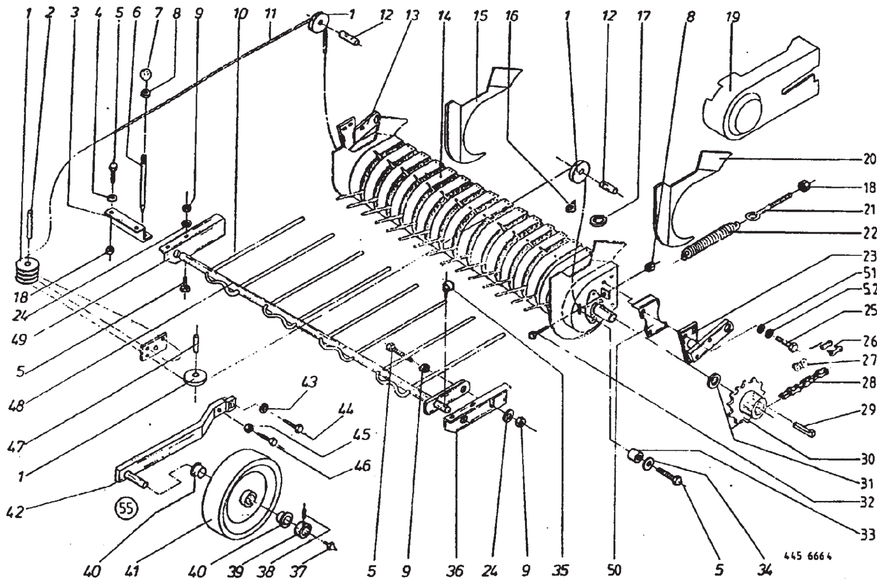
Pickup Drive & Mounting Parts
