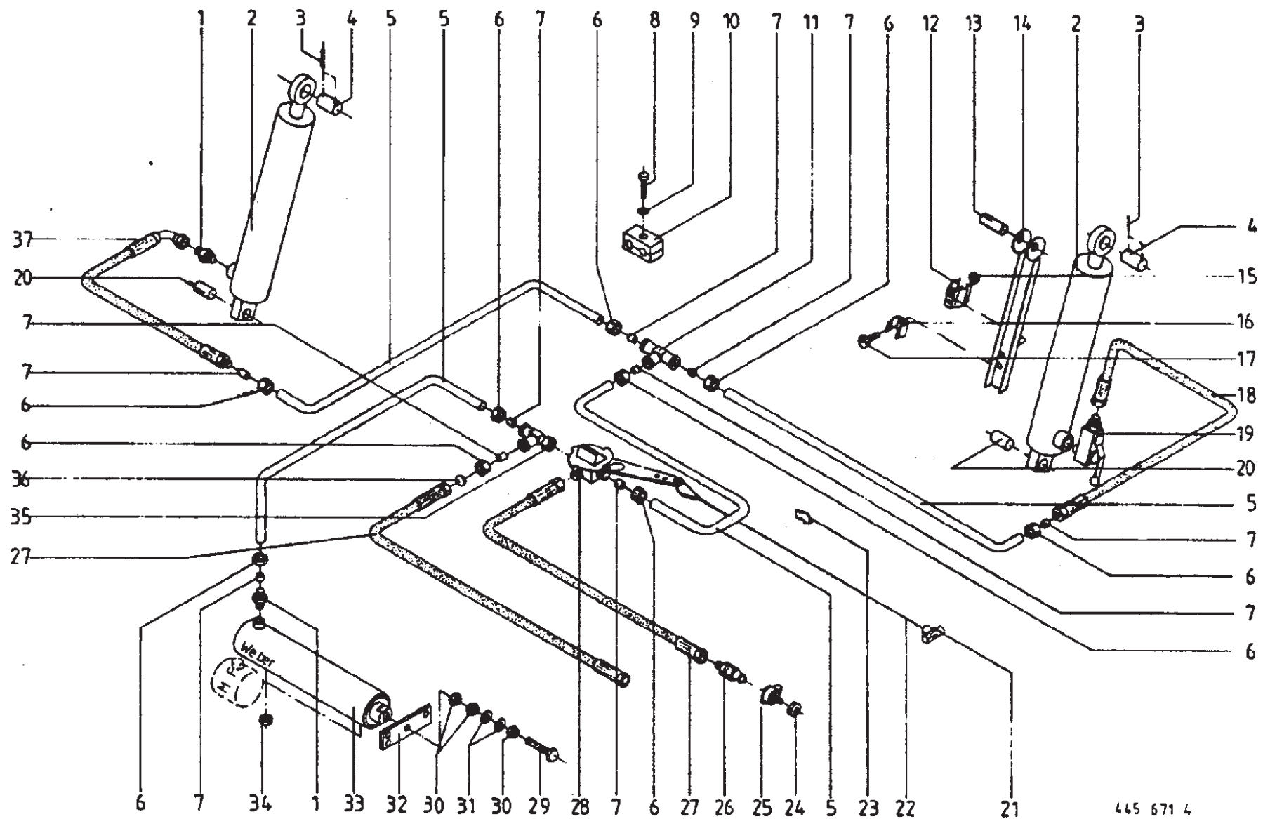
Hydraulic System
