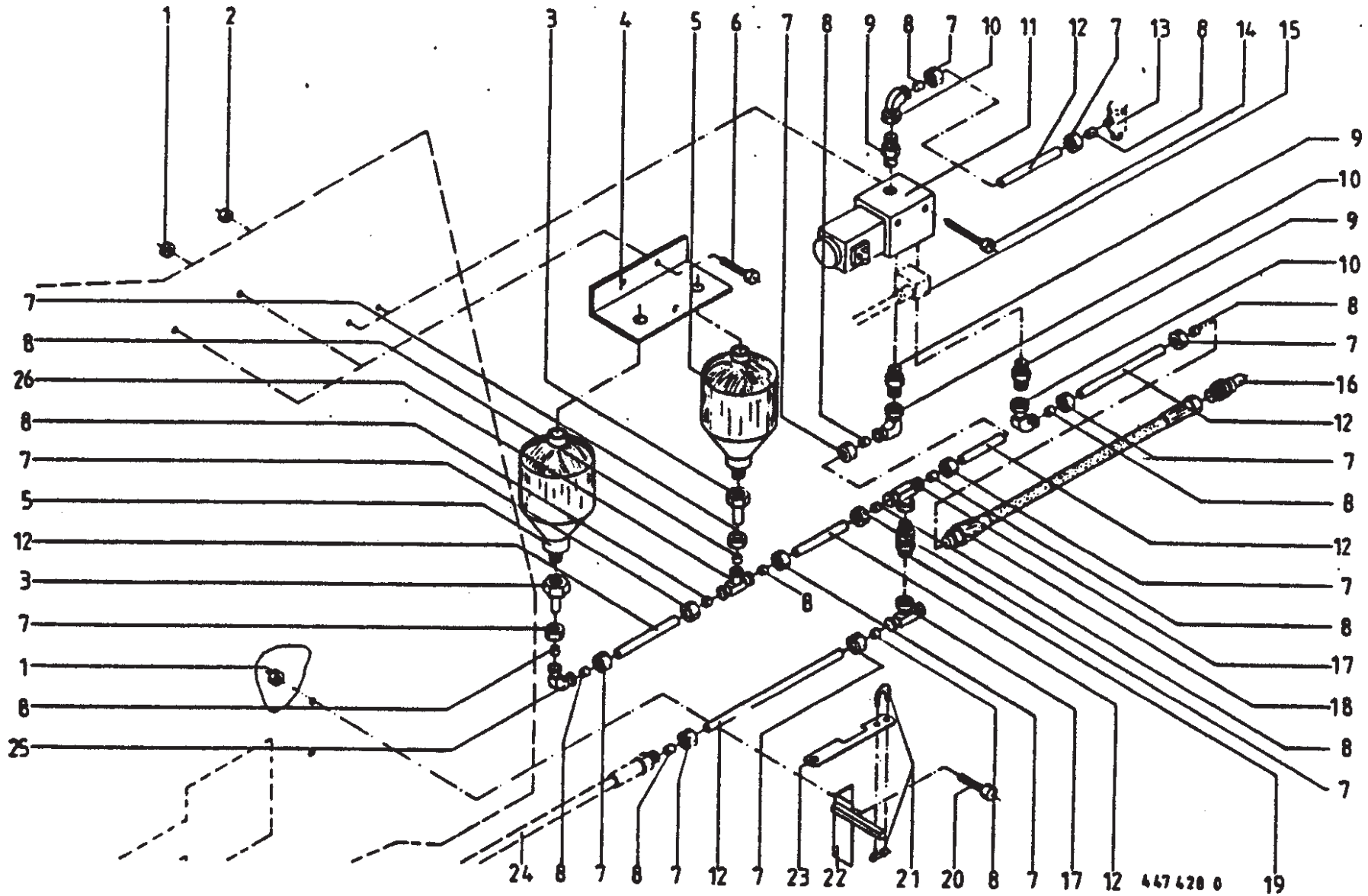
Comfort Control Hydraulics
