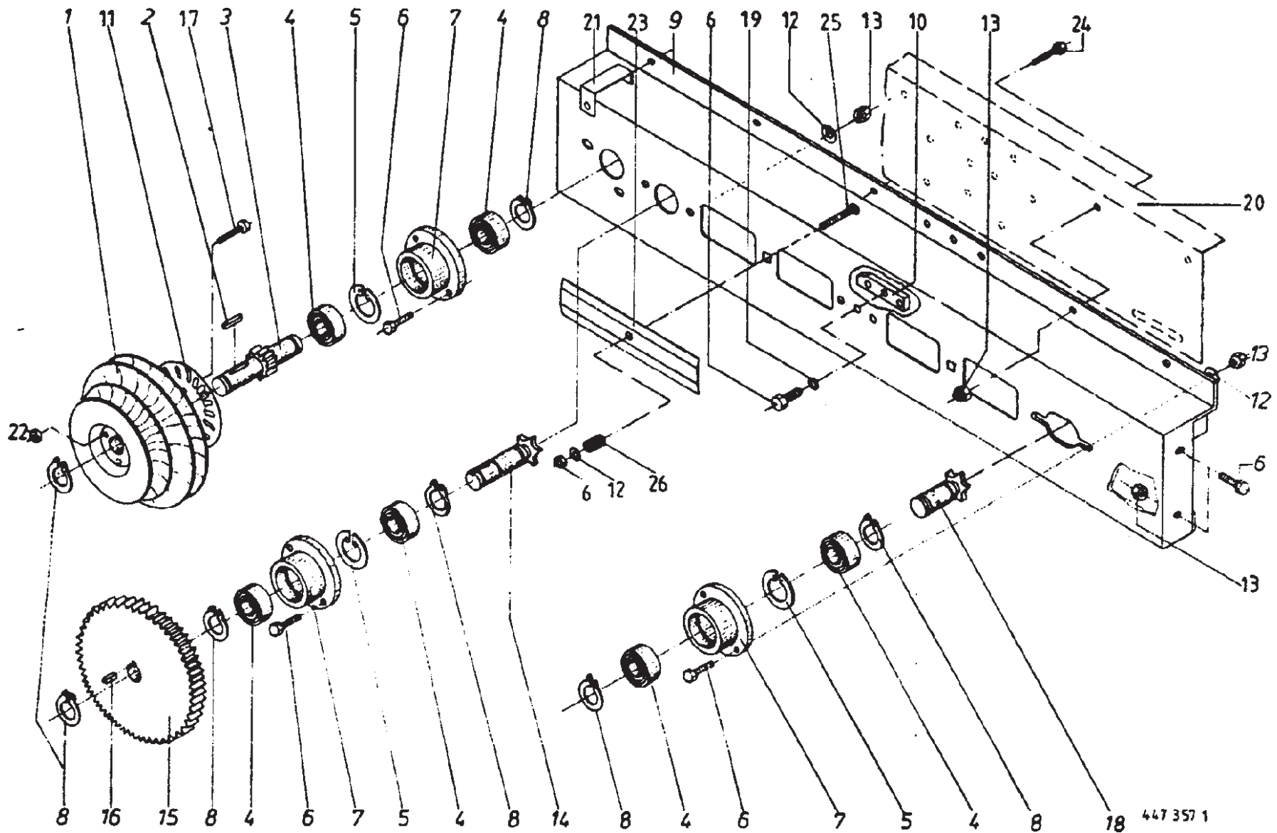
Double Twine Mechanism
