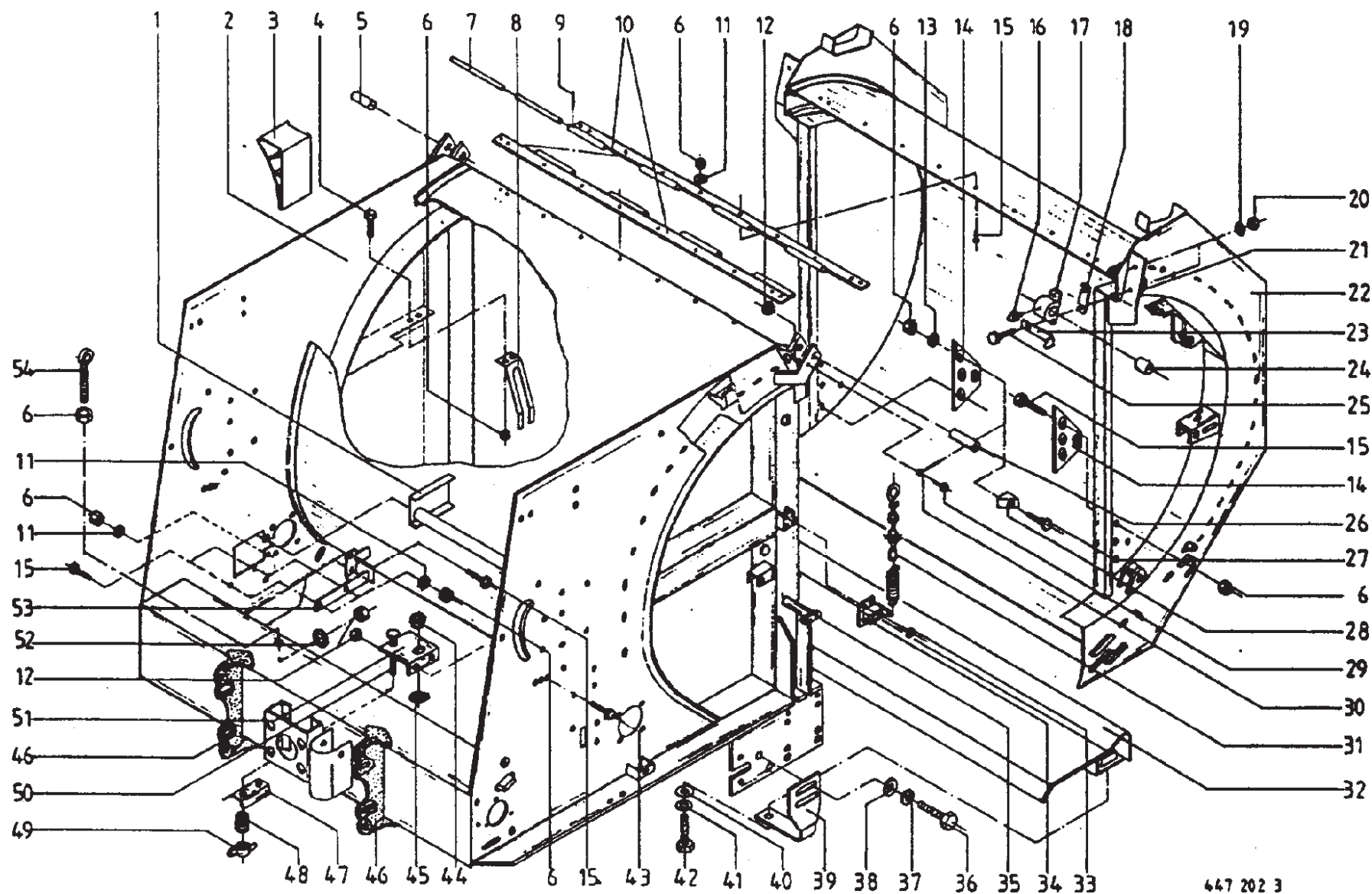
Front & Rear Frame
