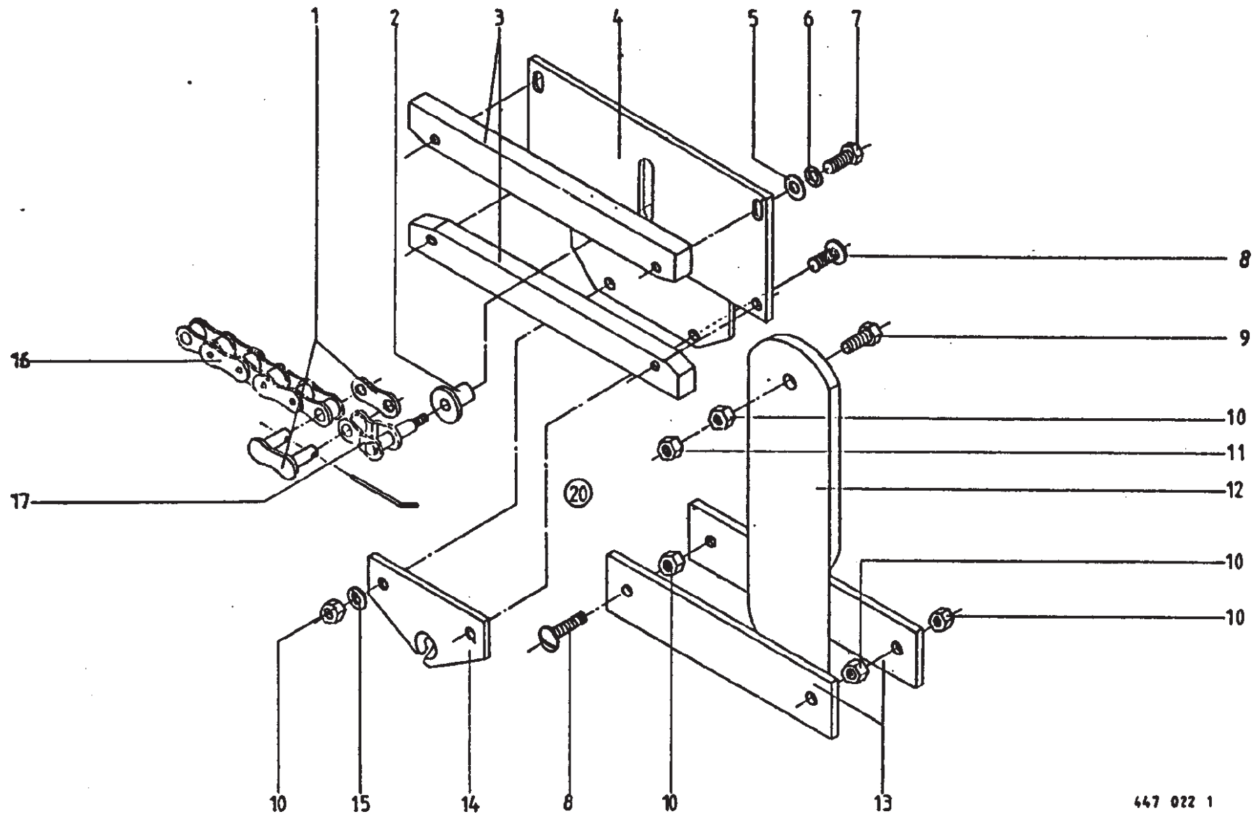
Single Twine Drive & Cutting Unit
