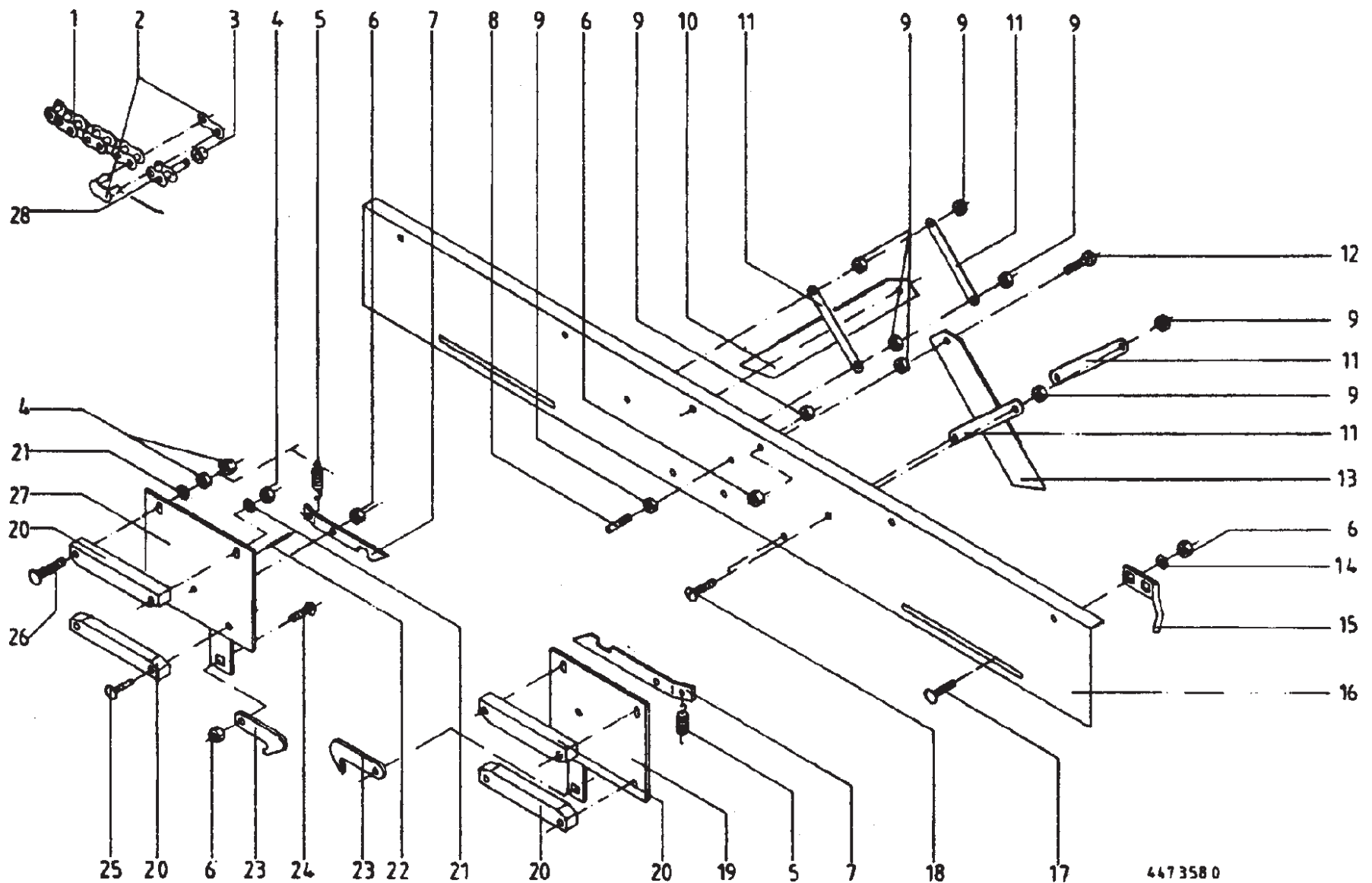
Double Twine Cutting Unit
