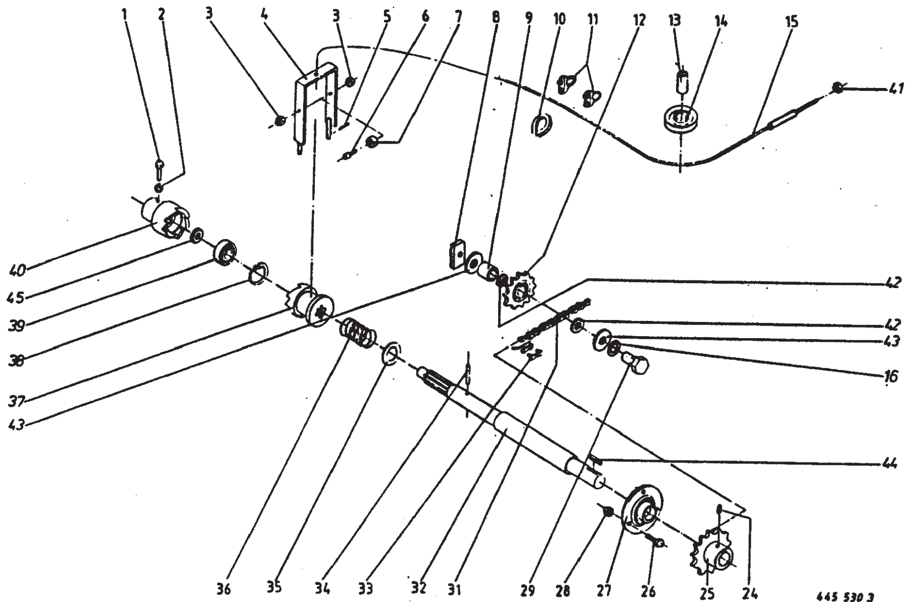
Dog Clutch
