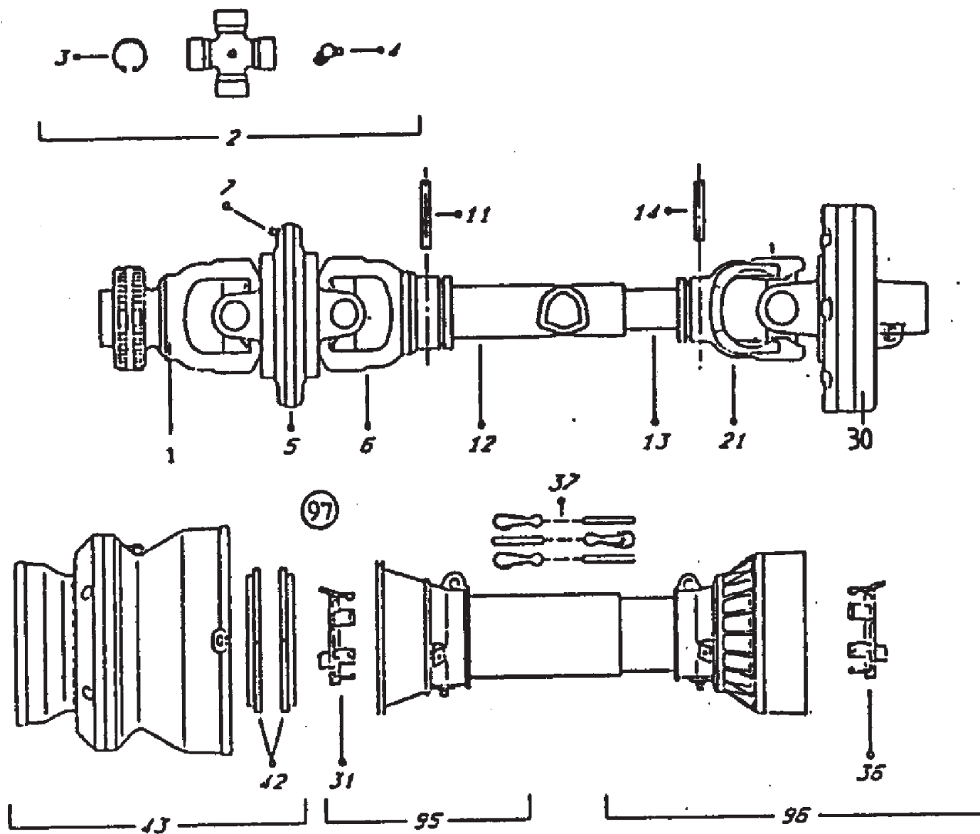
Wide Angle PTO Shaft
