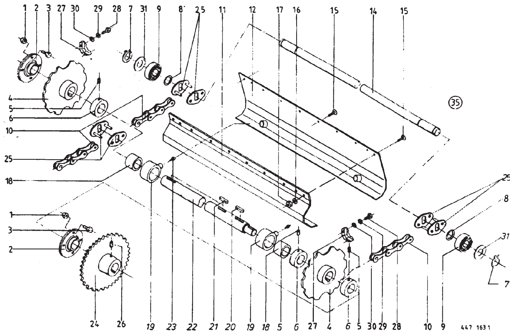
Elevator Chain Drive
