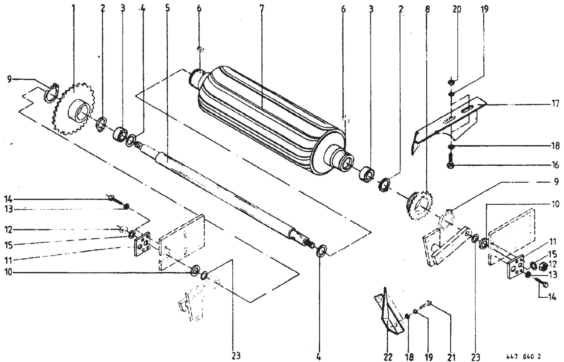
Lower Roller
