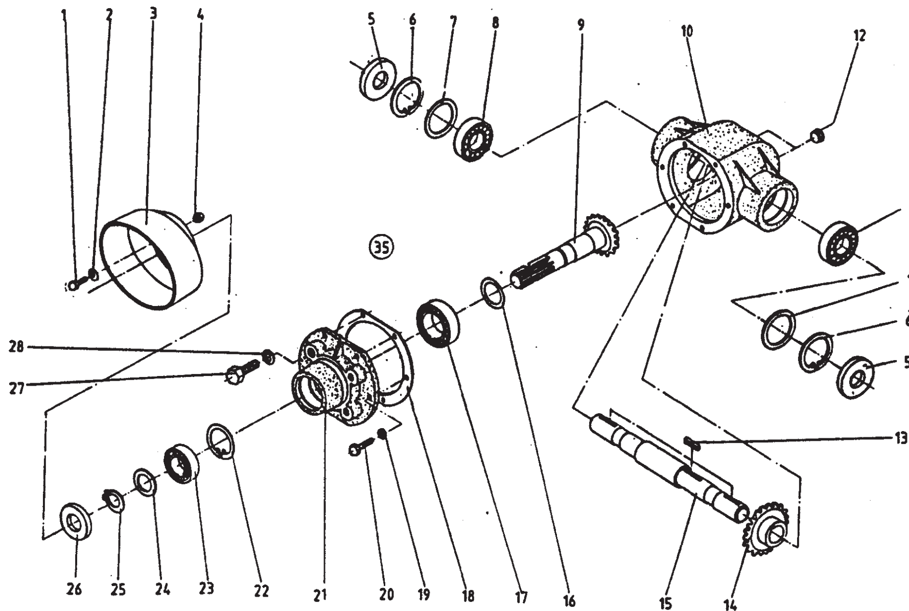
Gearbox
