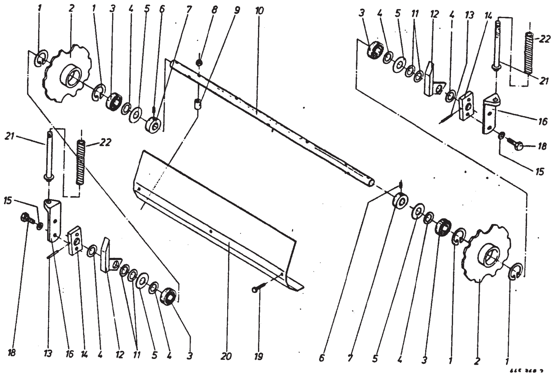
Elevator Chain Tensioner
