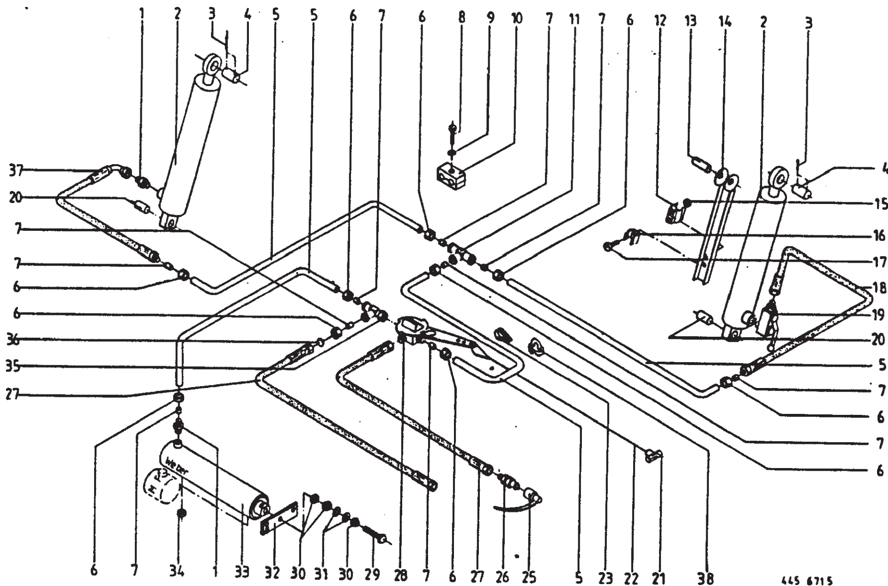
Hydraulic System
