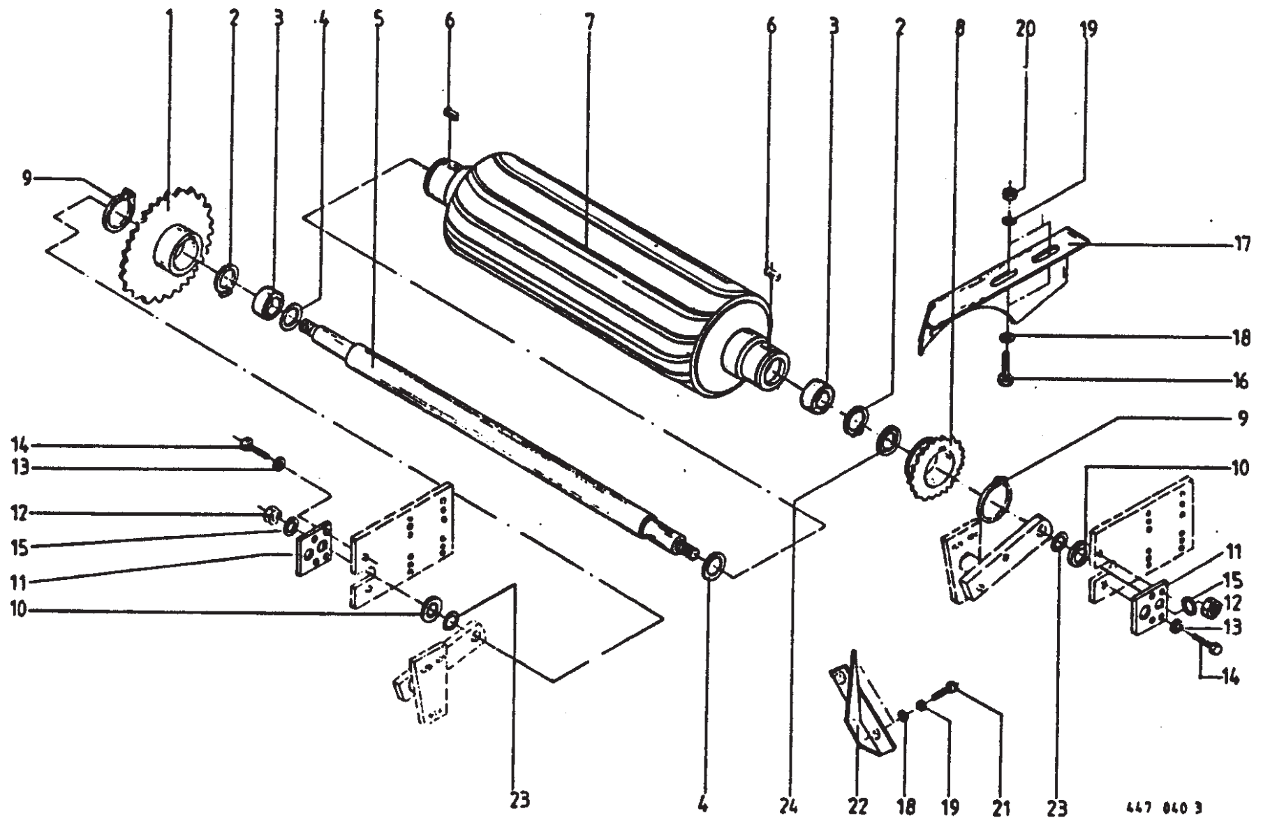
Lower Roller
