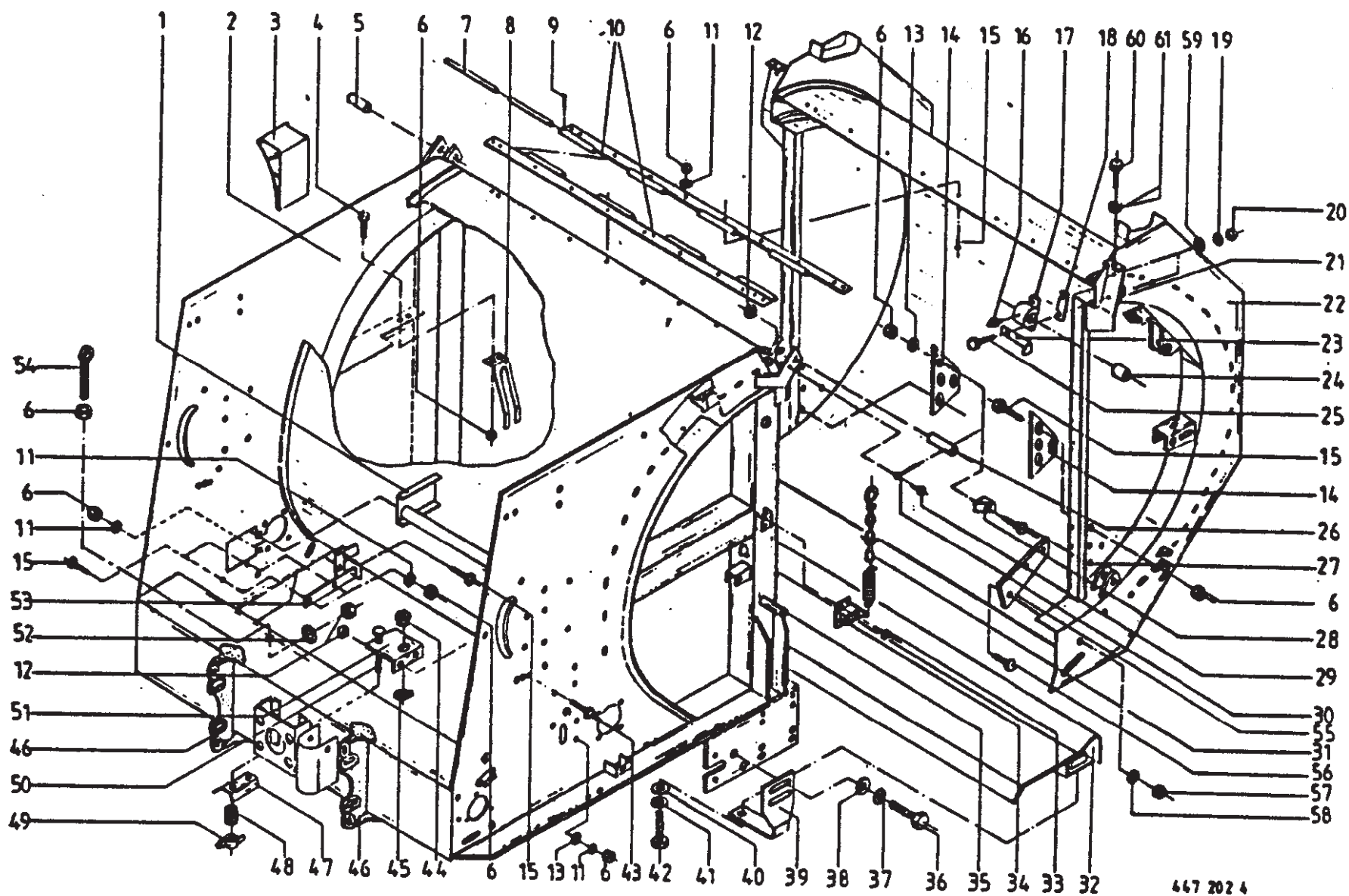
Front & Rear Frame
