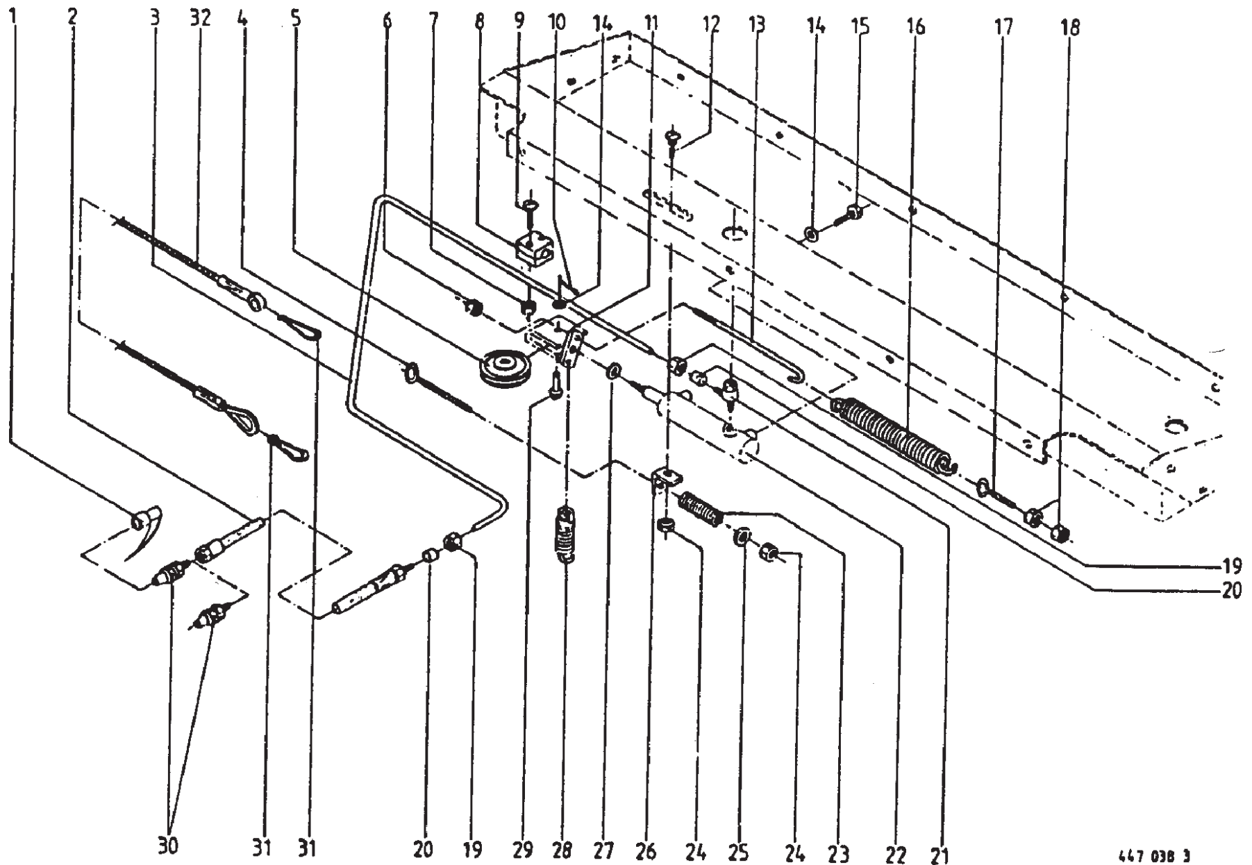
Hydraulic Starter
