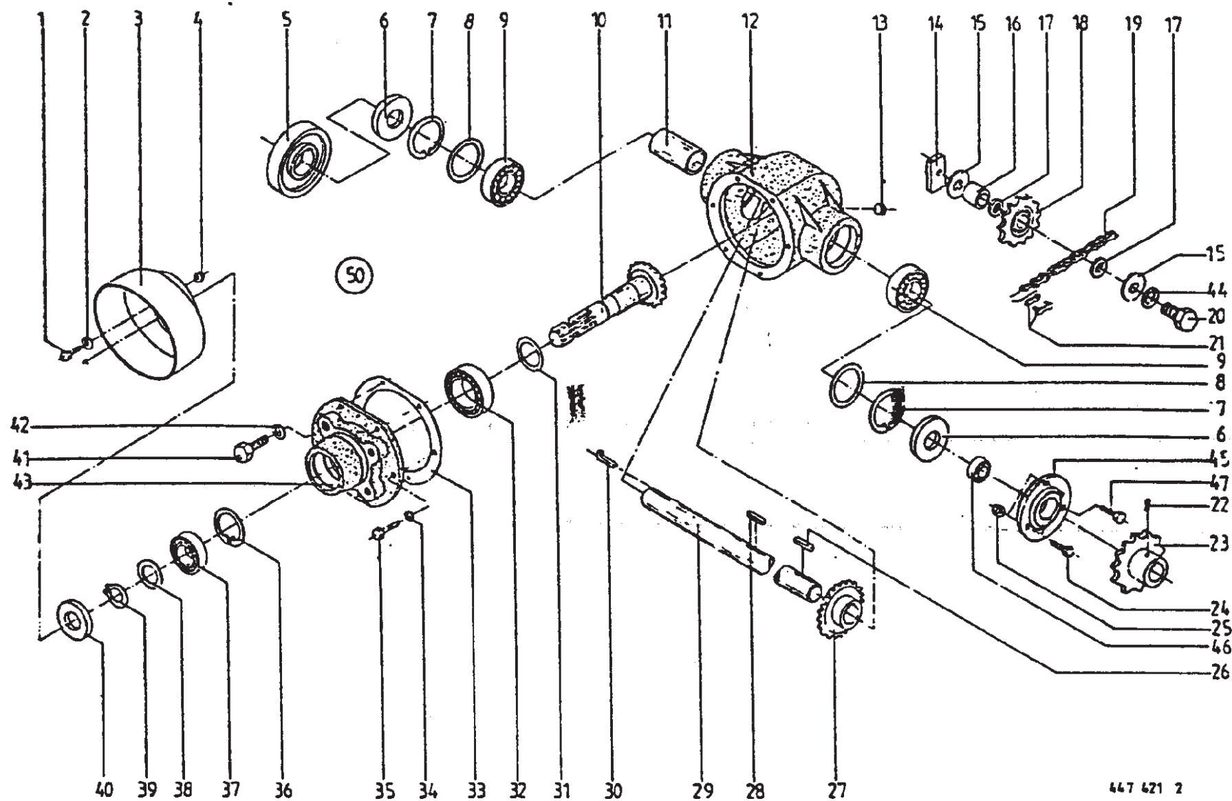
Gearbox
