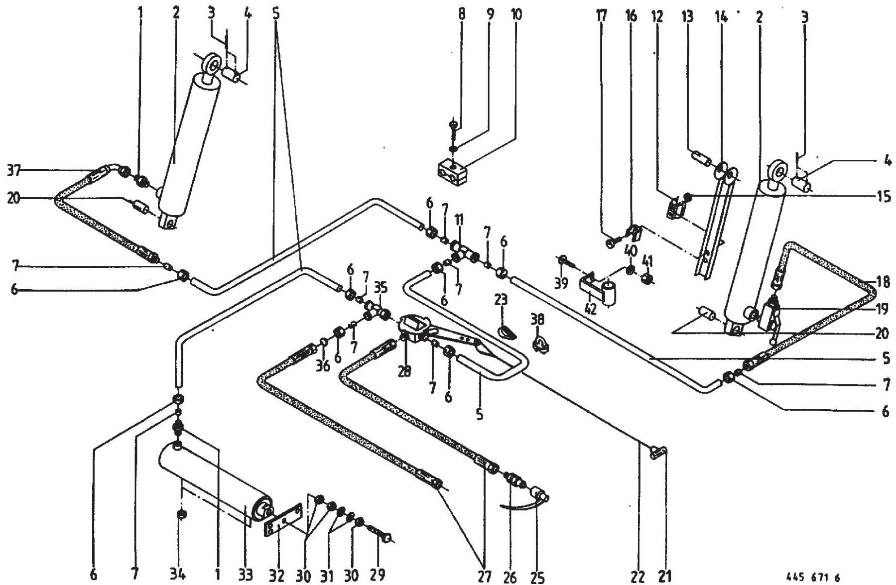
Hydraulic System
