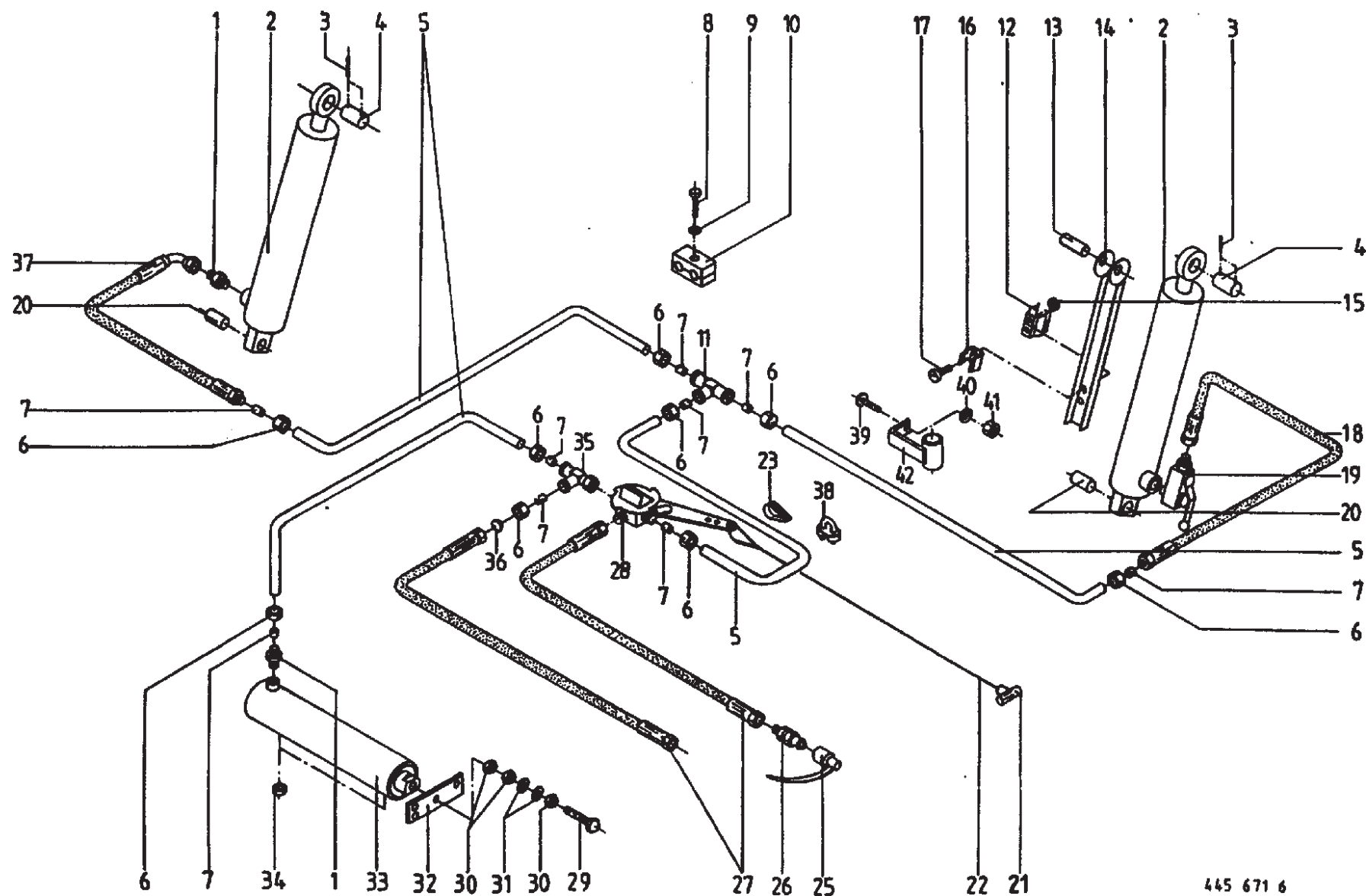
Hydraulic System
