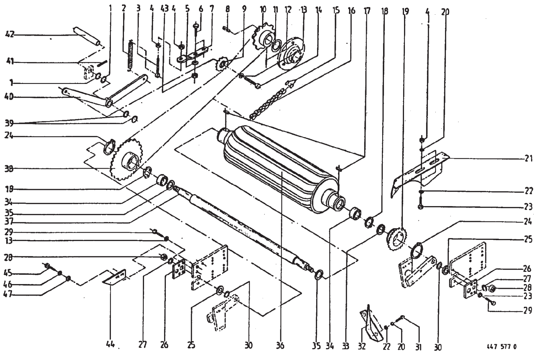
Lower Roller
