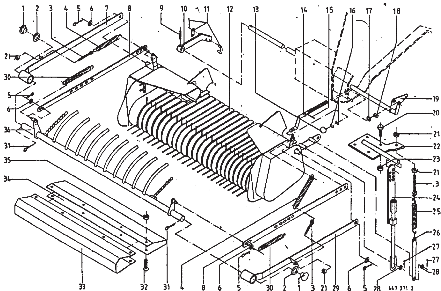
Wide Pickup Baffle Plate & Compressing Rake
