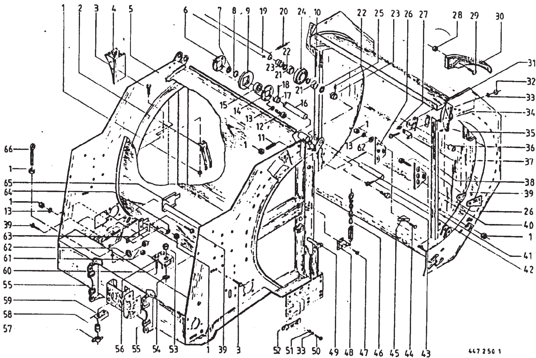
Main Frame - Wide Pickup
