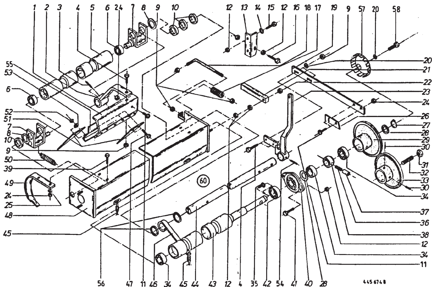
Net Wrap Unit - Standard Pickup
