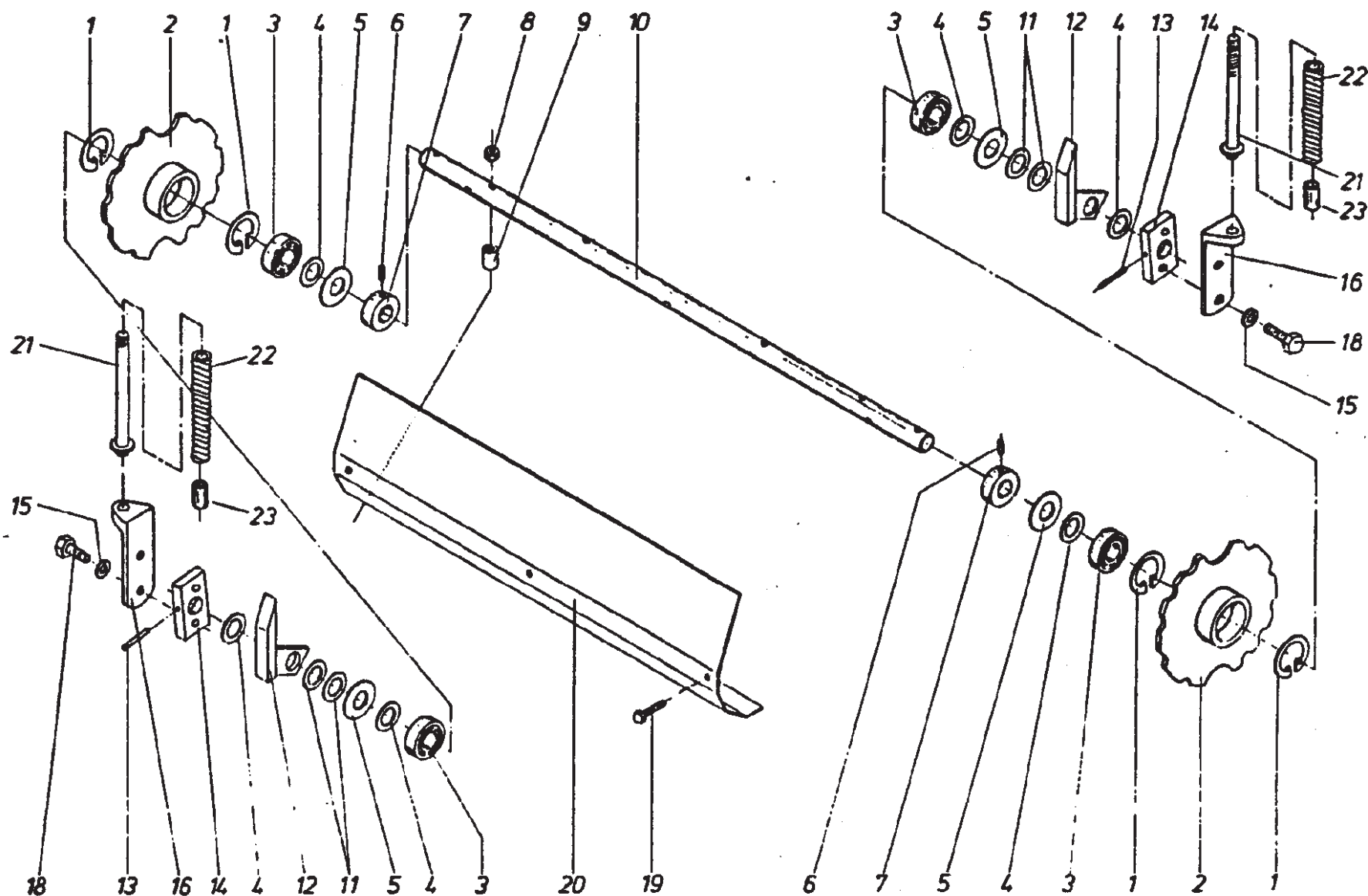
Elevator Chain Tensioner
