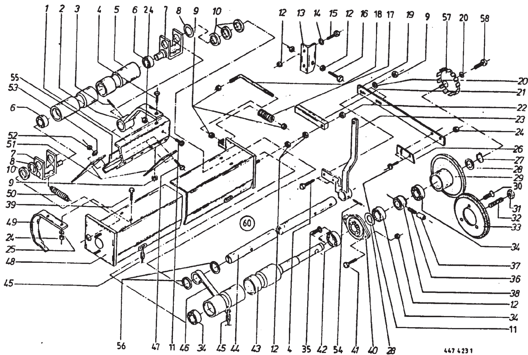
Net Wrap Unit - Wide Pickup
