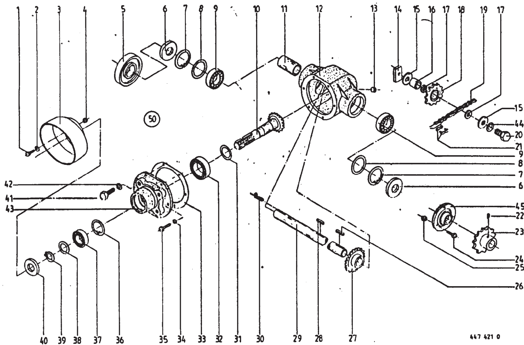
Gearbox (without Dog Clutch)
