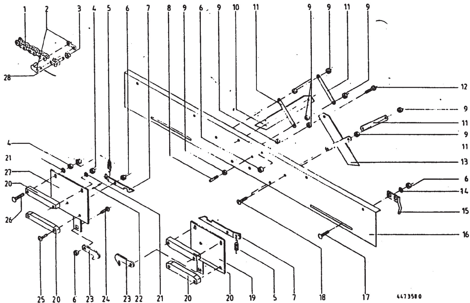
Double Twine Tying Cutting Unit
