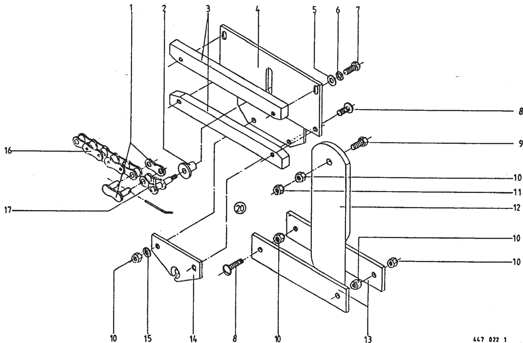
Single Twine Drive & Cutting Mechanism
