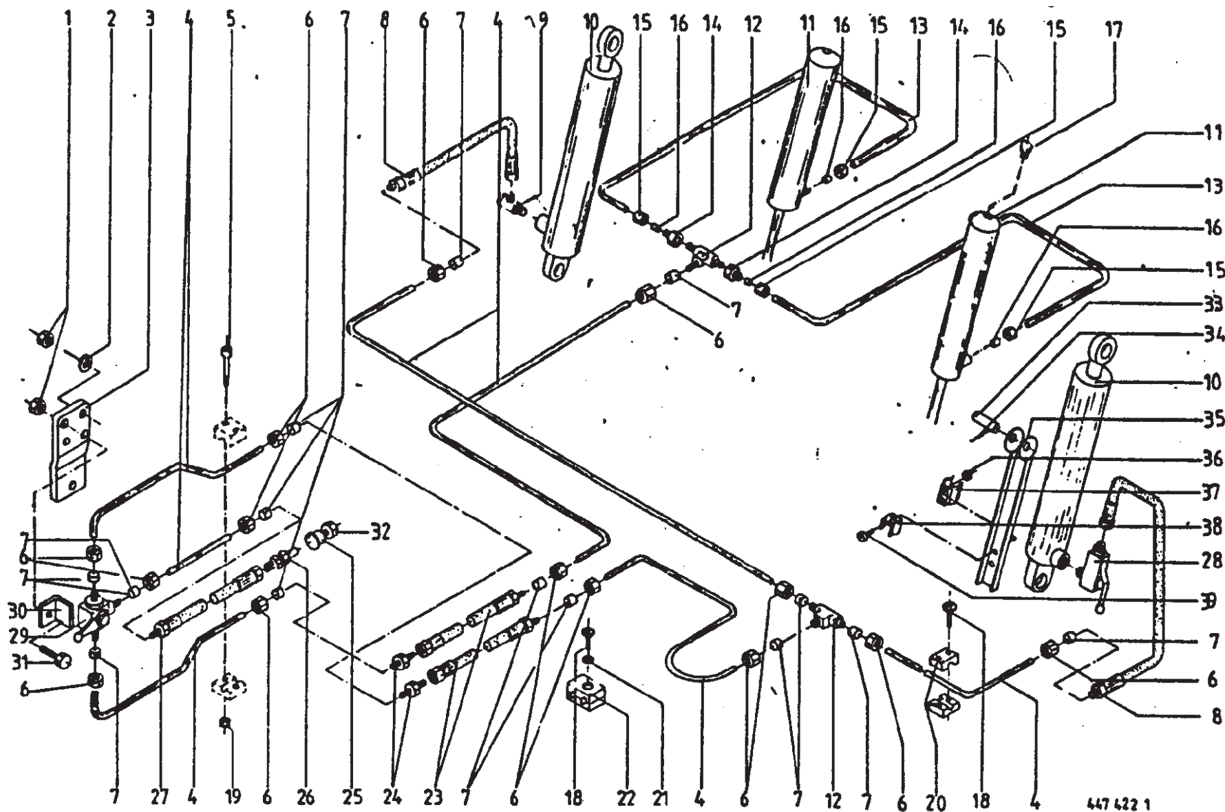
Hydraulics - Wide Pickup
