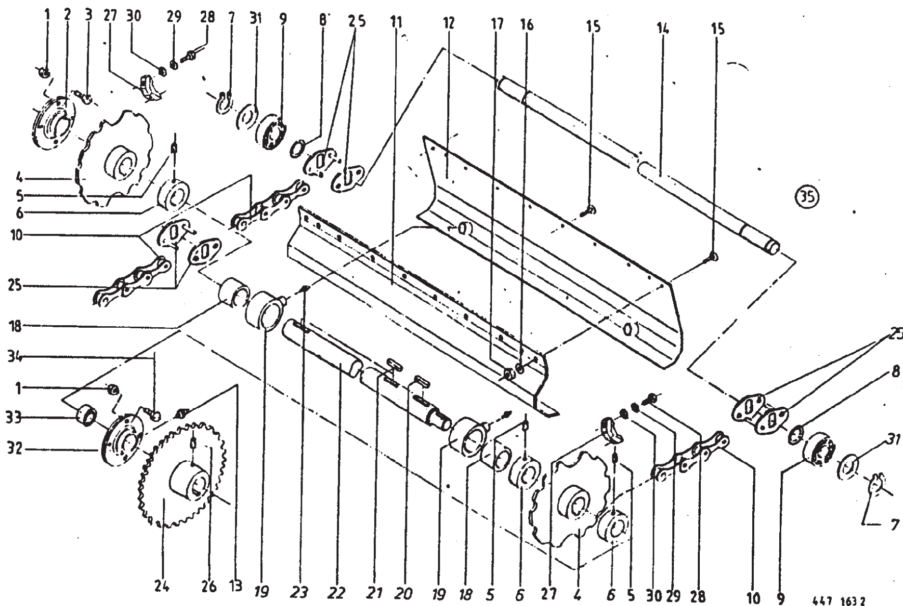
Elevator Chain - Standard Pickup
