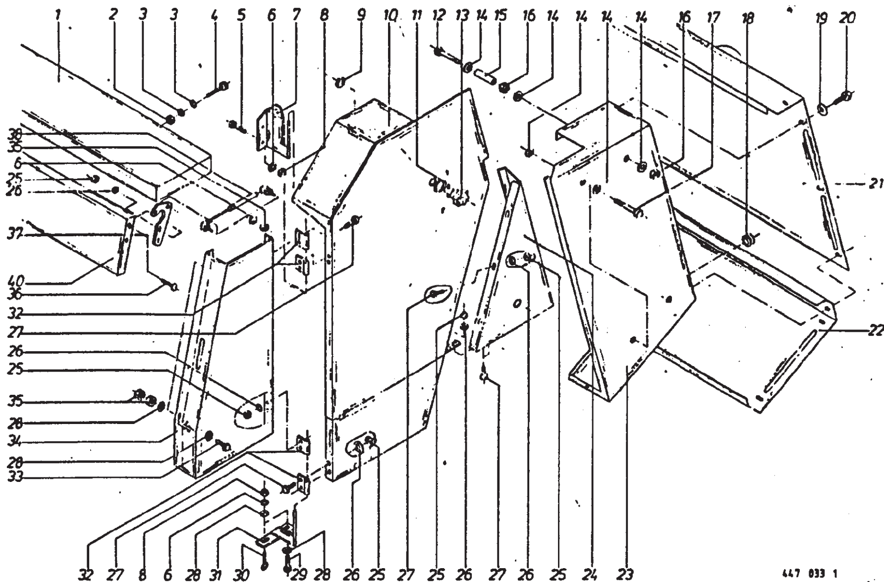
Front & Rear Guards - KR-160 - Standard Pickup
