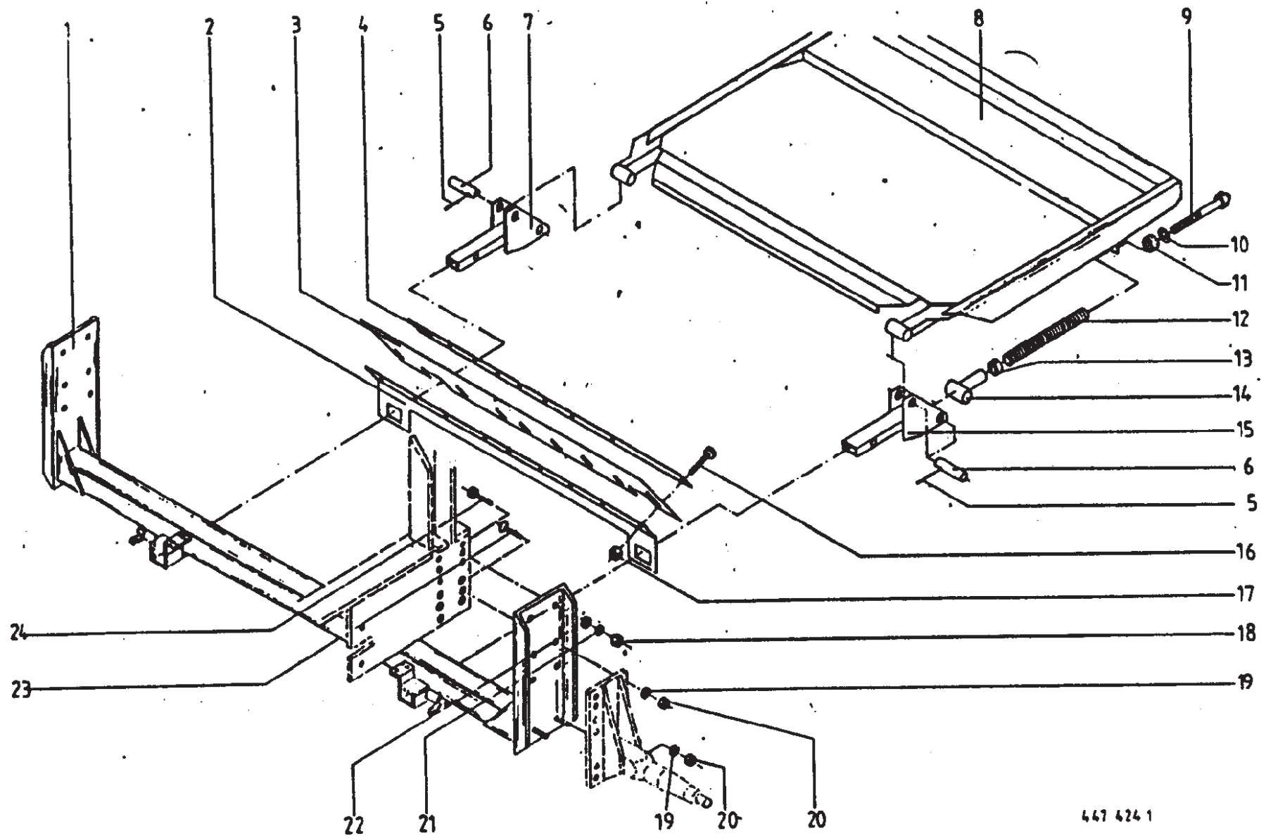
Axle Beam & Bale Ramp - Wide Pickup
