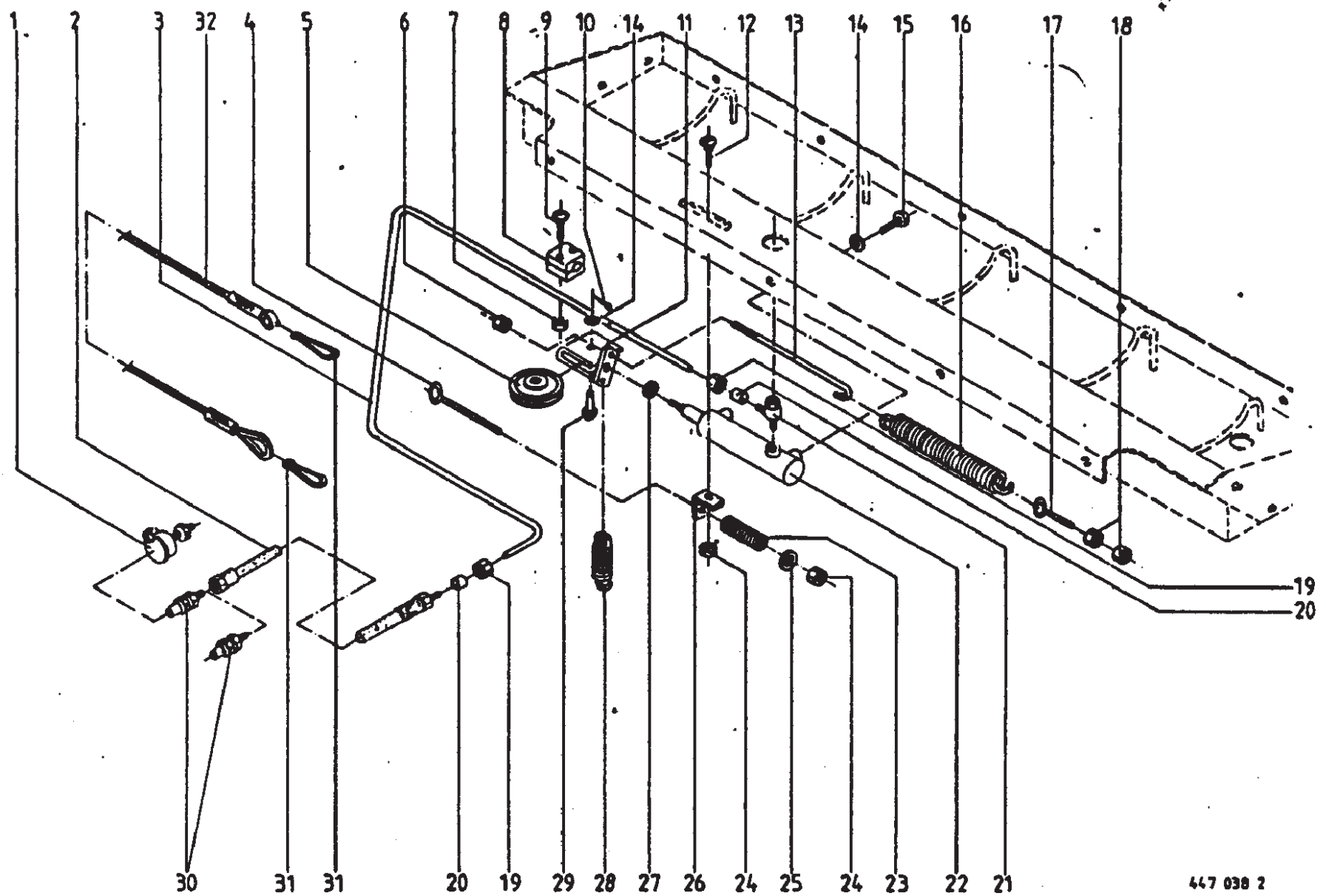
Hydraulic Starter
