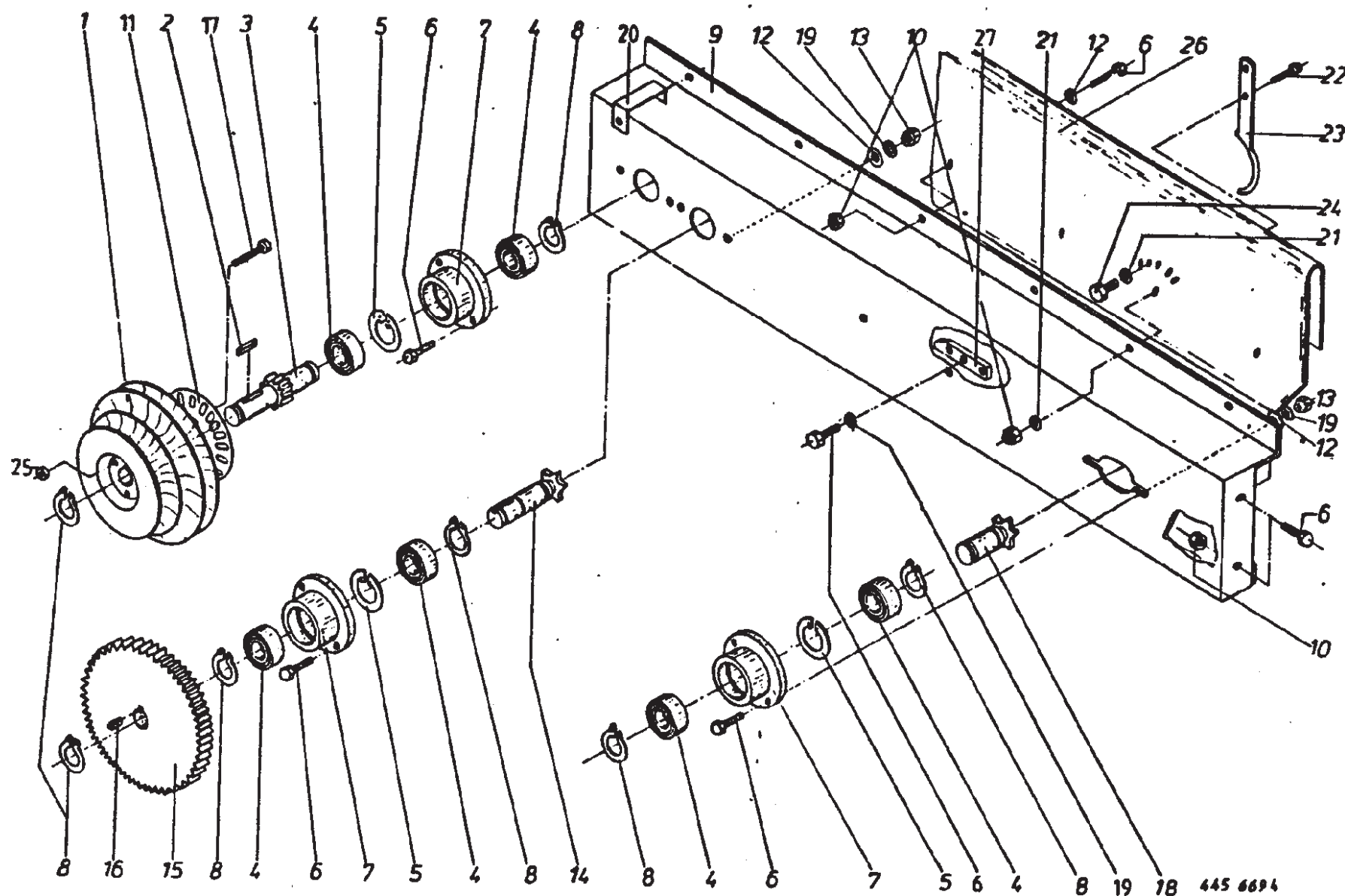
Single Twine Tying Mechanism
