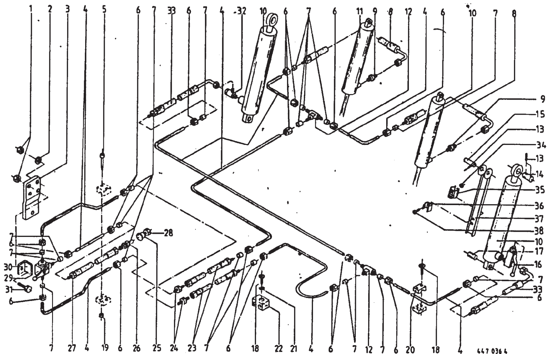
Hydraulics - Standard Pickup
