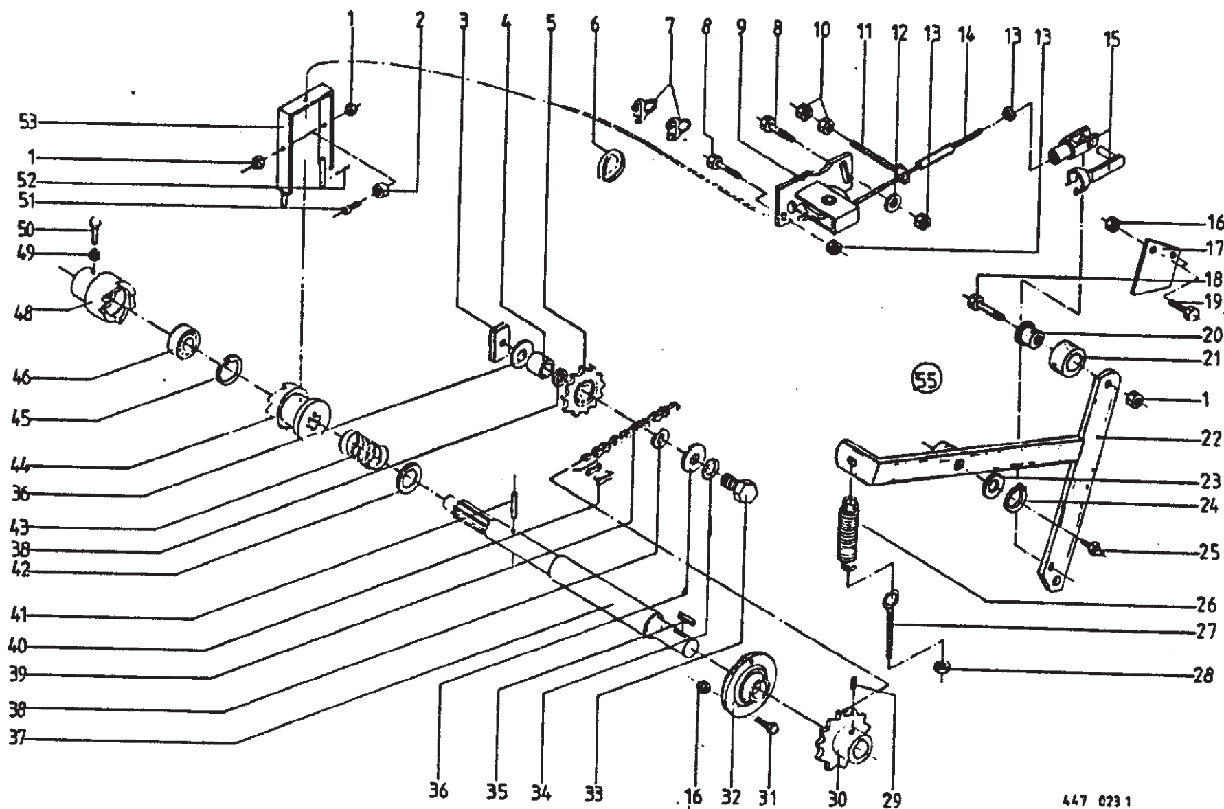
Dog Clutch
