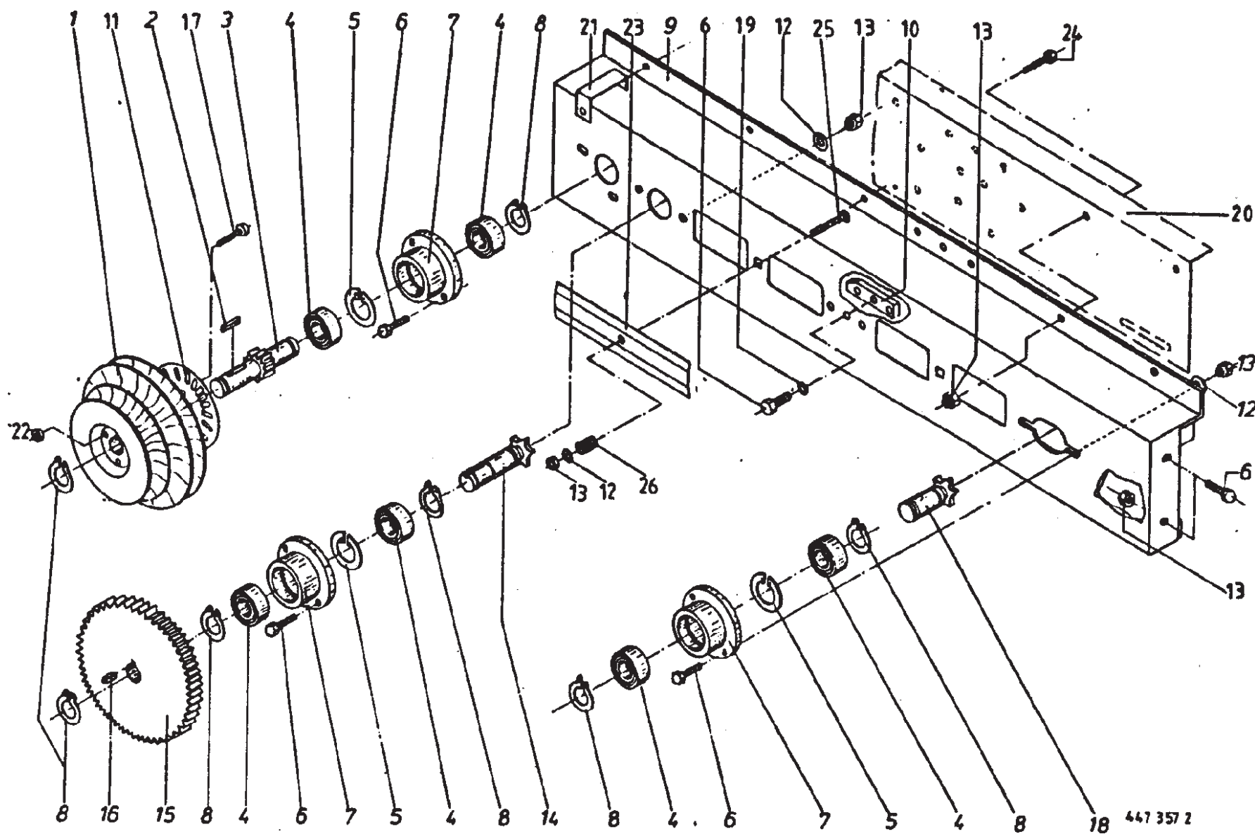
Double Twine Tying Mechanism
