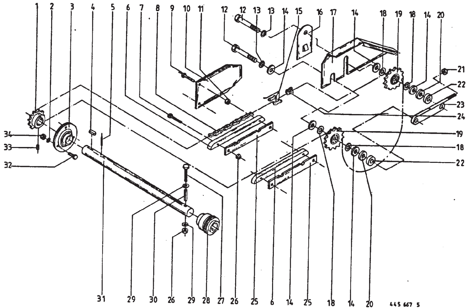
Roller Drive (with Dog Clutch)
