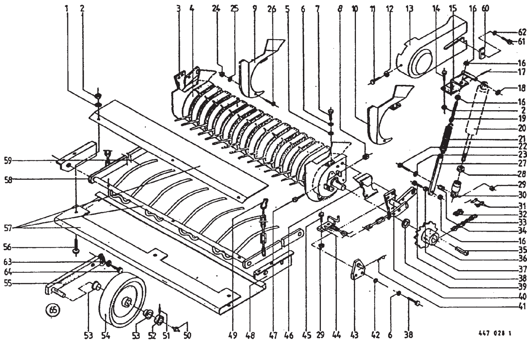
Pickup Mounting
