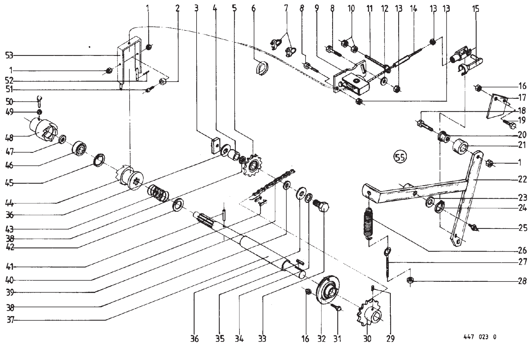
Dog Clutch
