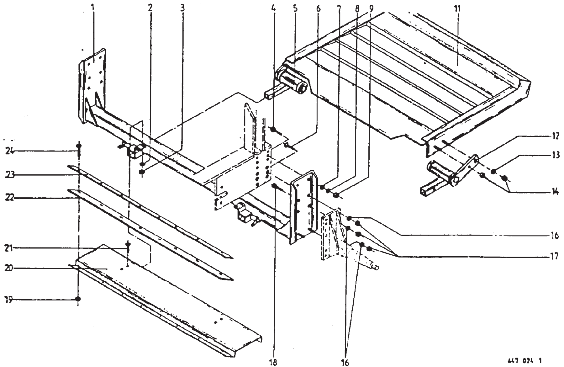
Axle Beam & Bale Ramp
