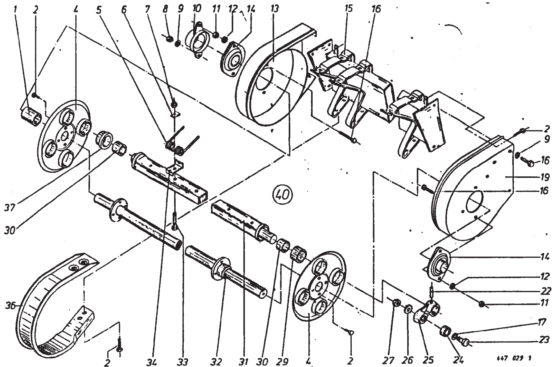
Pickup Drum
