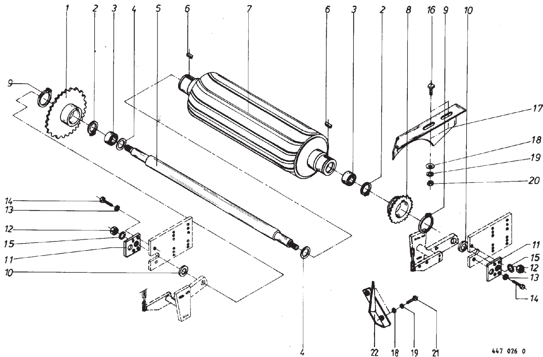
Lower Roller
