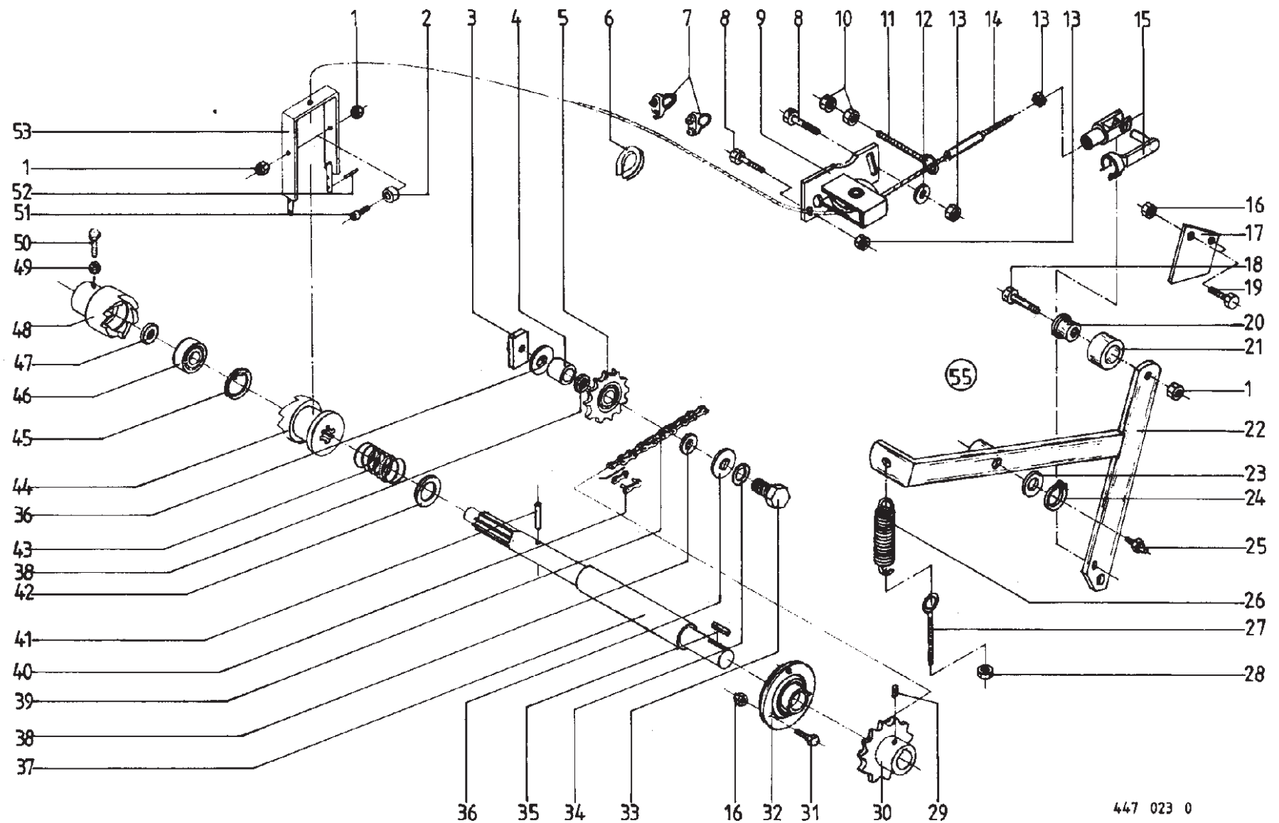
Dog Clutch
