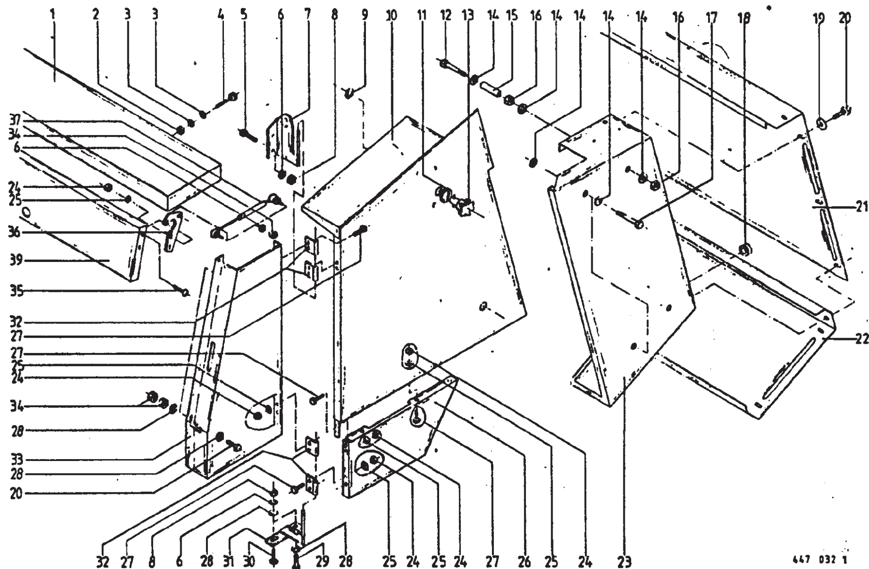
Front & Rear Guards - KR-130
