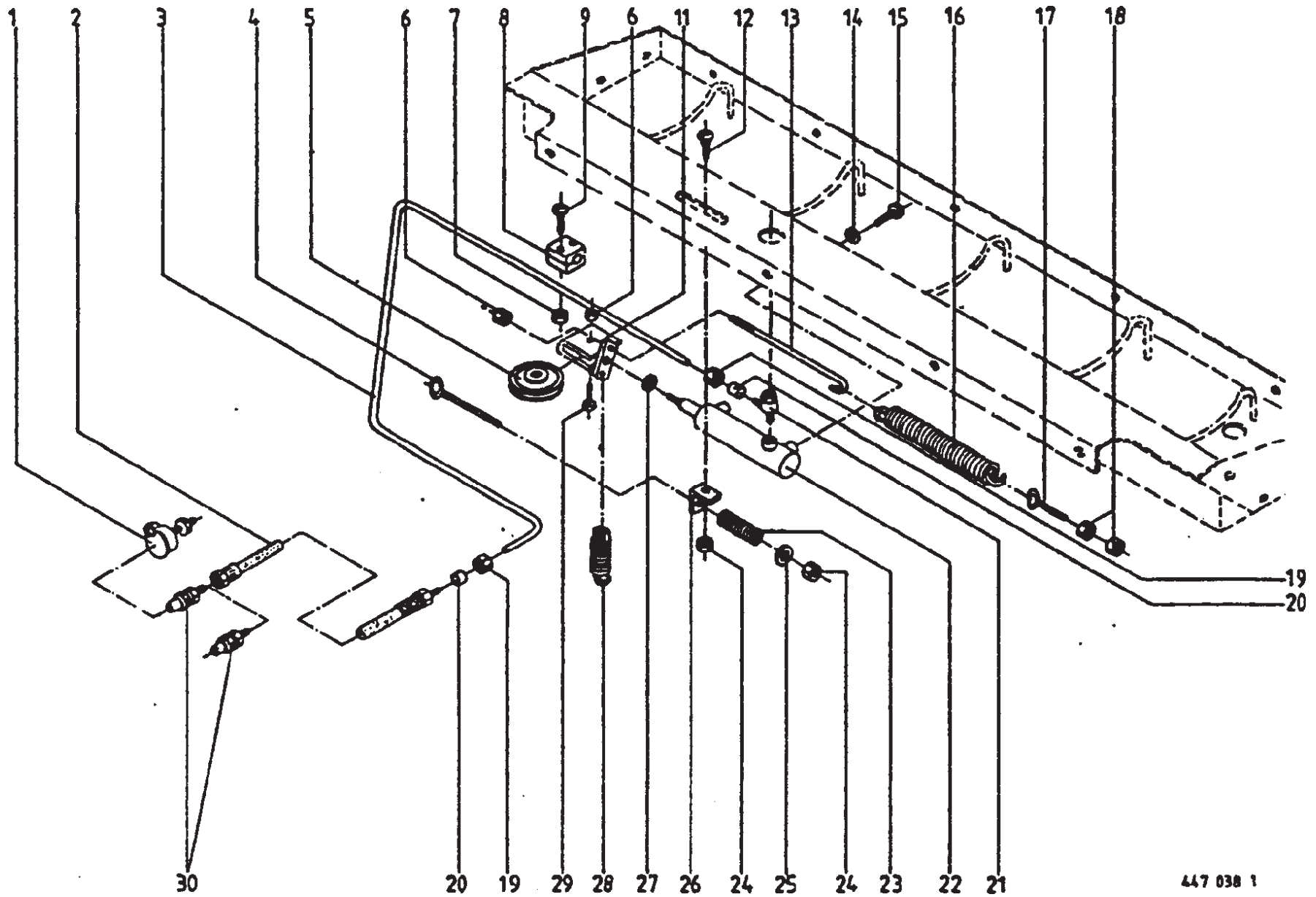
Hydraulic Starter
