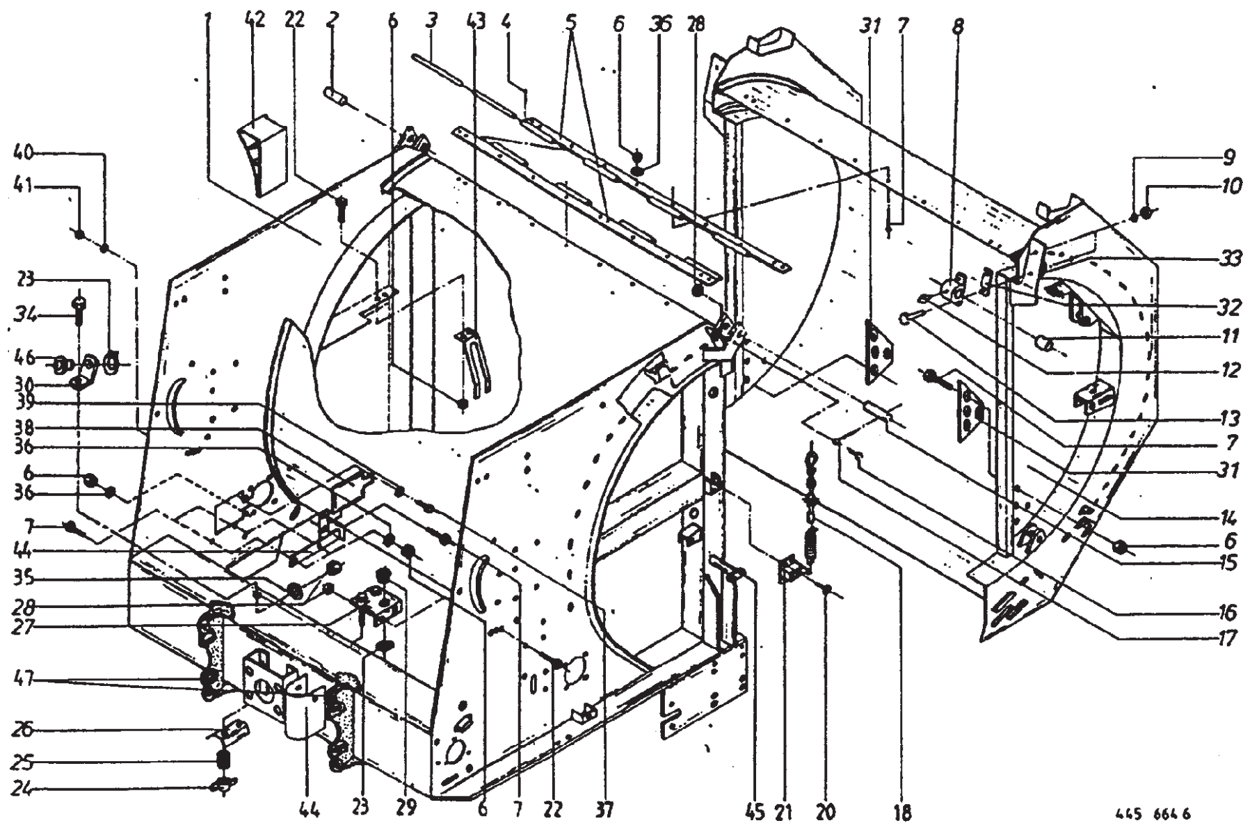
Main Frame
