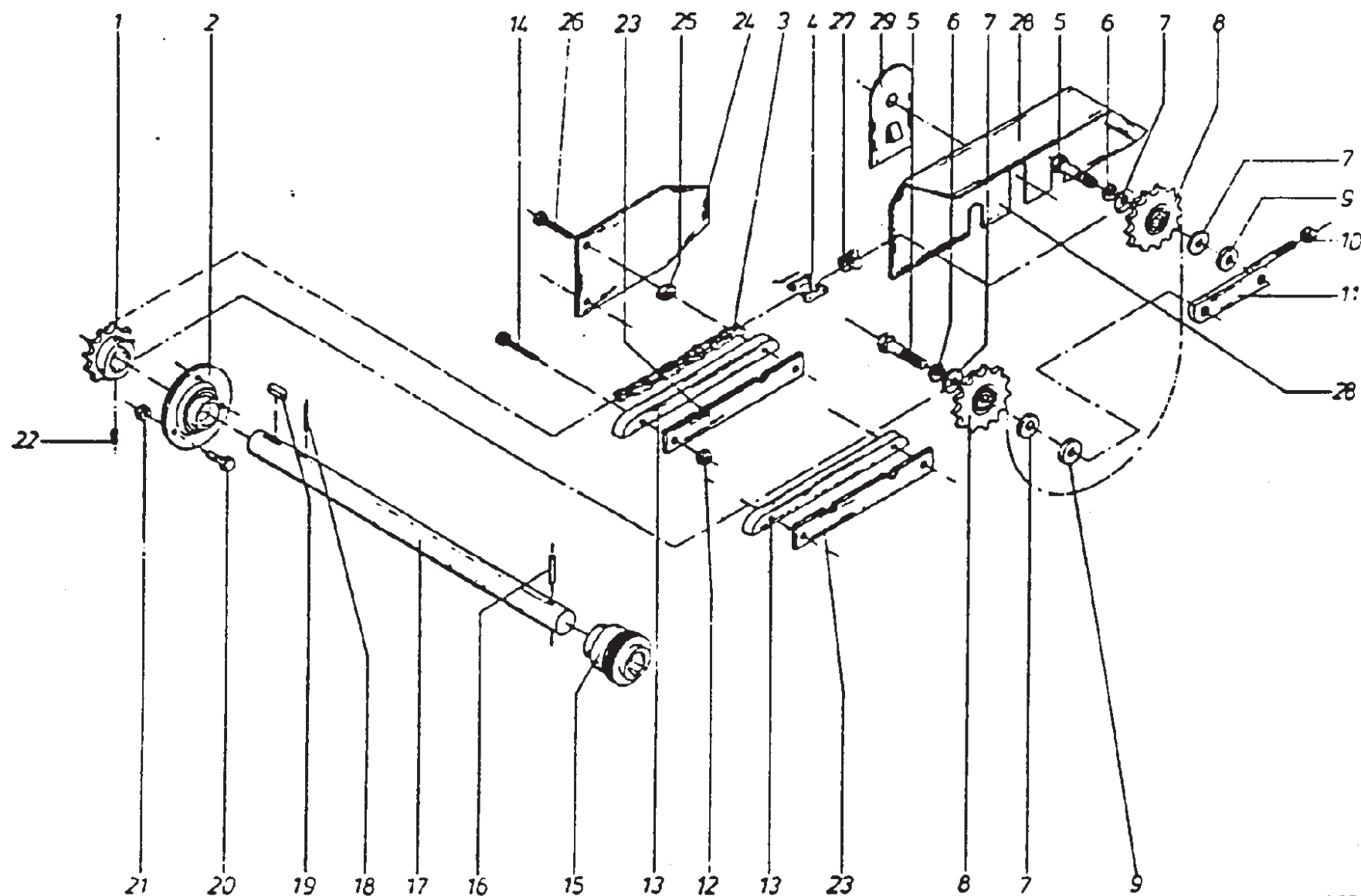
Roller Drive
