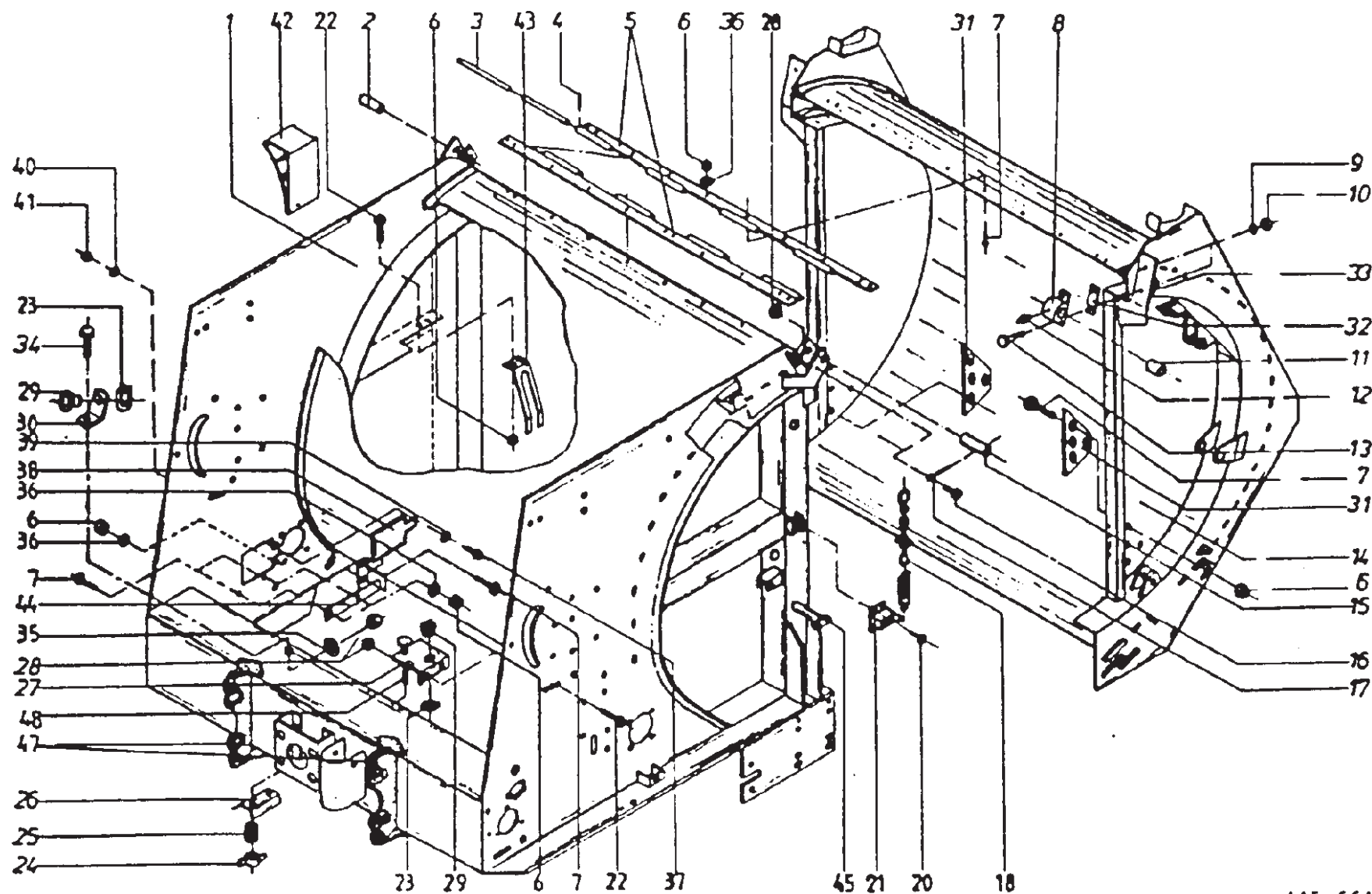
Main Frame
