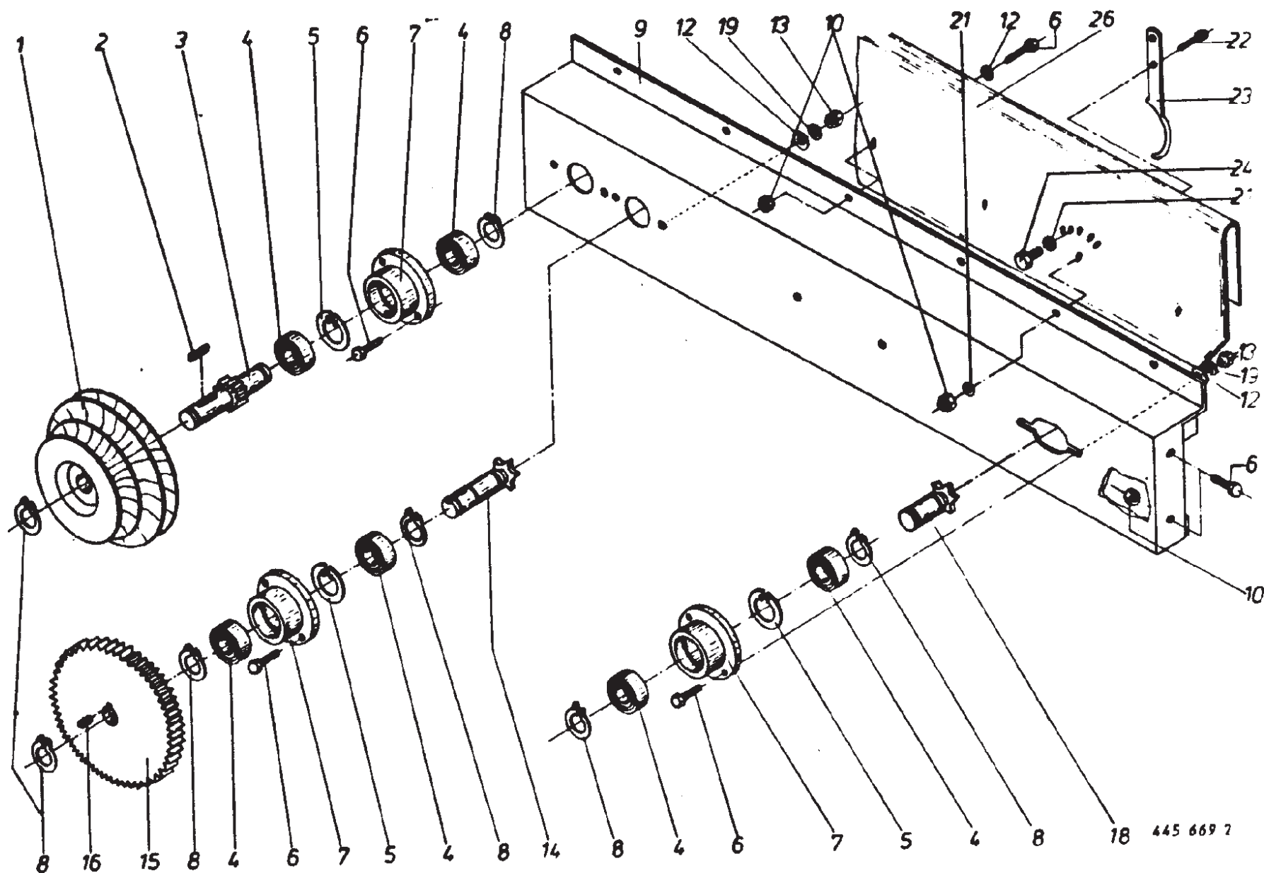
Single Twine Tying Mechanism
