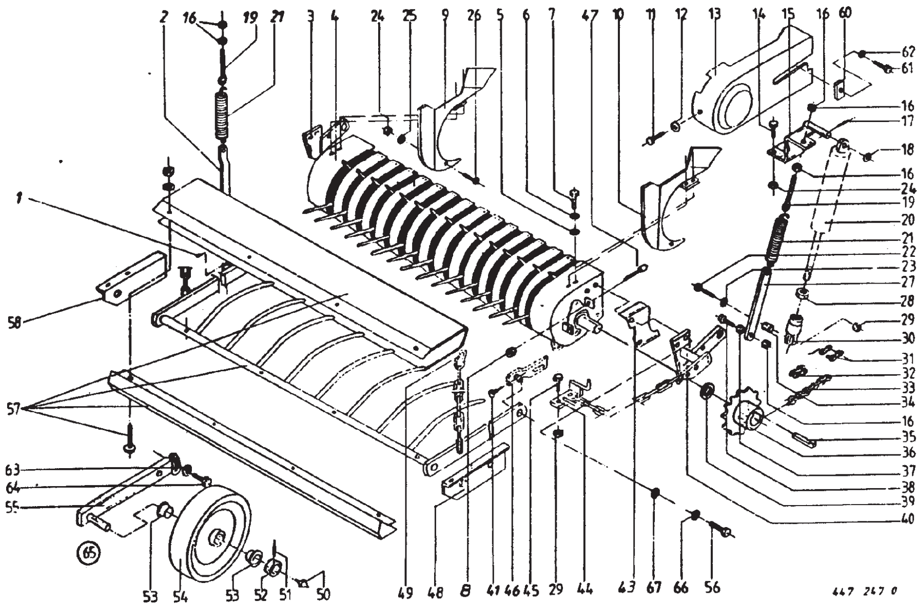
Pickup Mounting
