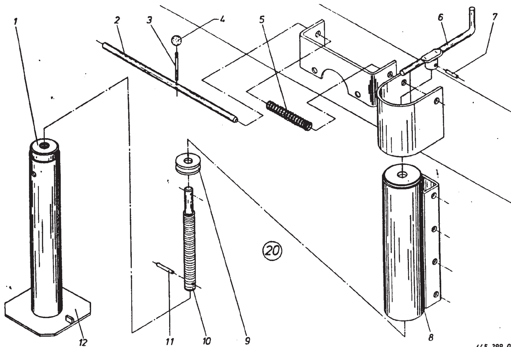
Jack
