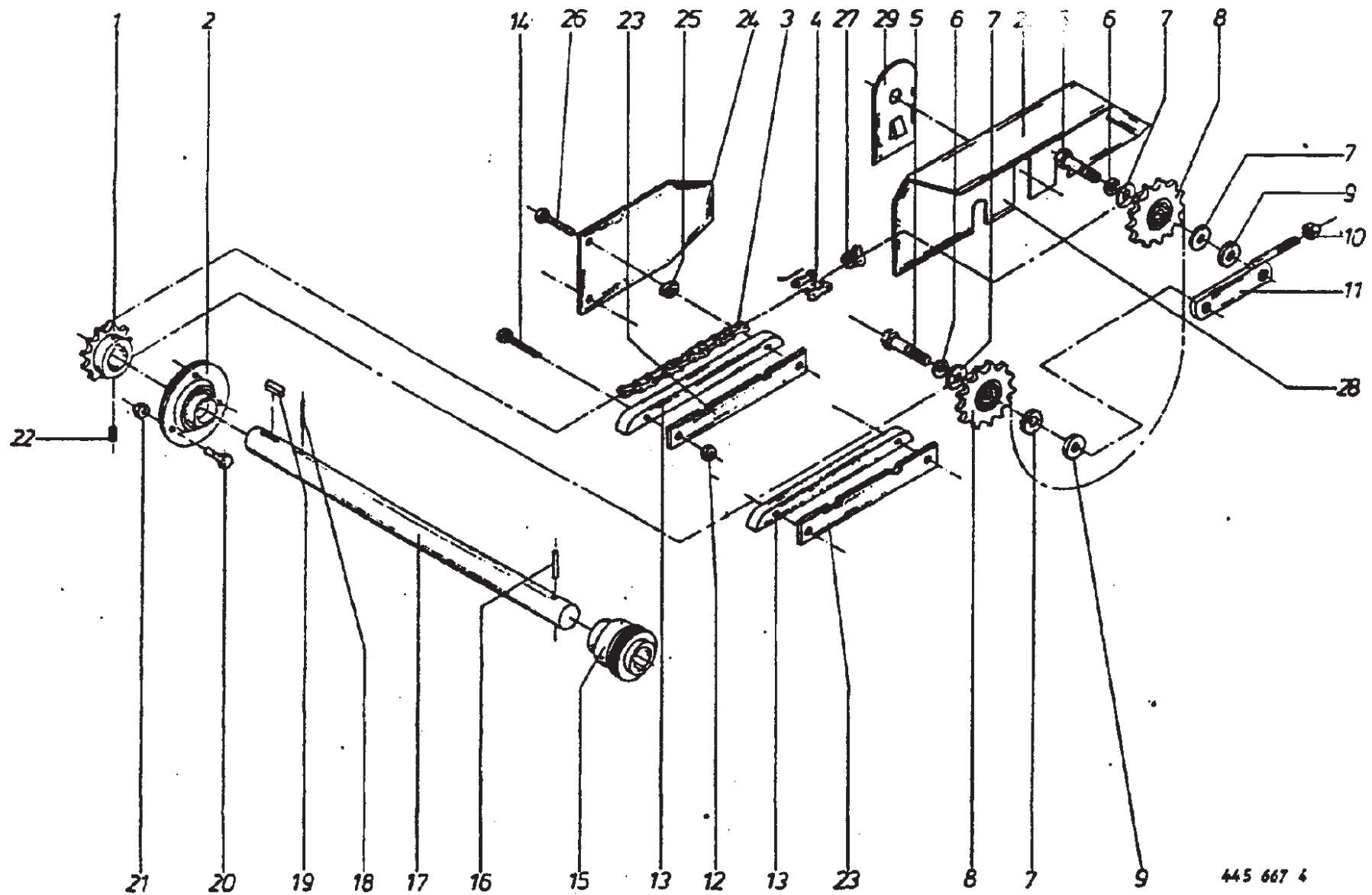
Roller Drive
