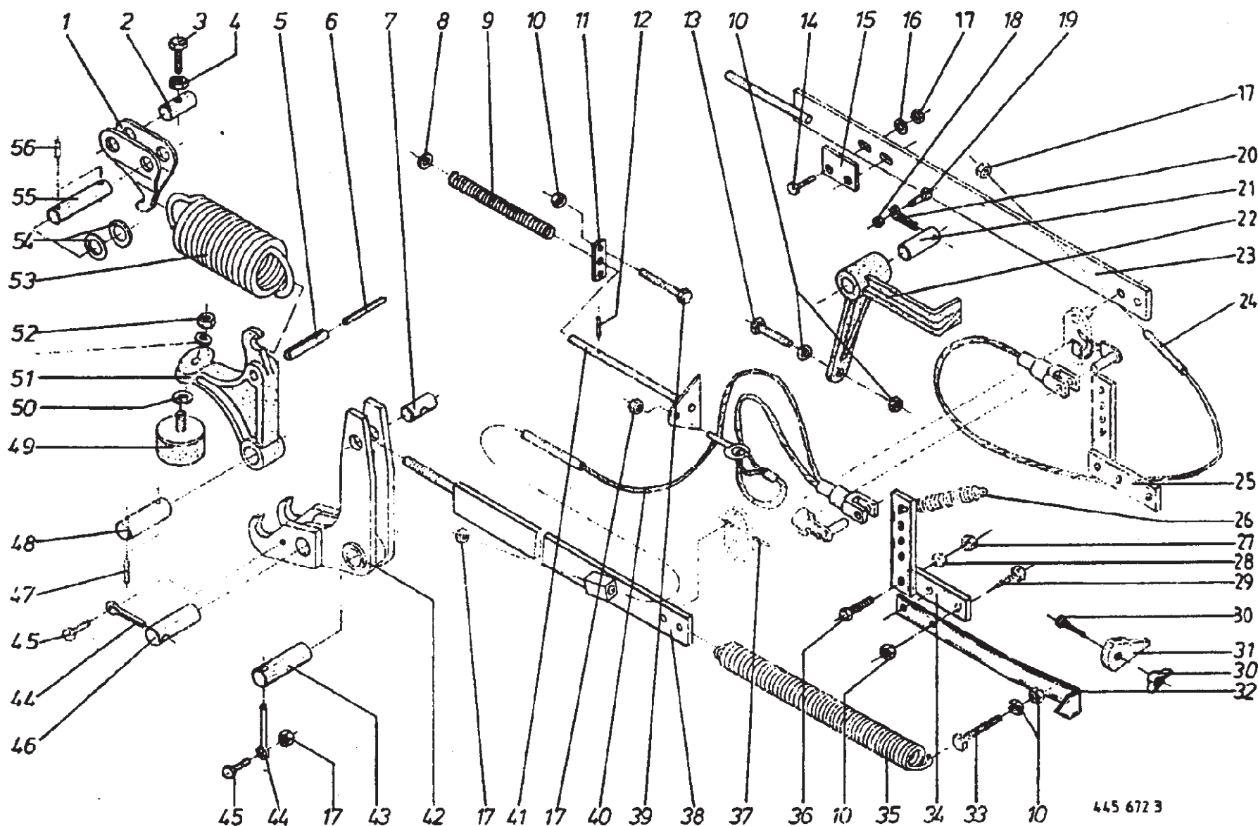
Tailgate Locking Mechanism
