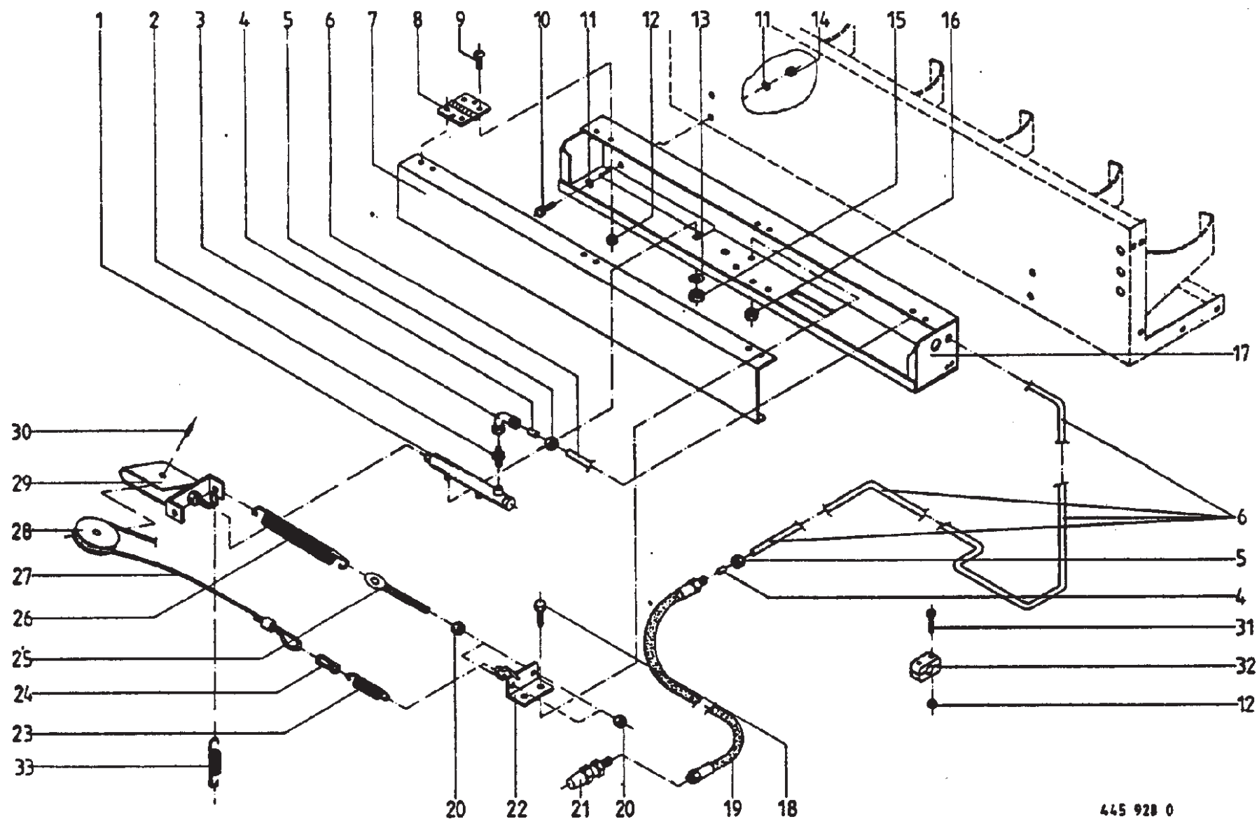
Hydraulic Starter
