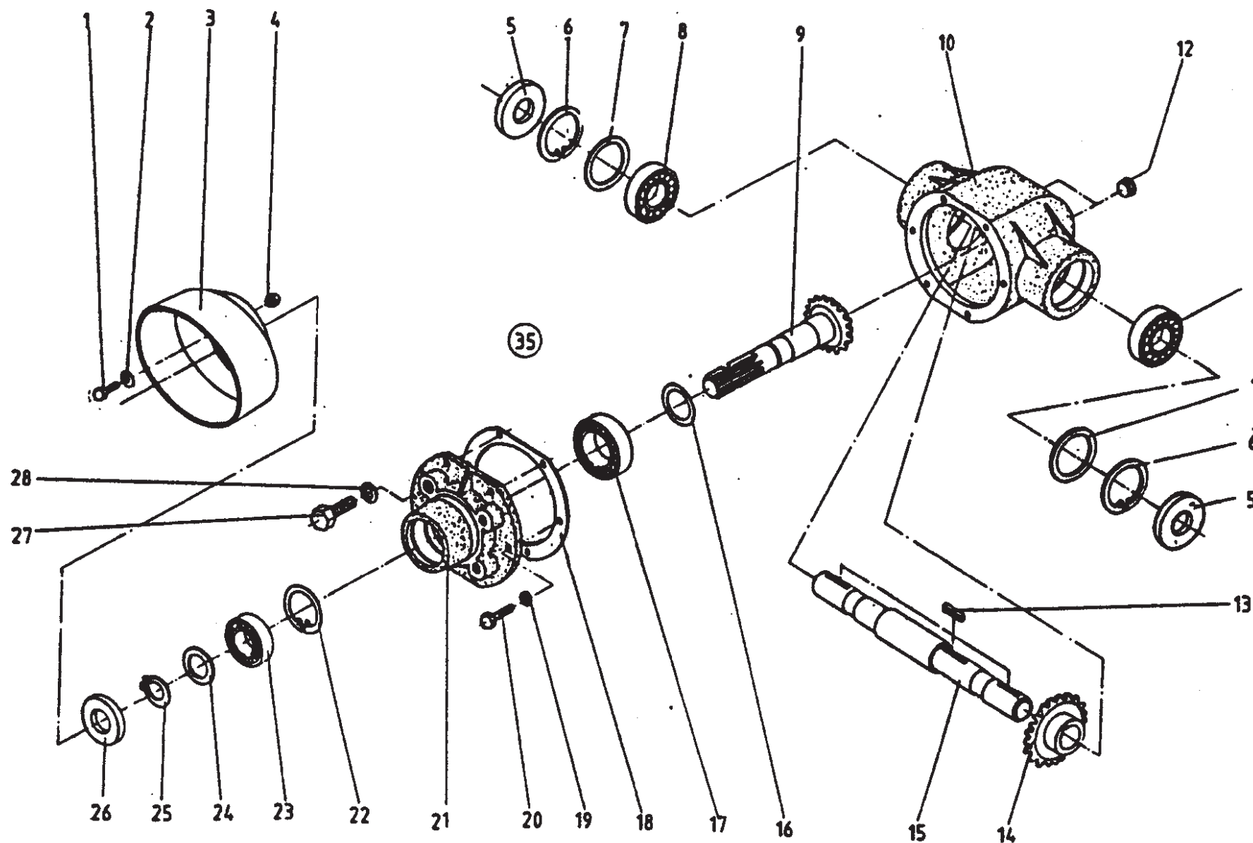
Gearbox
