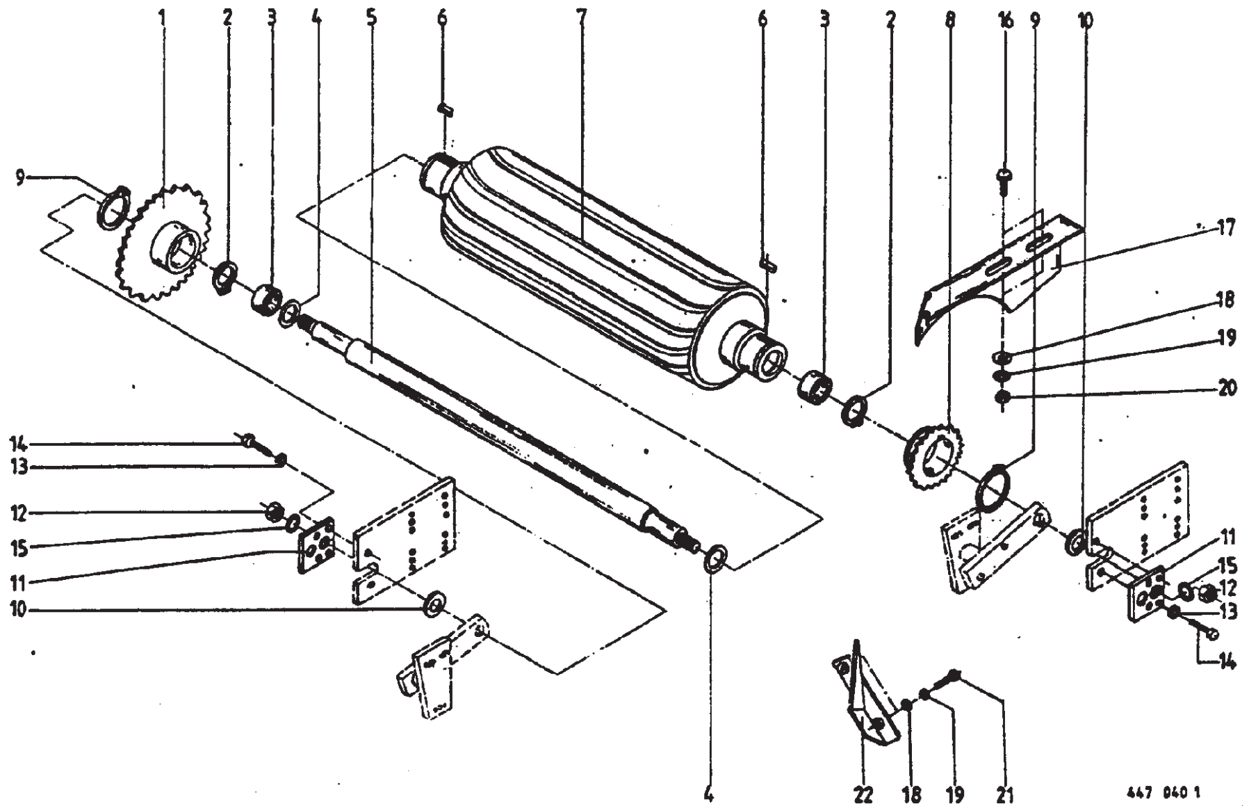
Lower Roller
