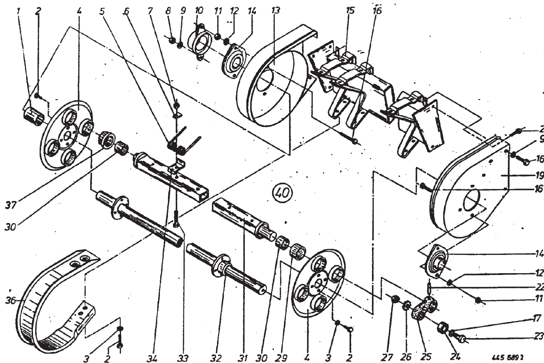
Pickup Drum
