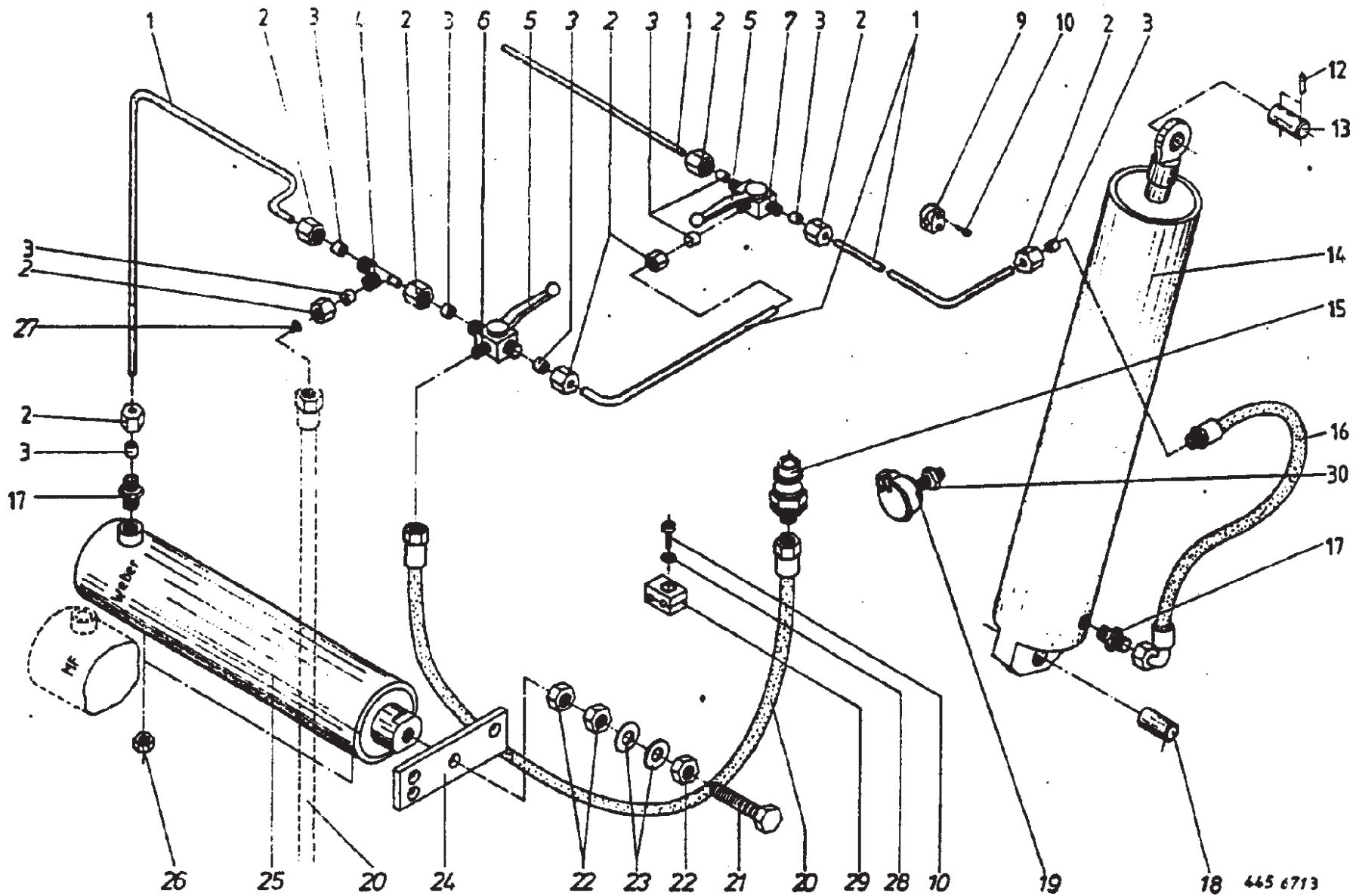
Hydraulic System
