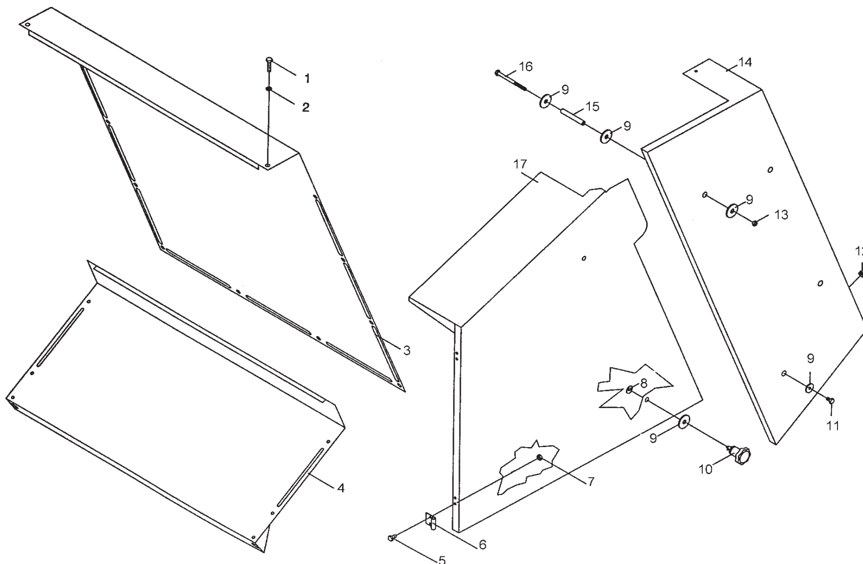
Rear Guards
