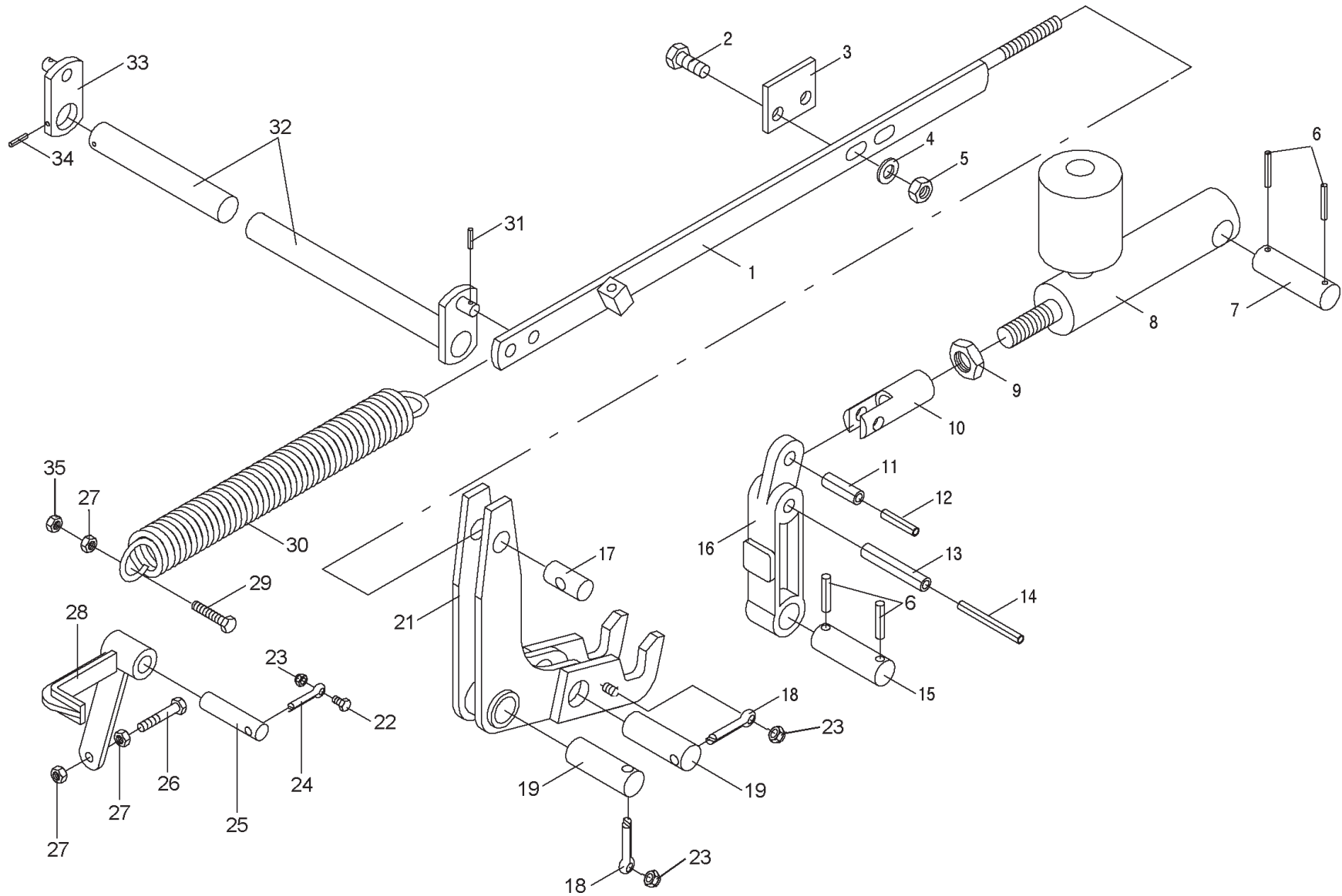
Tailgate Locking Mechanism
