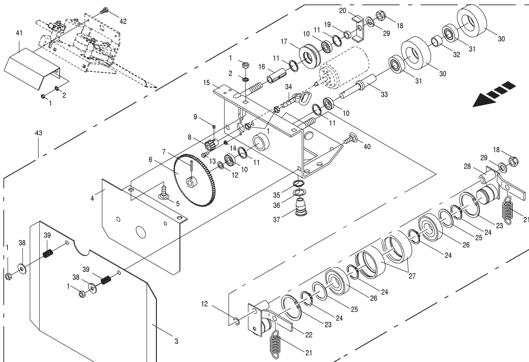
Electric Twine Starter
