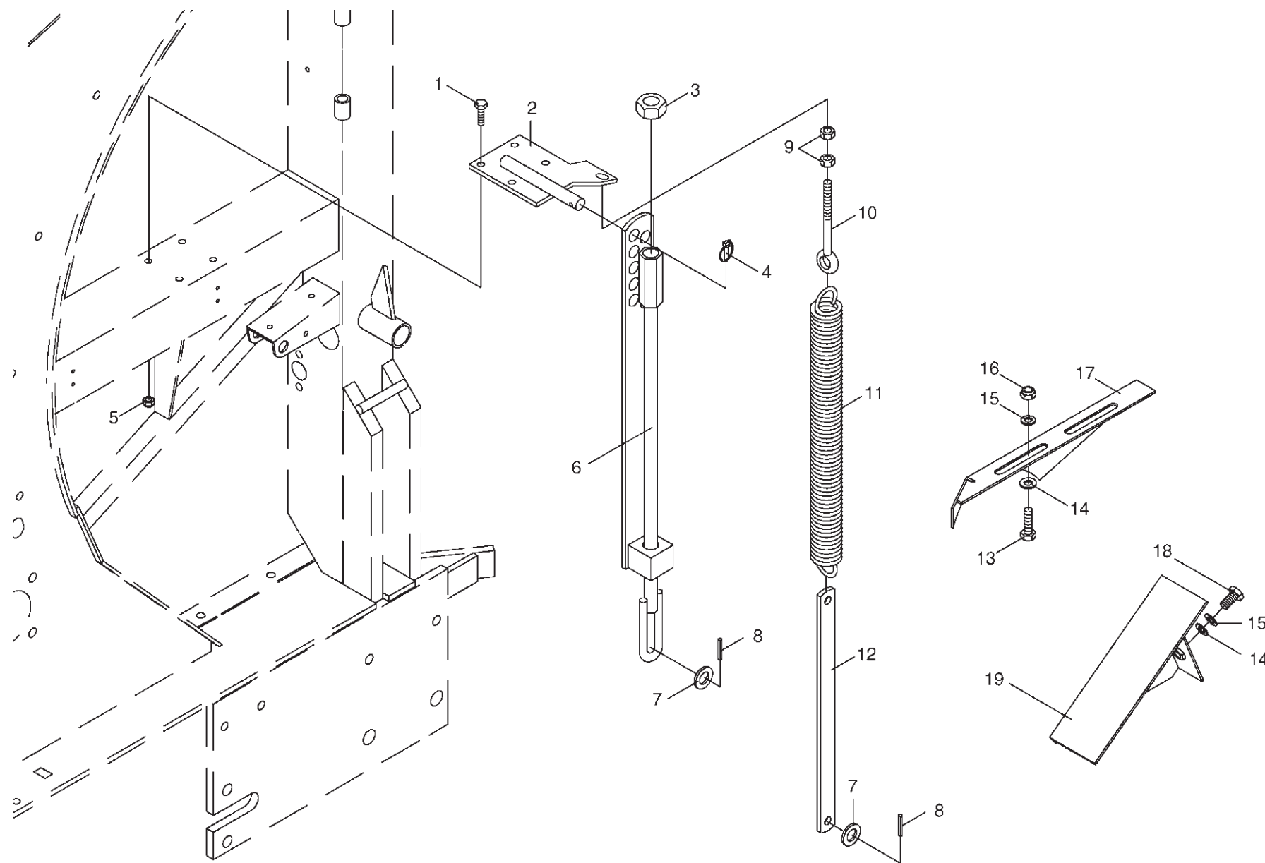
Wide Pickup Flotation
