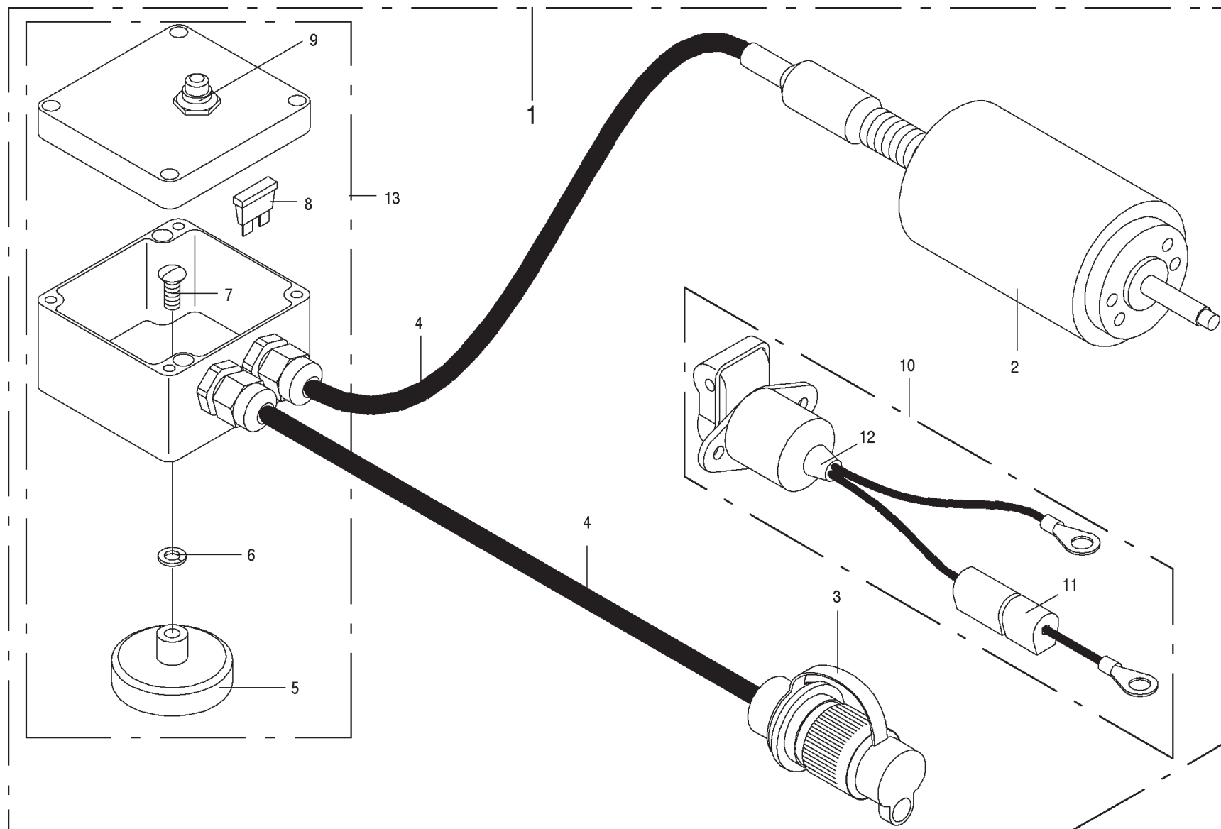
Electric Twine Starter Box
