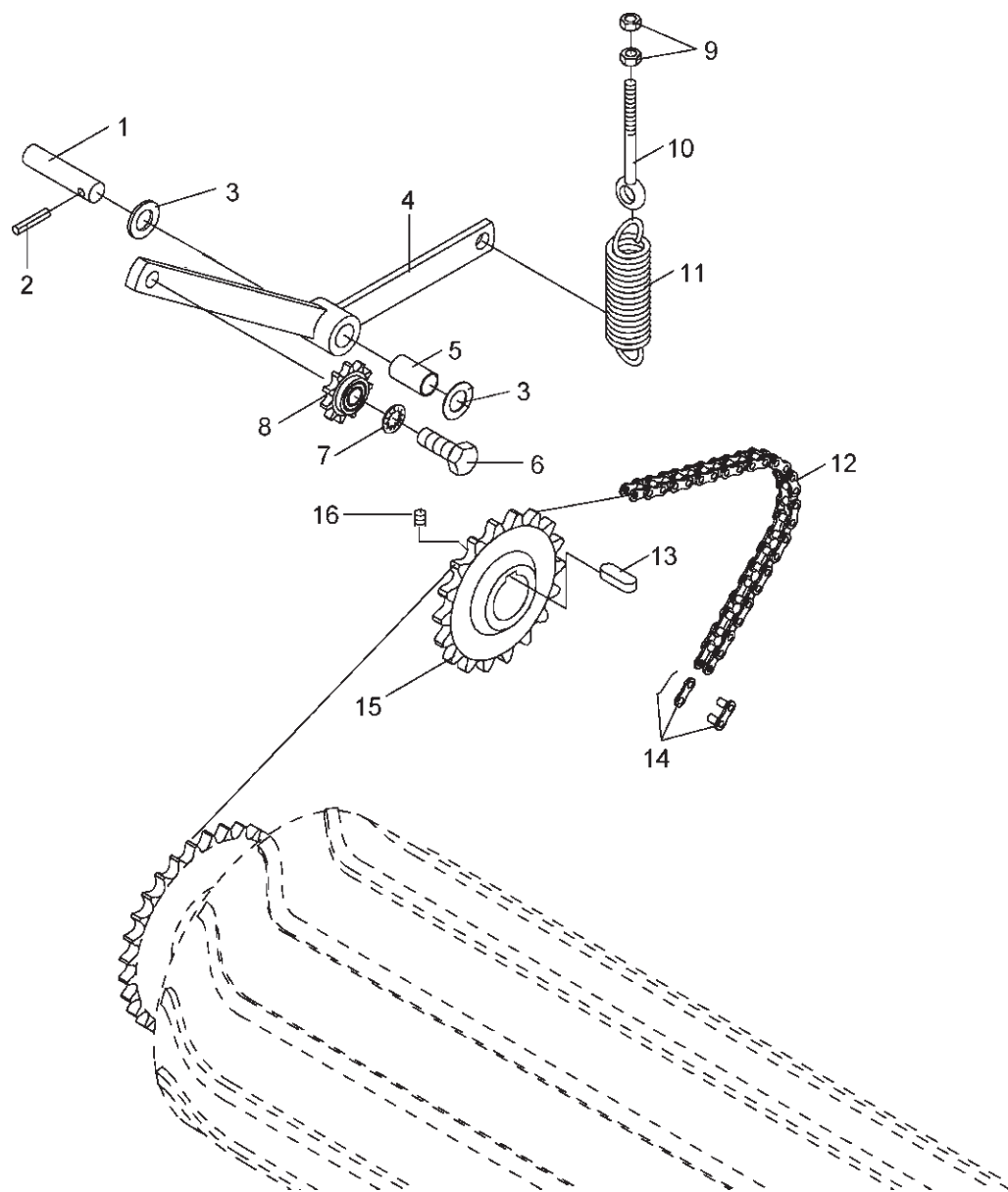
Right Hand Roller Drive
