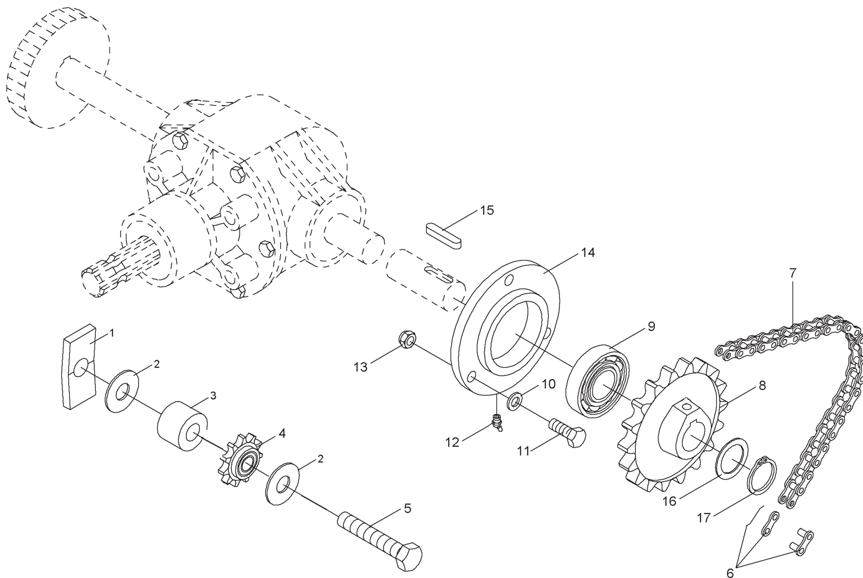
Left Hand Front Drive
