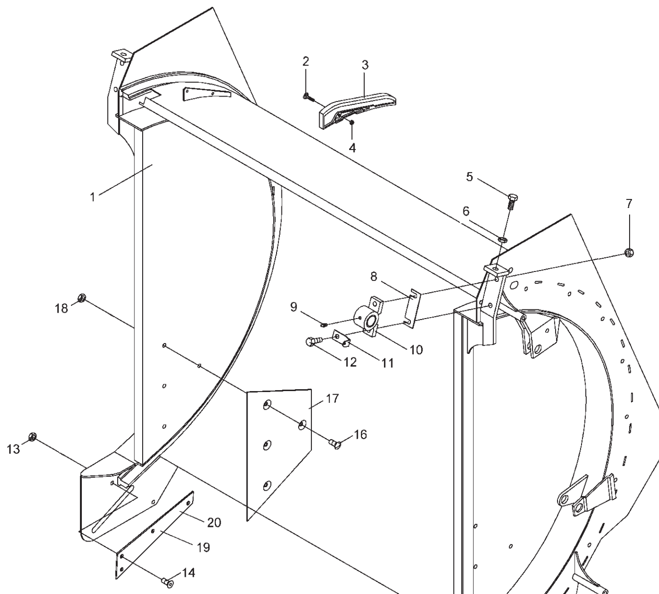
Rear Frame
