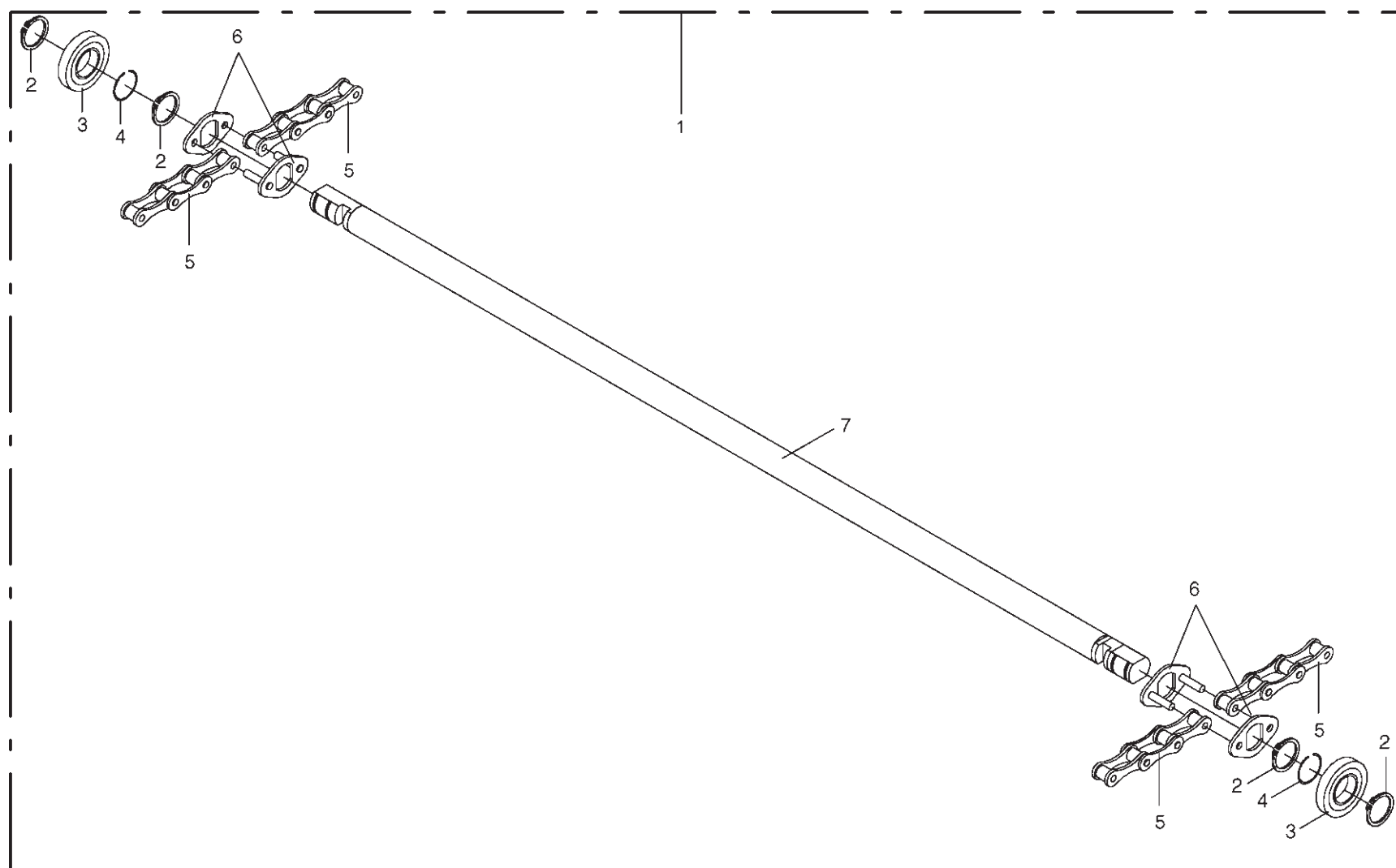
Elevator Chain
