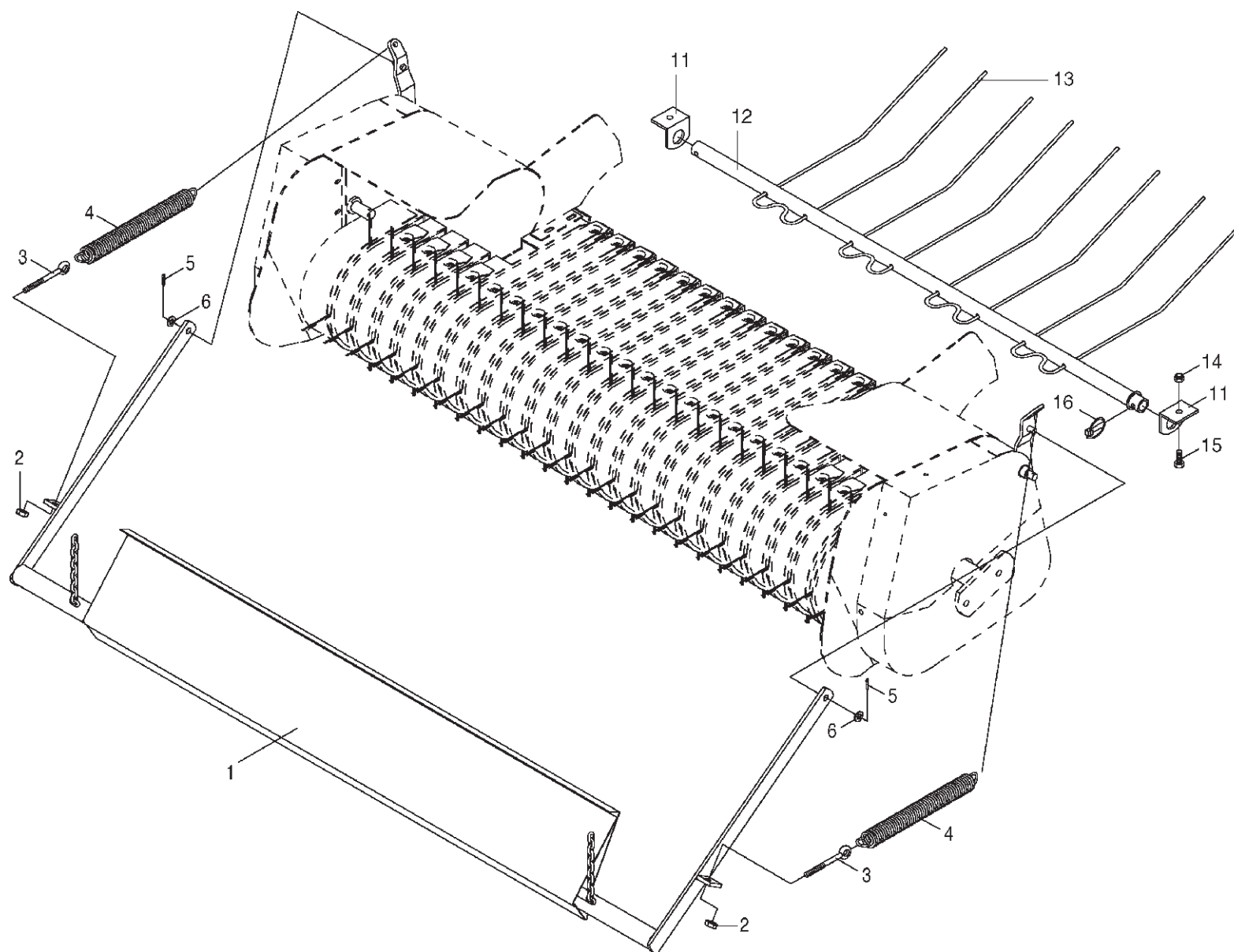
Compressing Rake
