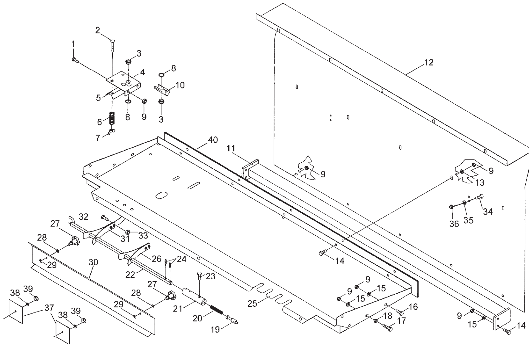
Twine Box
