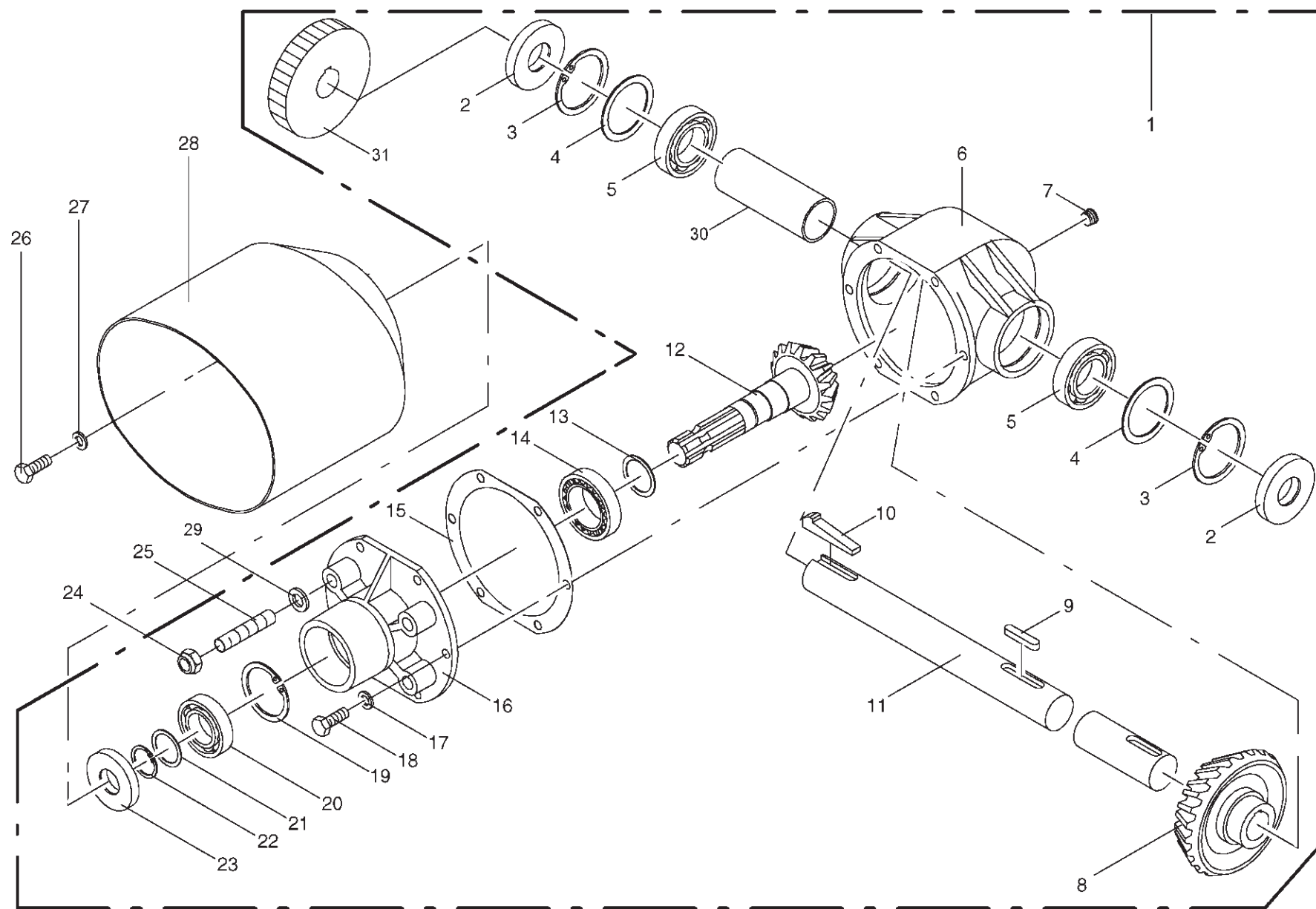
Gearbox
