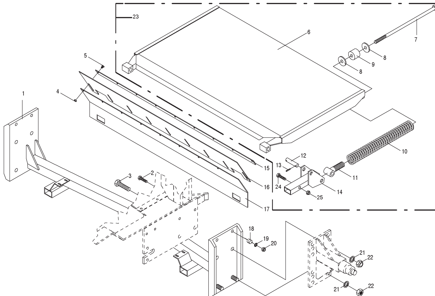
Axle Beam and Bale Ramp
