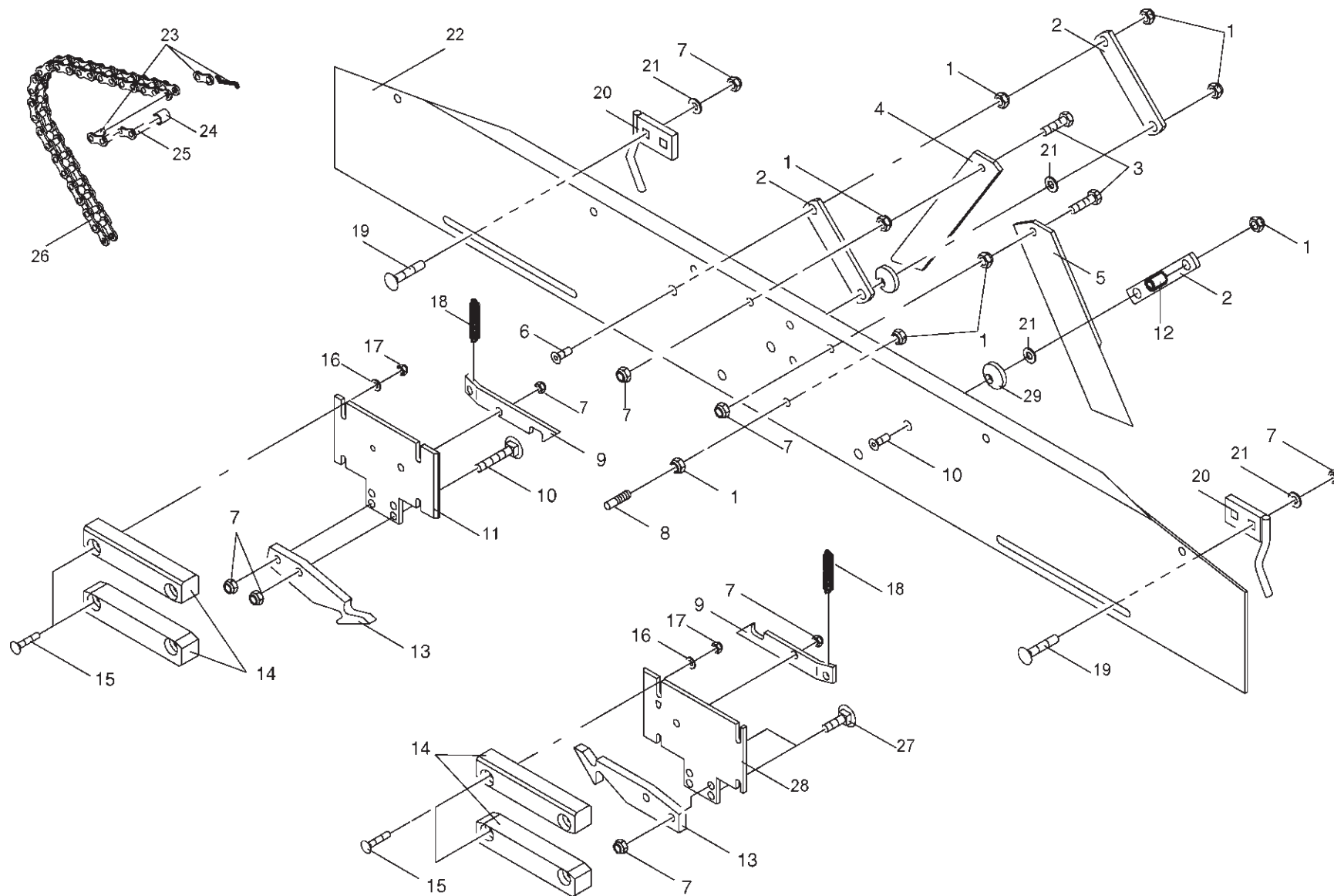
Double Twine Tying Cutting Unit
