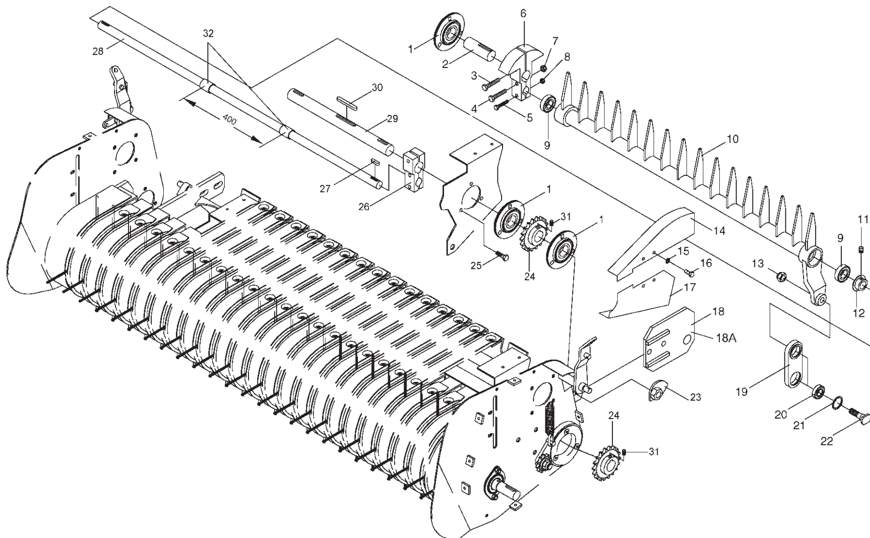
Wide Pickup Feed Rake Assembly
