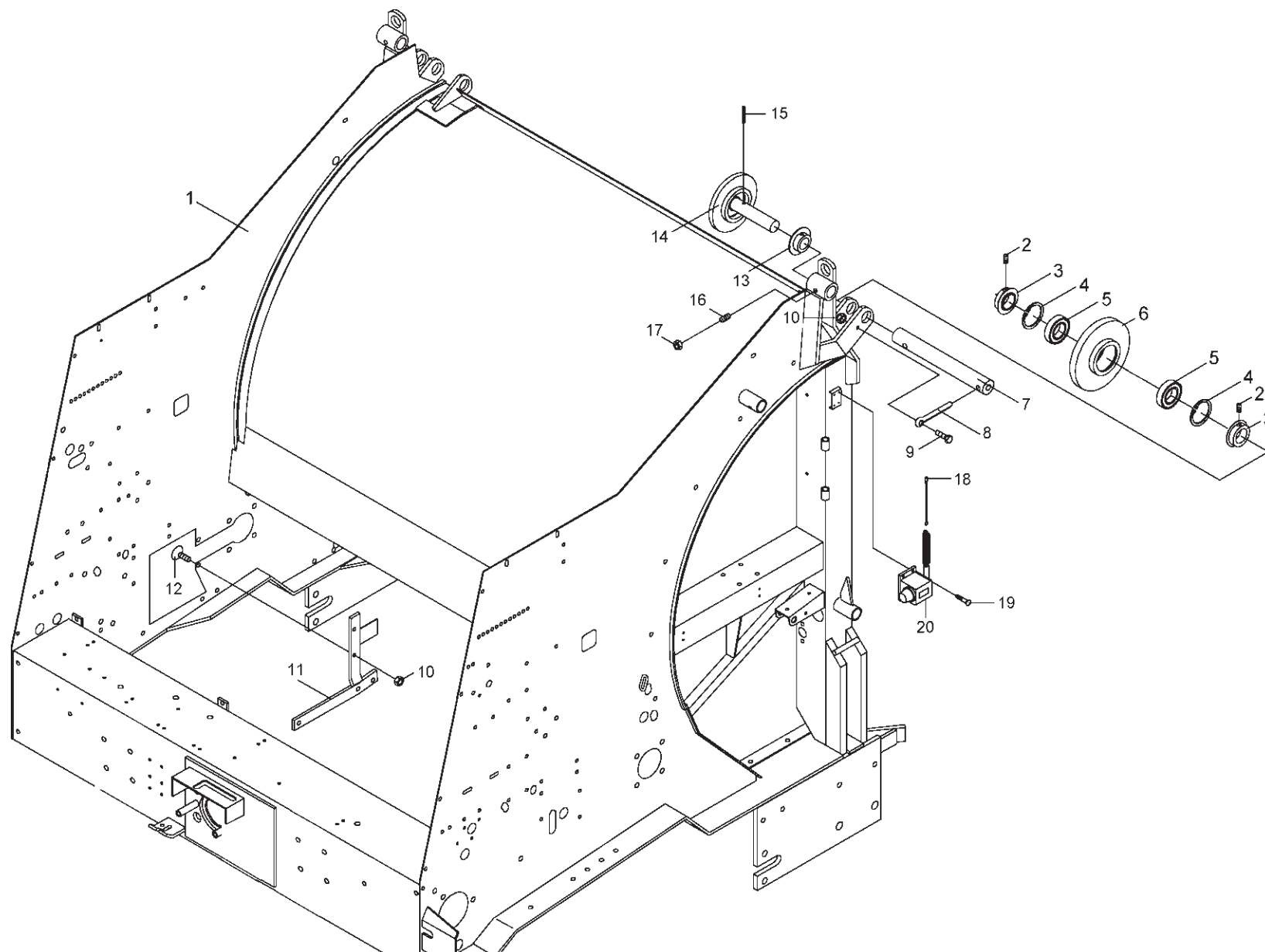
Front Frame
