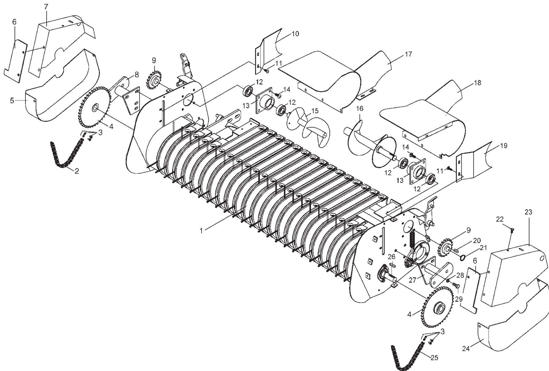
Wide Pickup Augers & Shields
