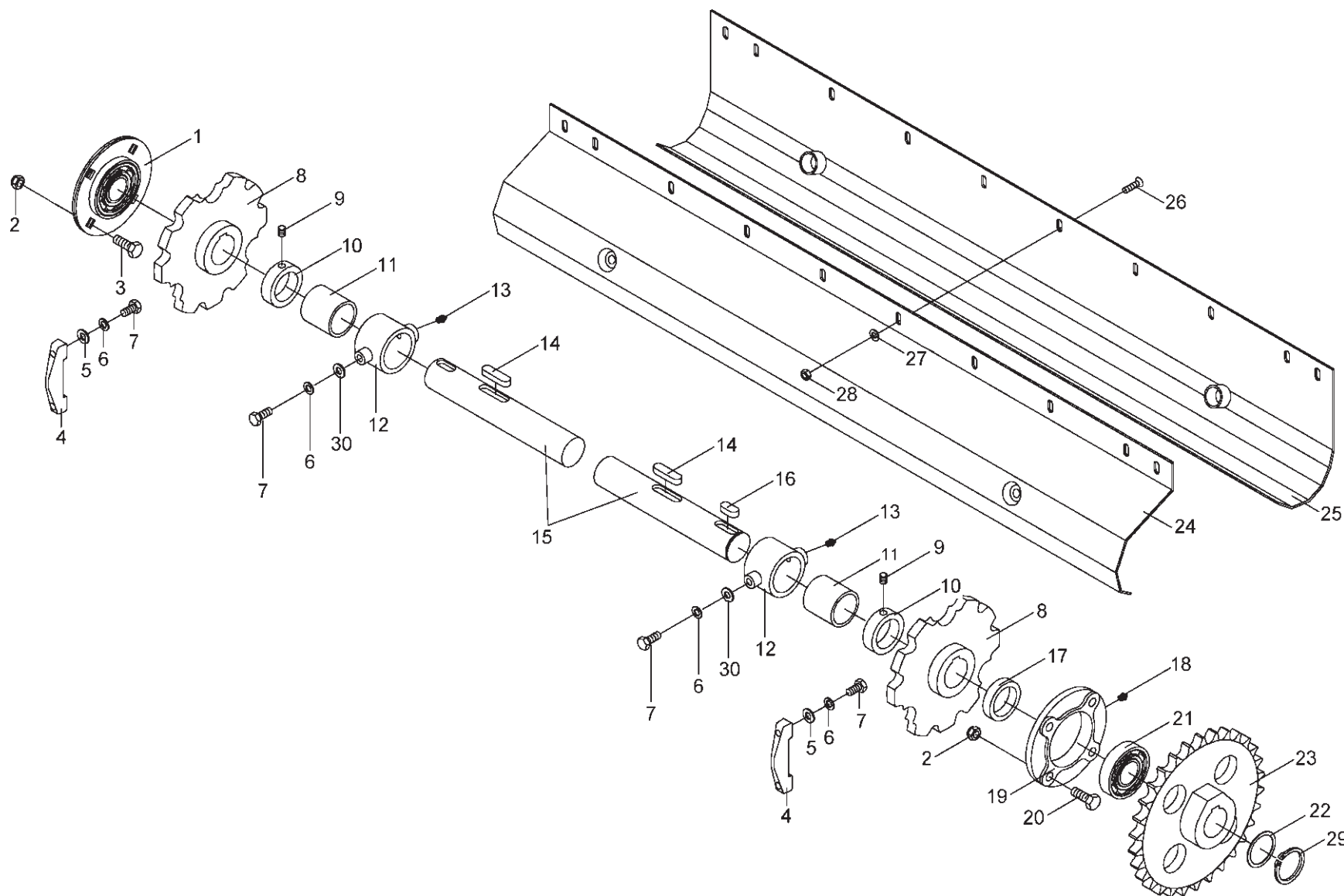
Elevator Chain Drive
