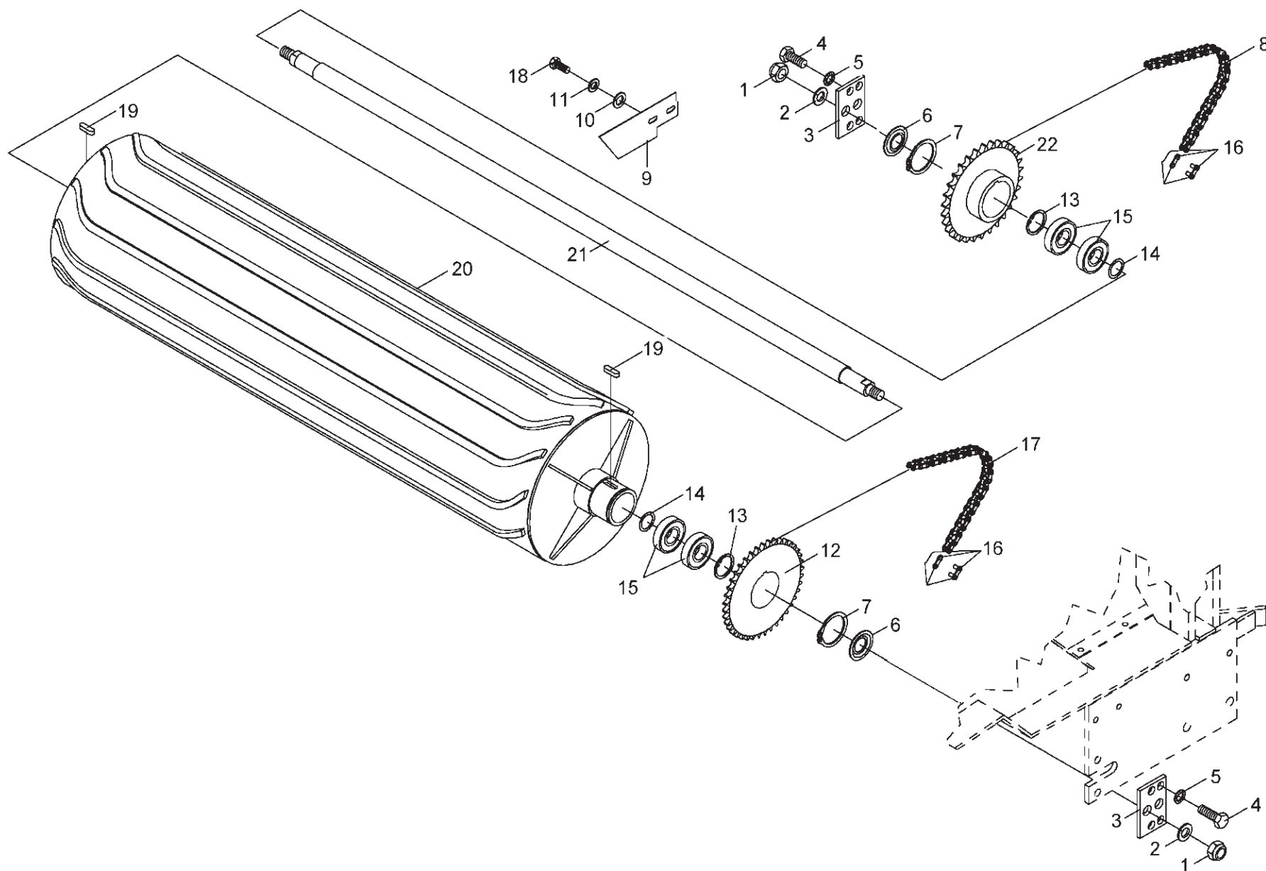
Lower Roller
