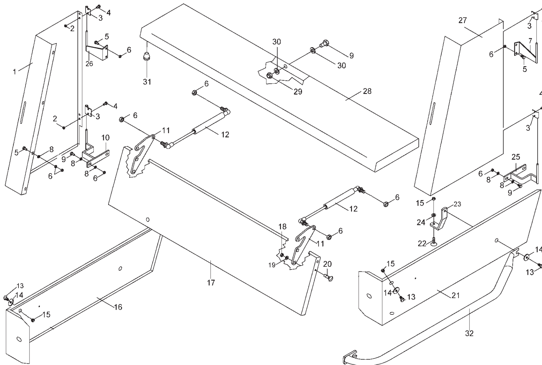
Front Guards
