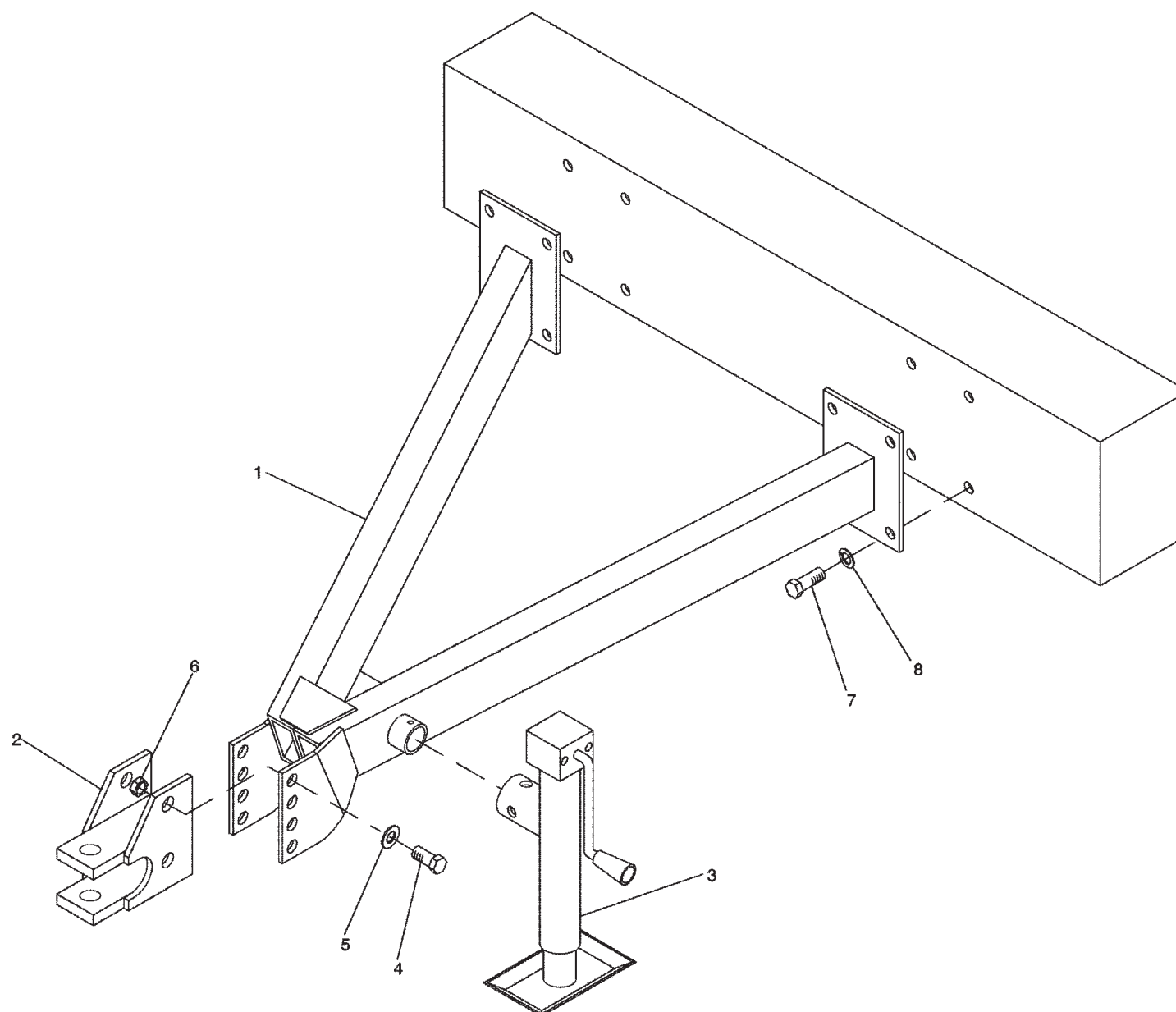
Drawbar
