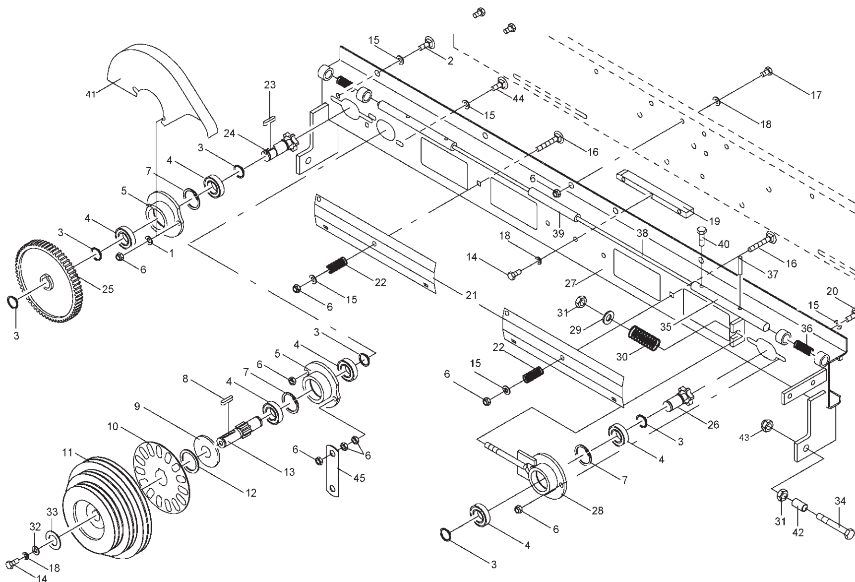
Double Twine Tying Mechanism
