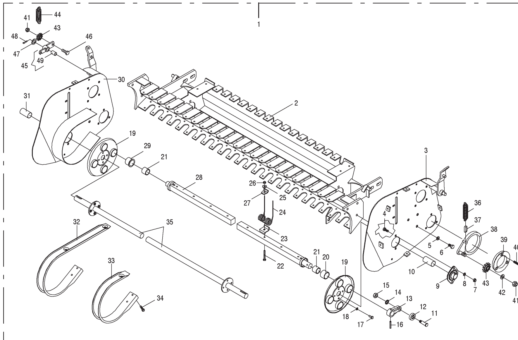
Wide Pickup Drum
