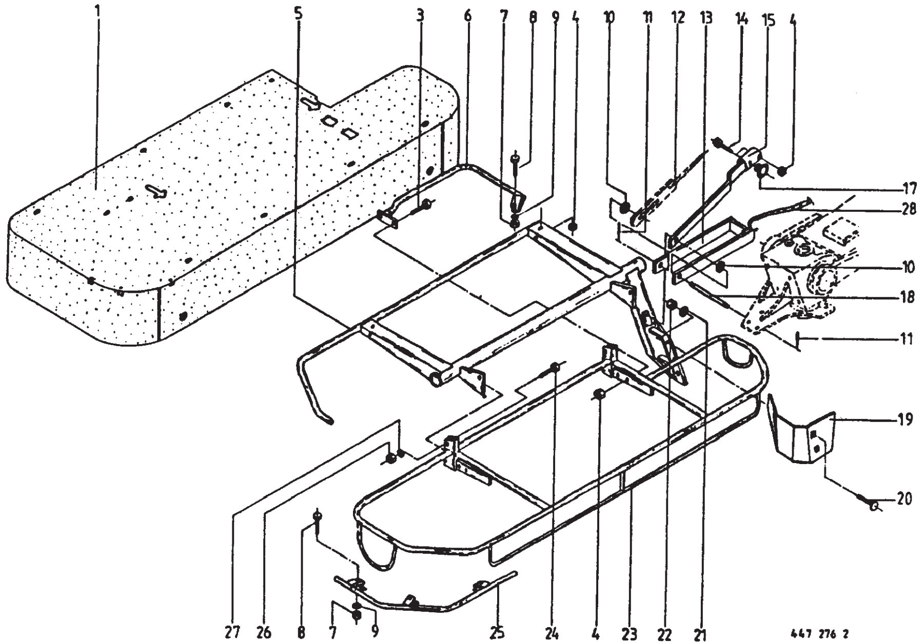
Safety Frames
