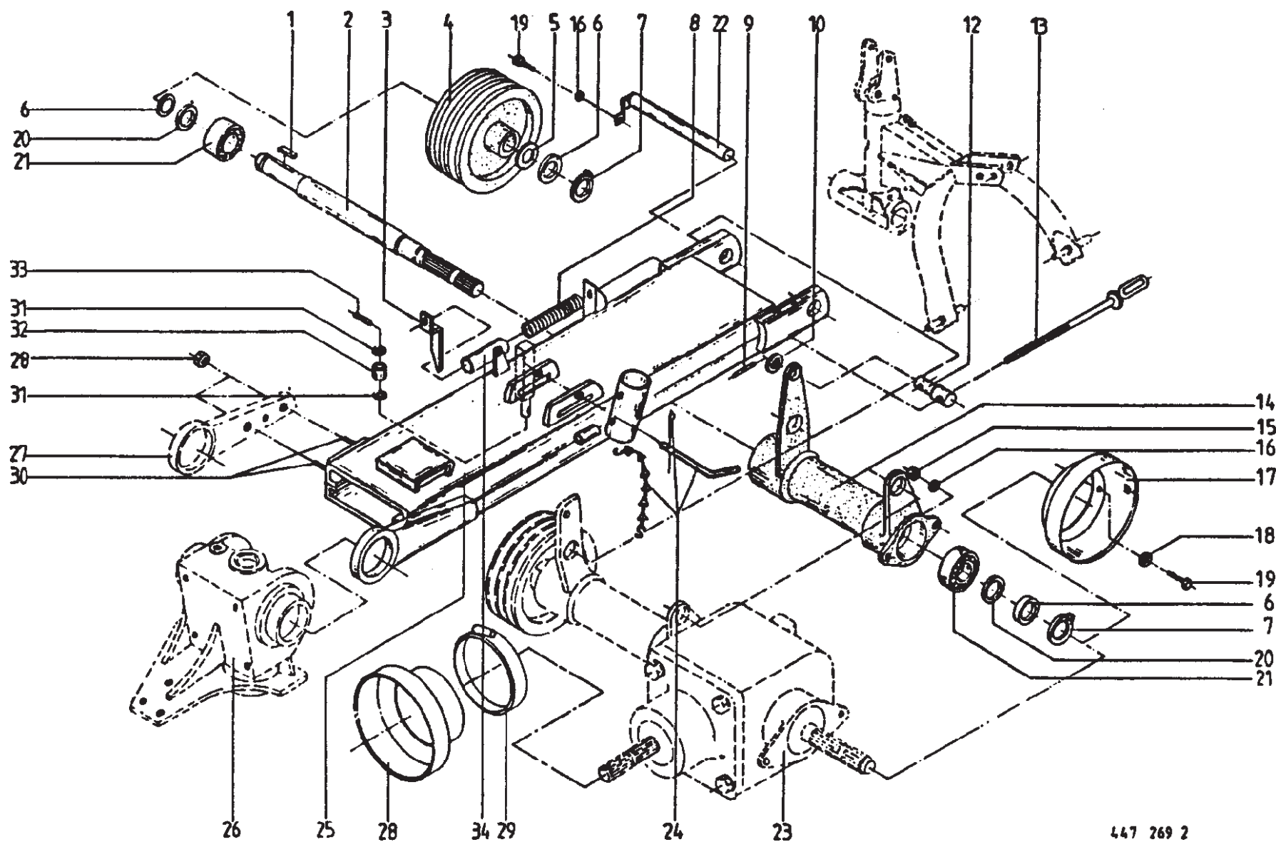
Carrier Beam
