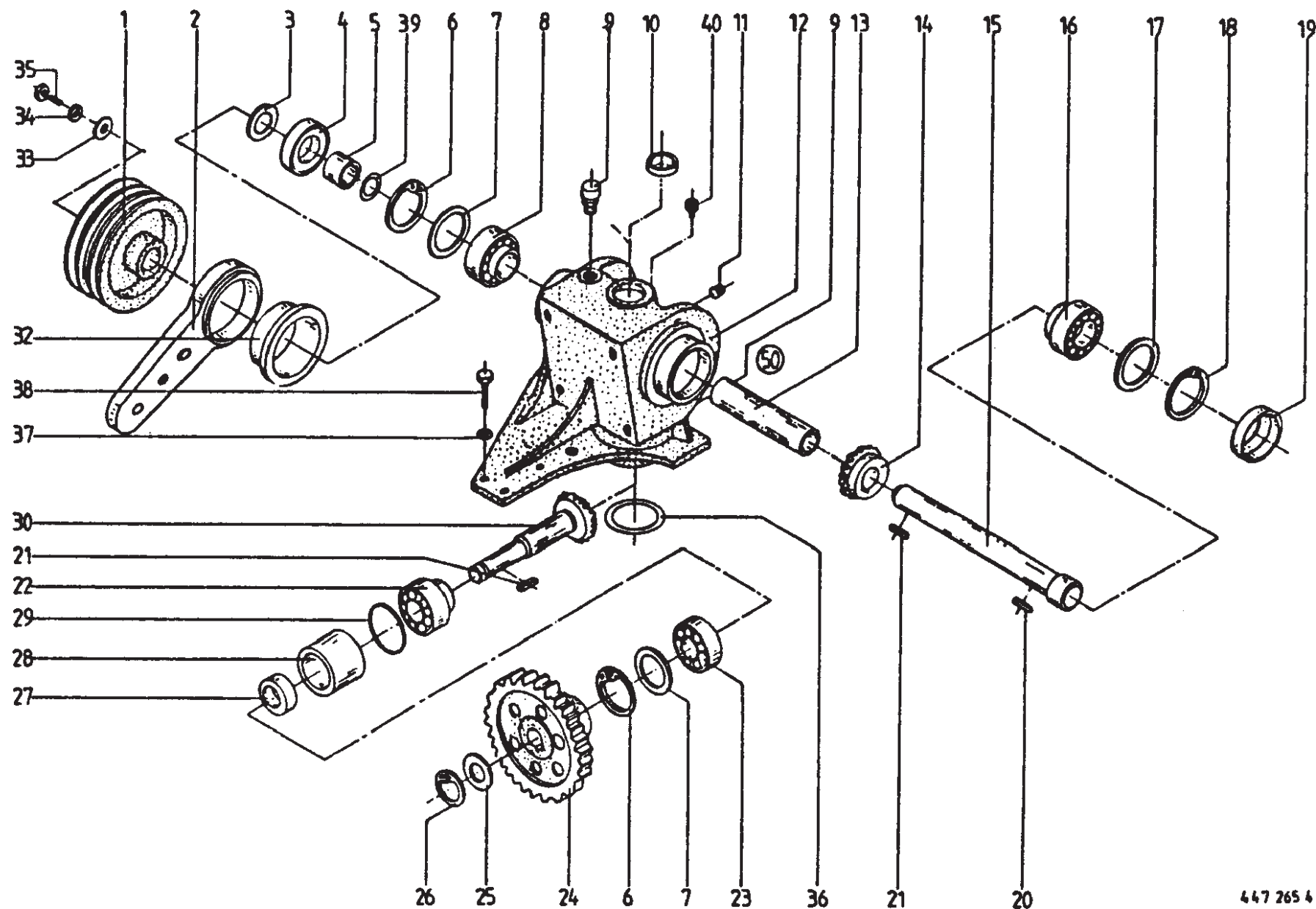
Main Gearbox
