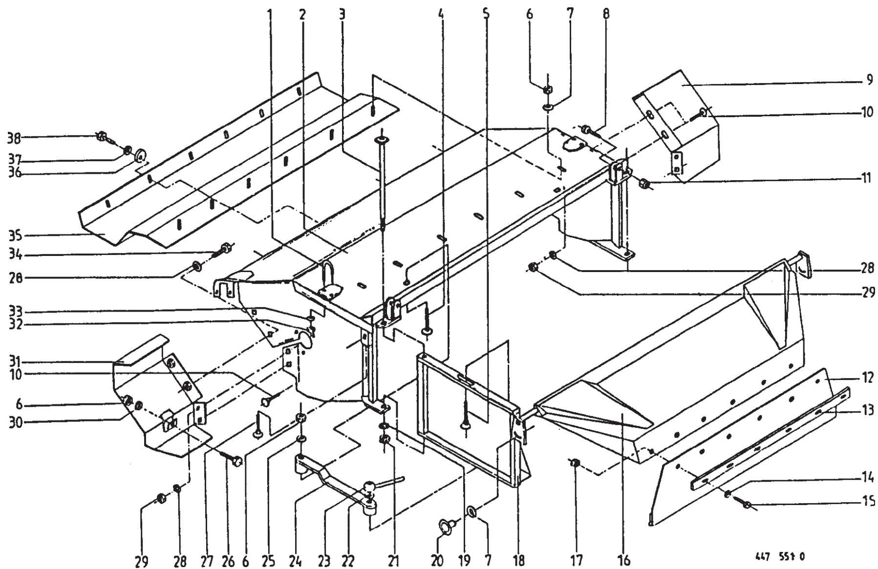
Conditioner Housing - AM-282Z
