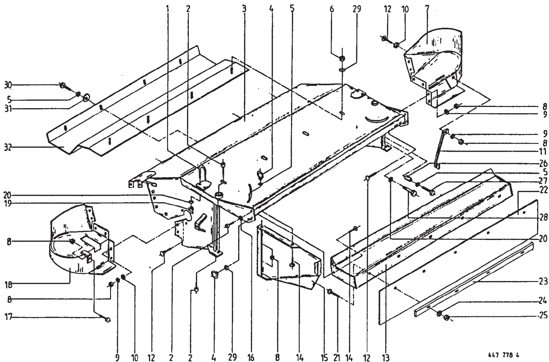
Conditioner Housing - AM-202Z
