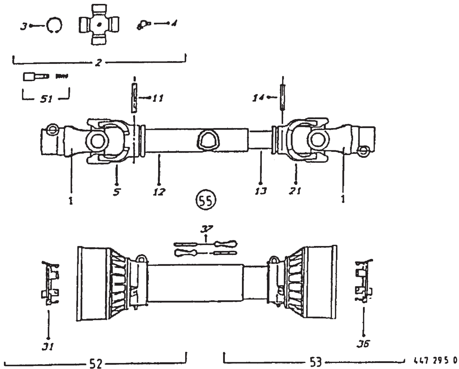
Conditioner PTO Shaft - Bondioli - AM-202Z
