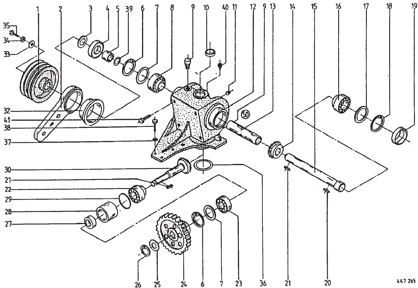
Main Gearbox
