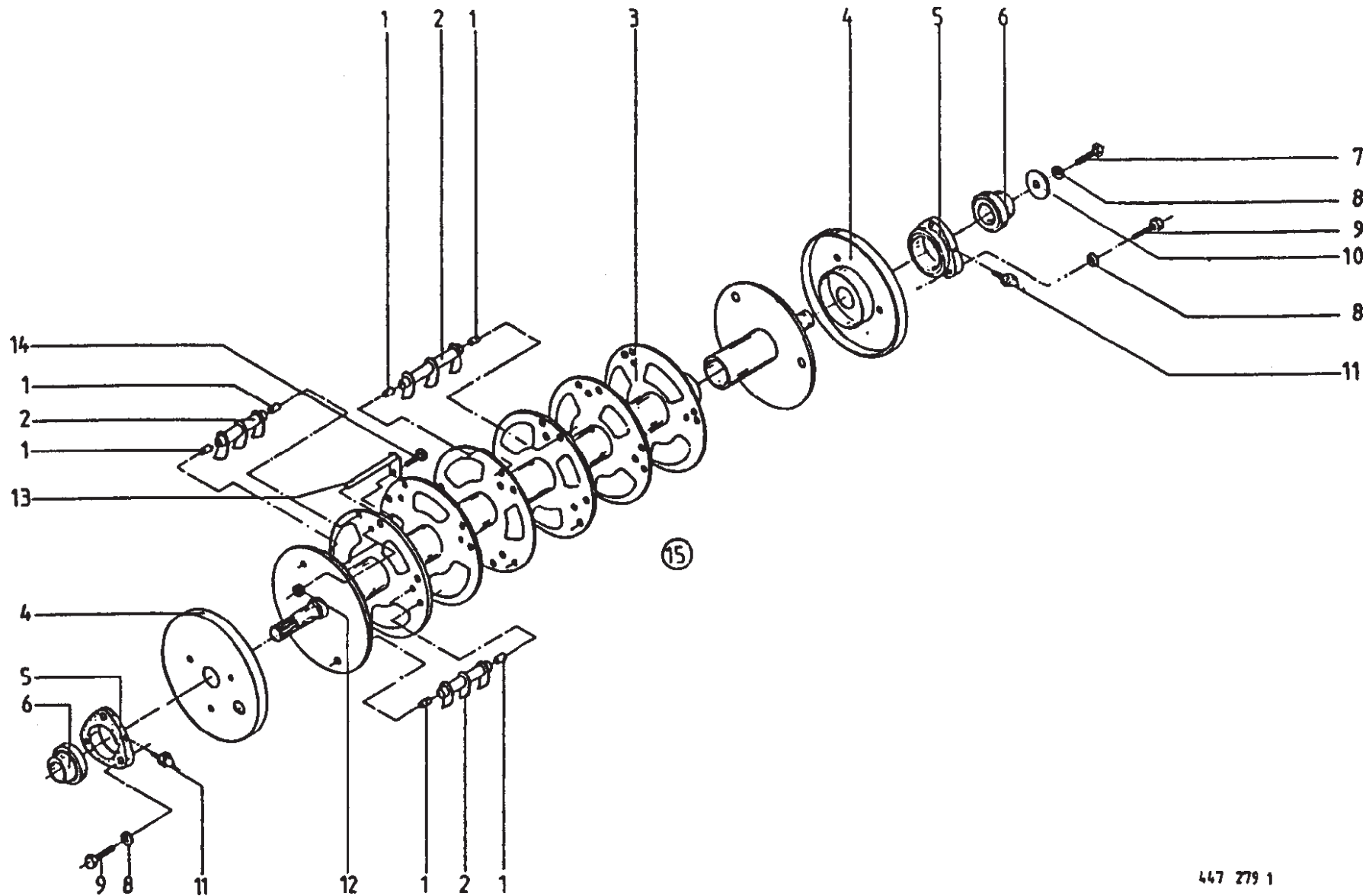
Conditioner Rotor - AM-202Z
