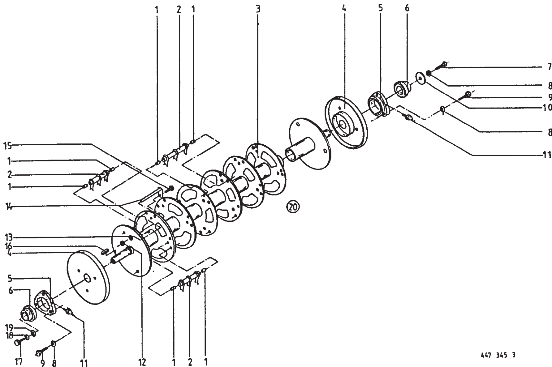
Conditioner Rotor - AM-242Z/282Z
