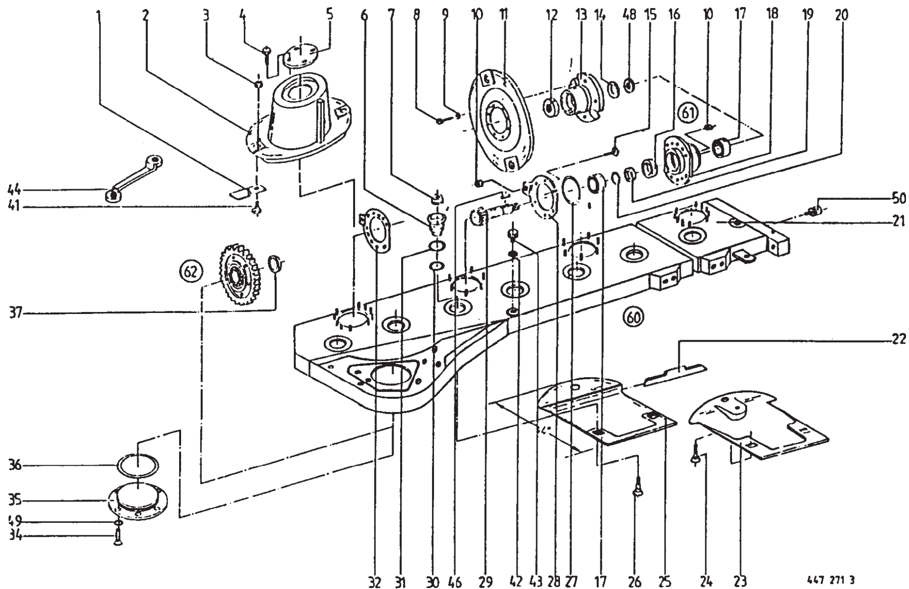
Cutterbar
