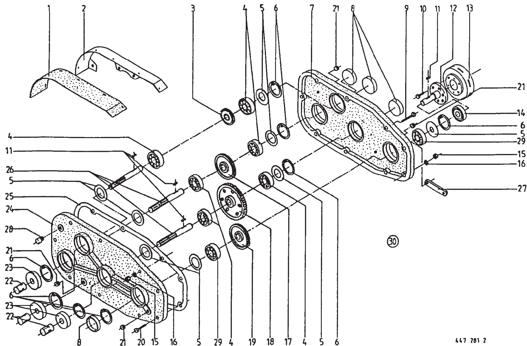
Conditioner Drive Gearbox - AM-202Z
