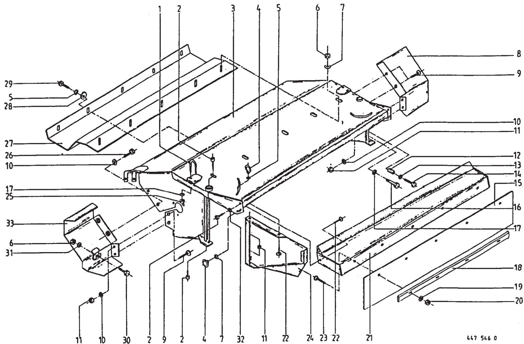
Conditioner Housing - AM-242Z
