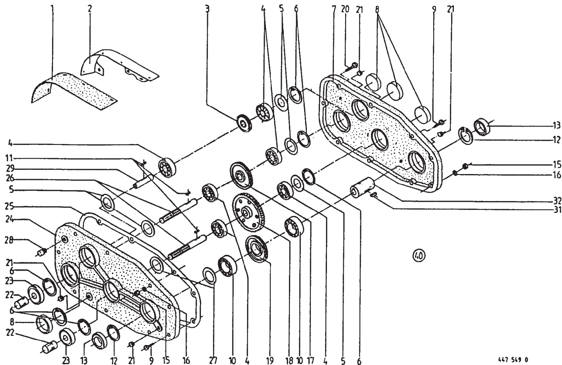
Conditioner Drive Gearbox - AM-242Z/282Z
