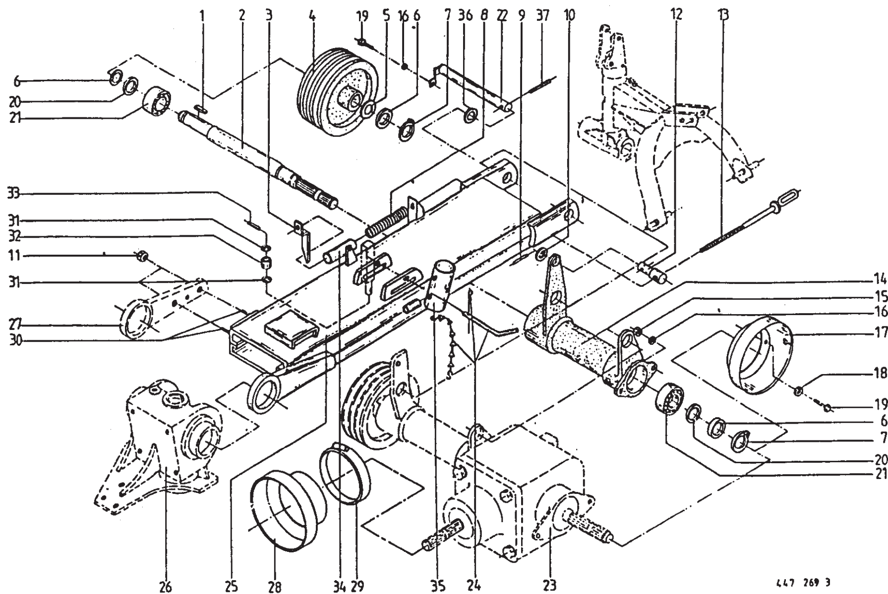
Carrier Beam
