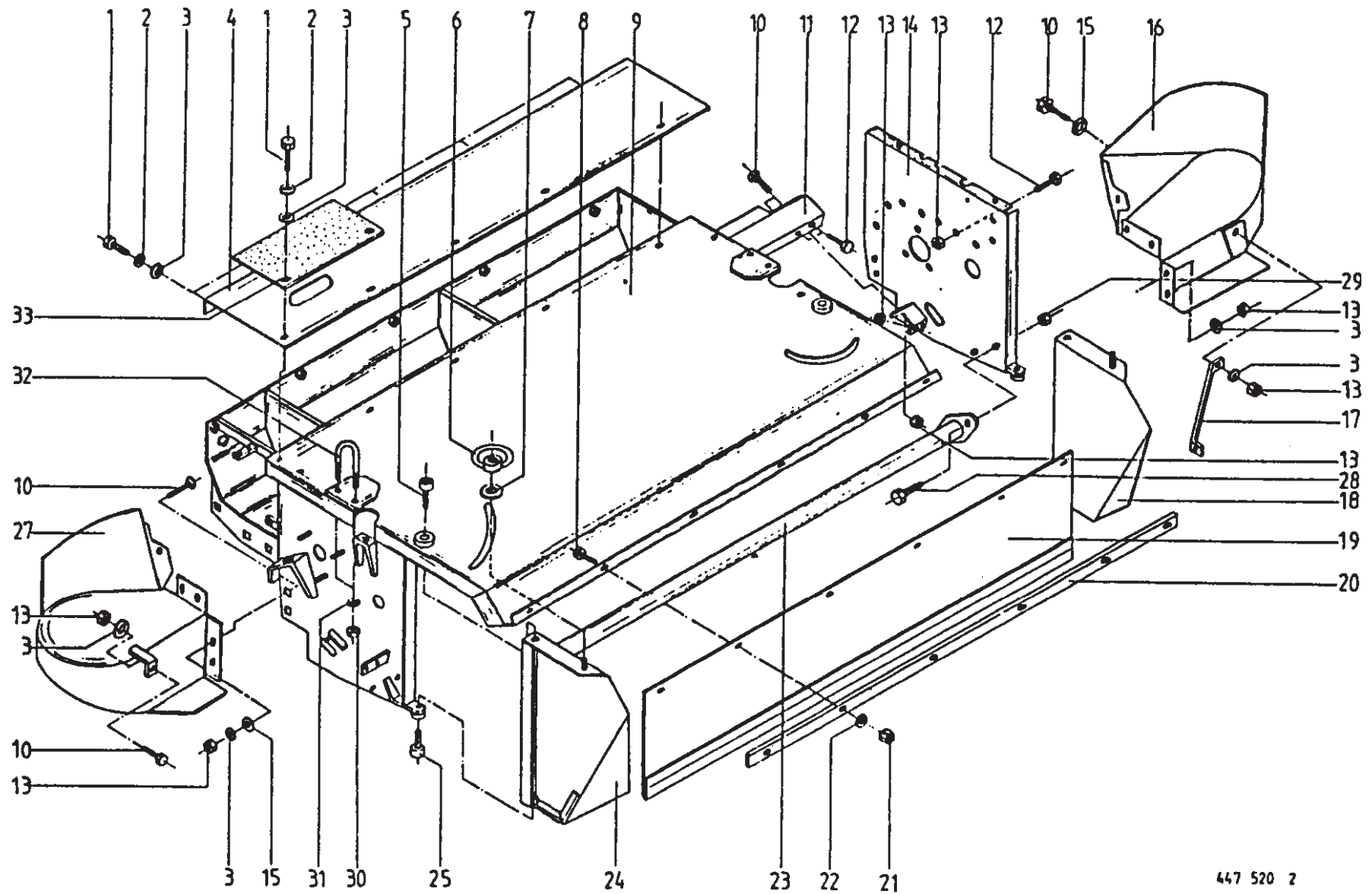
Conditioner Housing
