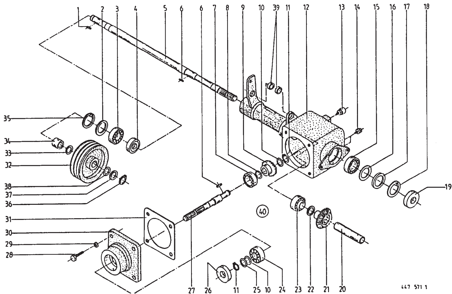
Conditioner Gearbox
