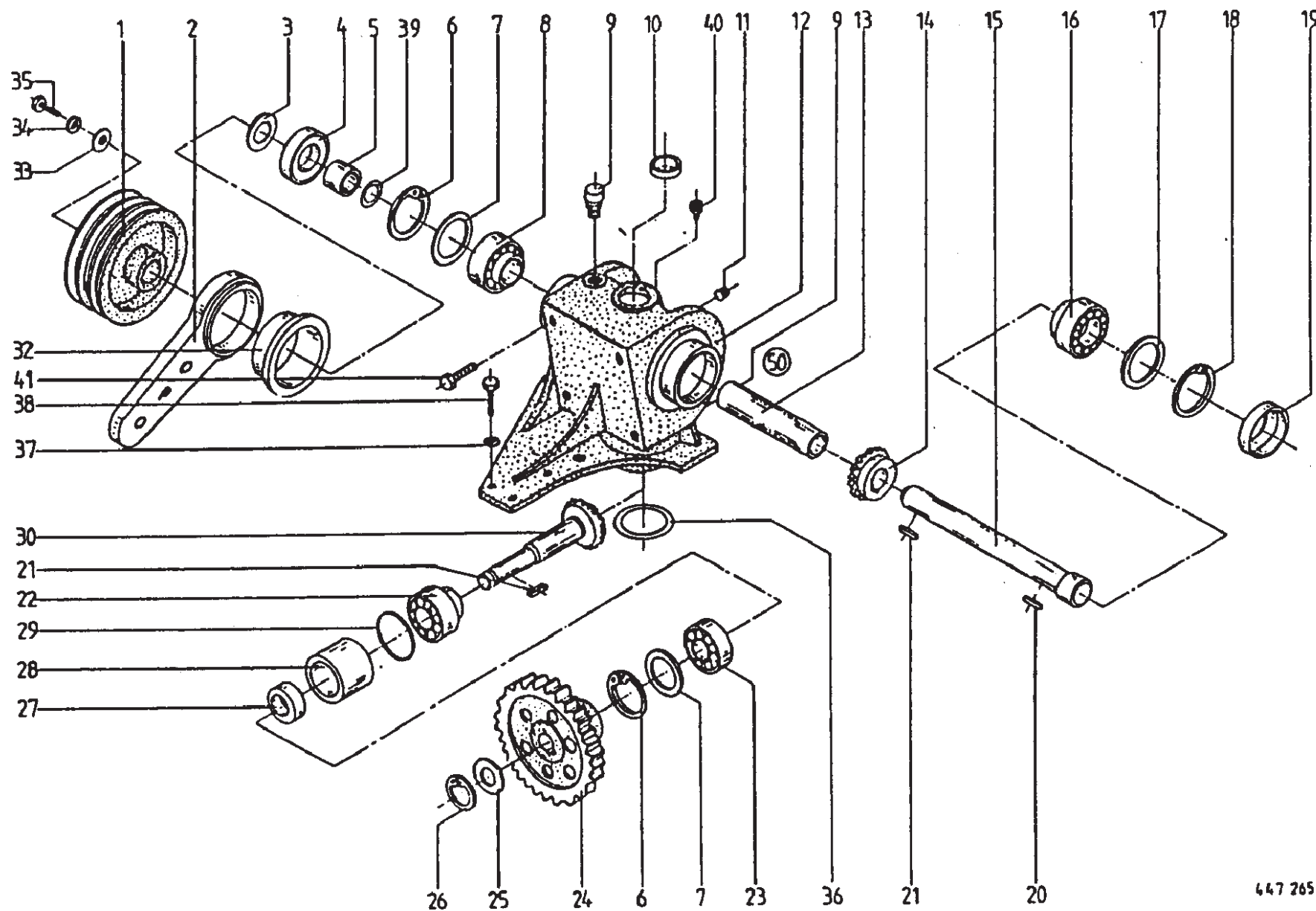
Main Gearbox
